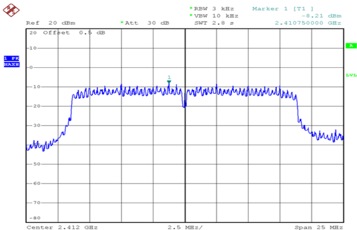
Channel 01 (2412MHz)
