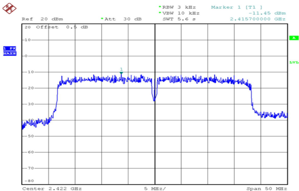
Channel 03 (2422MHz)
