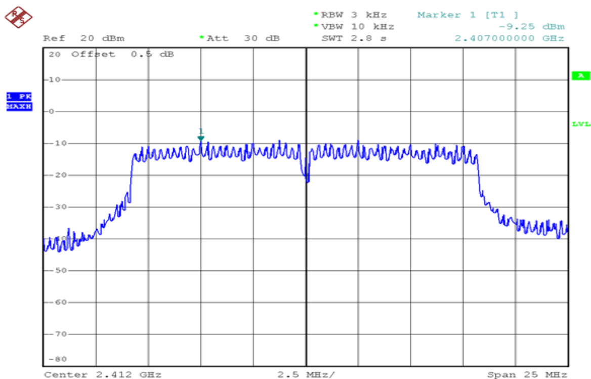
Channel 01 (2412MHz)
