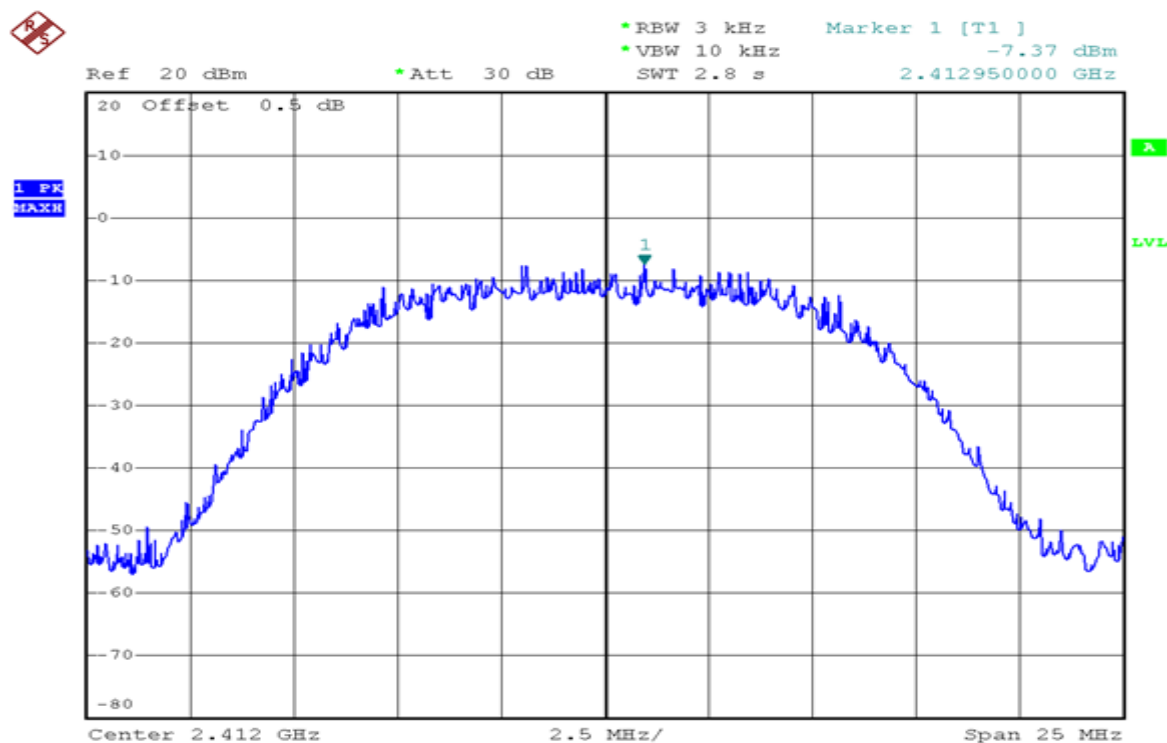
Channel 01 (2412MHz)
