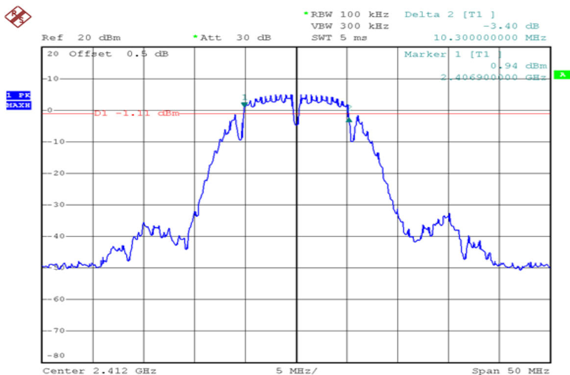
Channel 01 (2412MHz)
