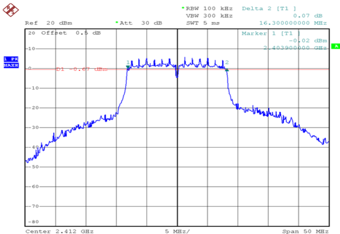
Channel 01 (2412MHz)
