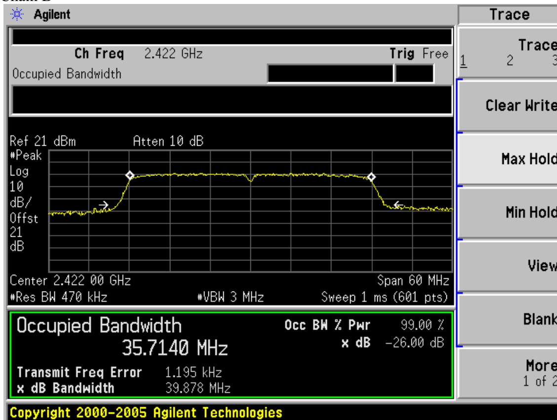
Chain B
