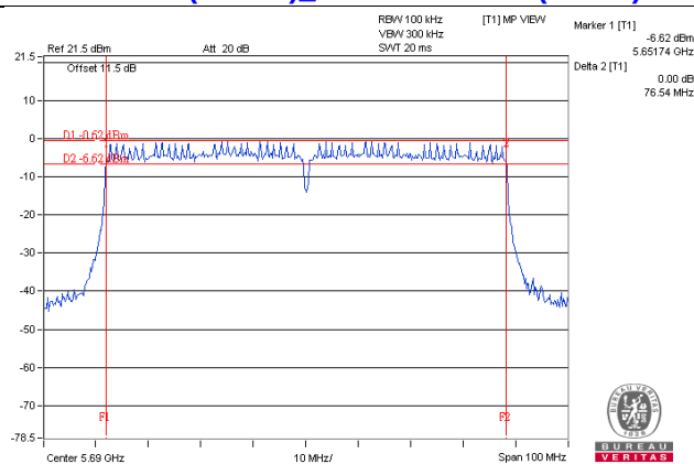
802.11ac (VHT80)_Chain 3 / CH138(UNII-3)
