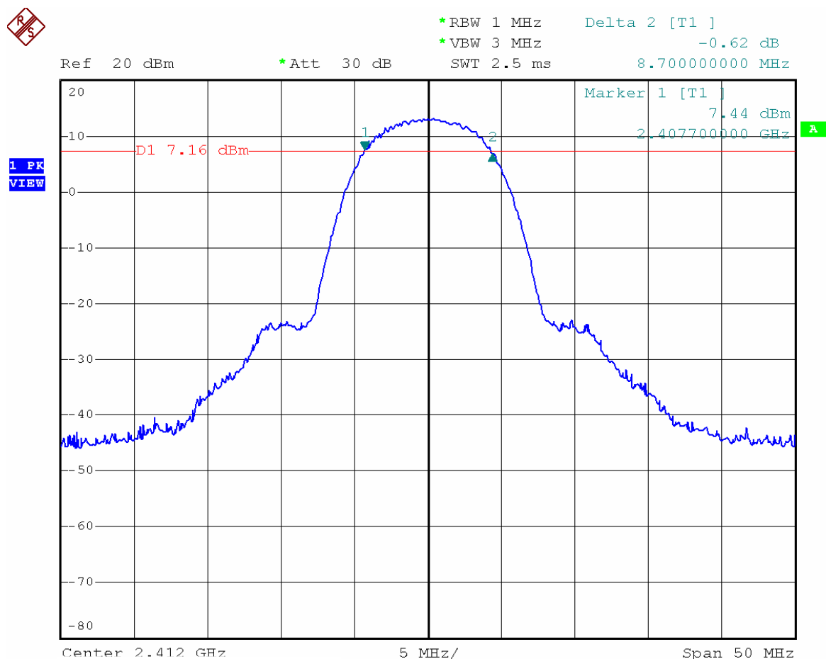
Channel 01 (2412MHz)
