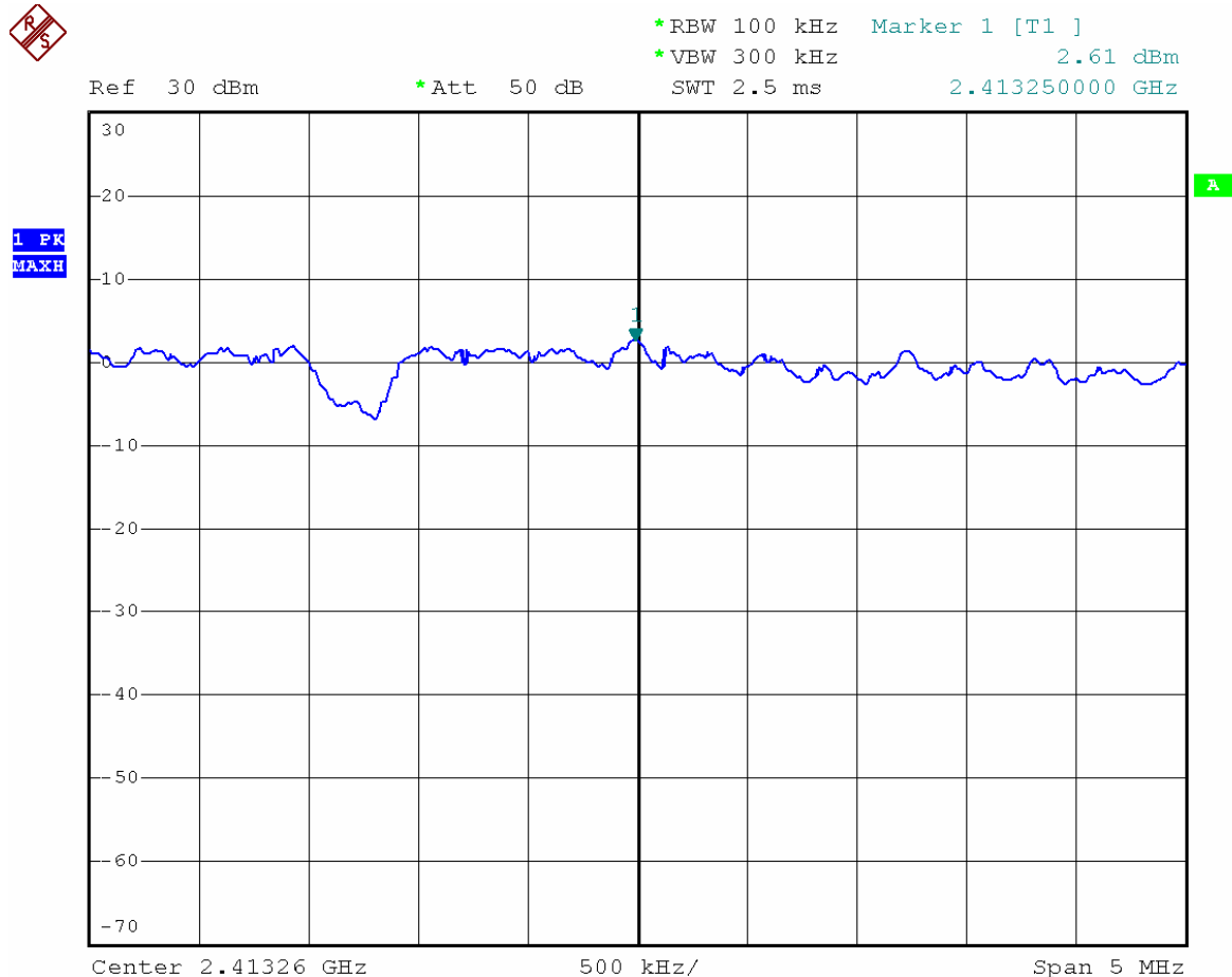
Channel 01 (2412MHz)
