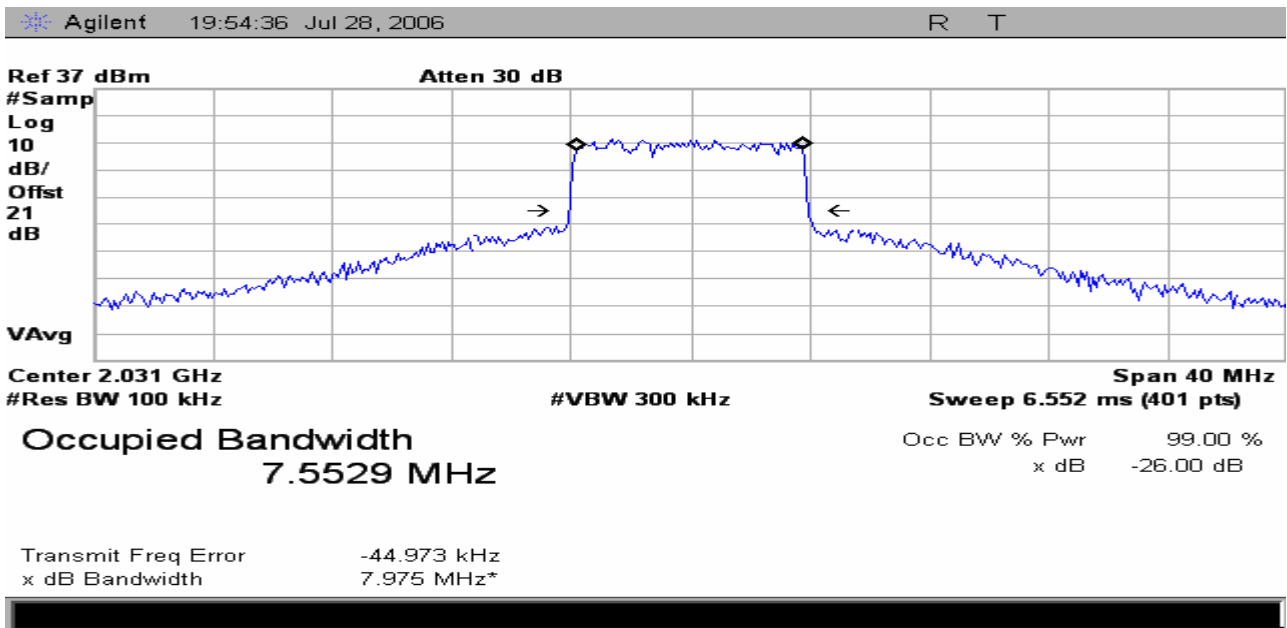
Figure 1 Occupied Bandwidth measurement; Modulation overlaying Mask and measured Power Bandwidth. COFDM modulation, 8 MHz 16QAM color Bars with Audio Channel 1 BAS relo frequency
