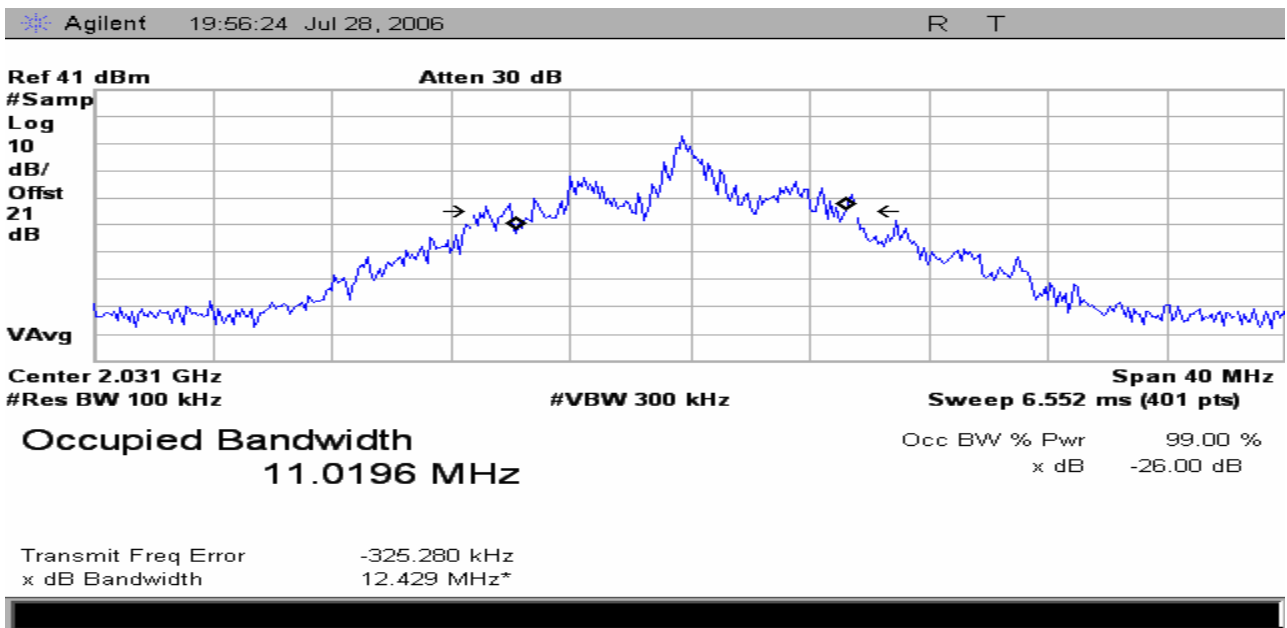
Figure 5 Occupied Bandwidth measurement; Modulation overlaying Mask and measured Power Bandwidth. FM , +/- 3 MHz Deviation ,Color Bars with Audio
