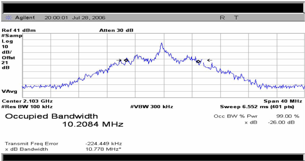
Figure 8 Occupied Bandwidth measurement; Modulation overlaying Mask and measured Power Bandwidth. FM , +/- 3 MHz Deviation ,Color Bars with Audio
