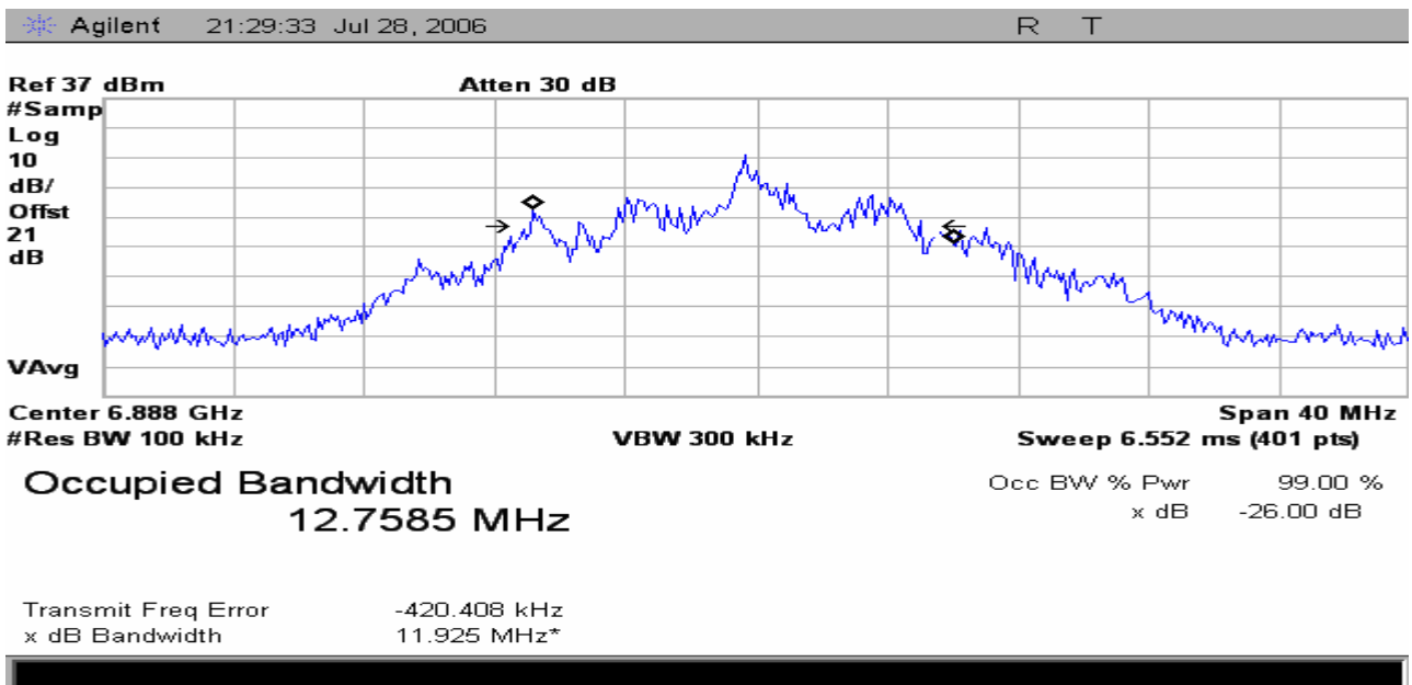
Figure 6 Occupied Bandwidth measurement; Modulation overlaying Mask and measured Power Bandwidth. FM , +/- 3 MHz Deviation ,Color Bars with Audio
