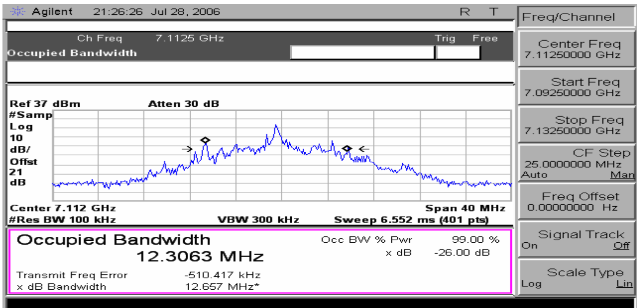
Figure 9 Occupied Bandwidth measurement; Modulation overlaying Mask and measured Power Bandwidth. FM , +/- 3 MHz Deviation ,Color Bars with Audio
