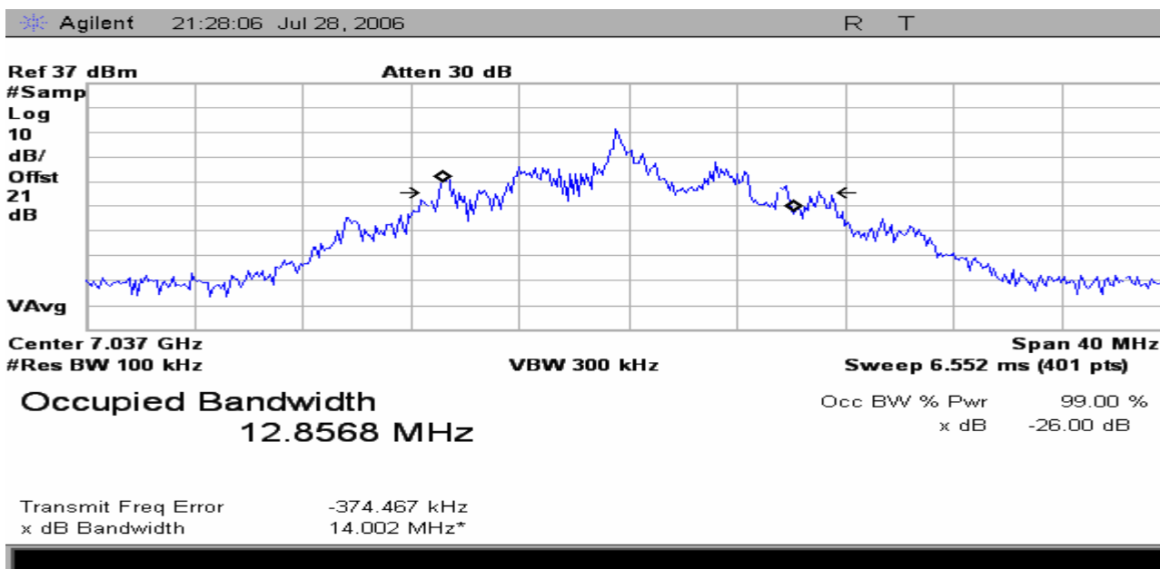
Figure 8 Occupied Bandwidth measurement; Modulation overlaying Mask and measured Power Bandwidth. FM , +/- 3 MHz Deviation ,Color Bars with Audio
