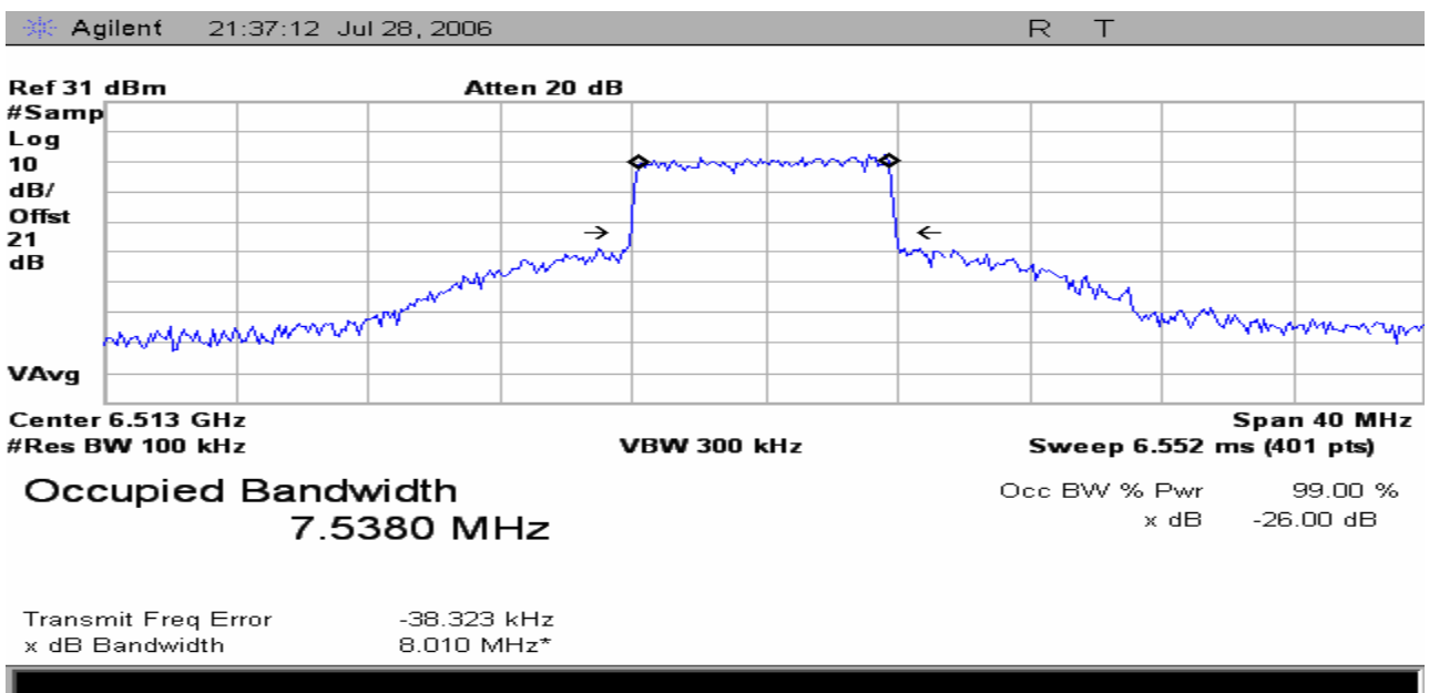
Figure 5 Occupied Bandwidth measurement; Modulation overlaying Mask and measured Power Bandwidth. COFDM modulation, 8 MHz 16QAM, Color Bars with Audio
