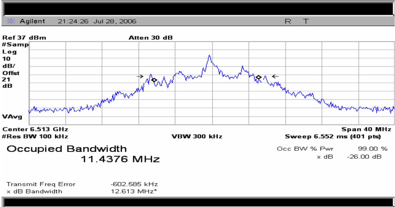
Figure 10 Occupied Bandwidth measurement; Modulation overlaying Mask and measured Power Bandwidth. FM , +/- 3 MHz Deviation ,Color Bars with Audio
