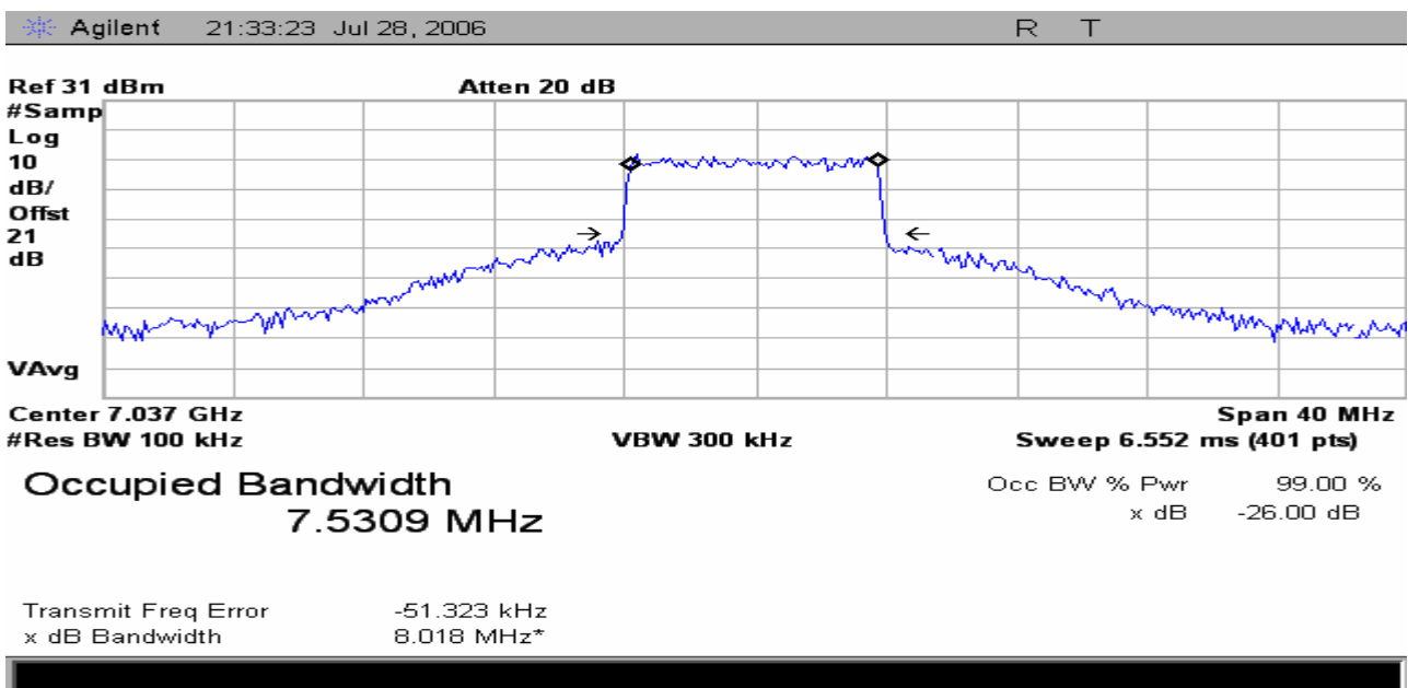
Figure 3 Occupied Bandwidth measurement; Modulation overlaying Mask and measured Power Bandwidth. COFDM modulation, 8 MHz 16QAM, Color Bars with Audio Channel 7 , 7 GHz Band 25 MHz Channels
