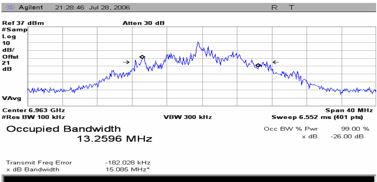
Figure 7 Occupied Bandwidth measurement; Modulation overlaying Mask and measured Power Bandwidth. FM , +/- 3 MHz Deviation ,Color Bars with Audio
