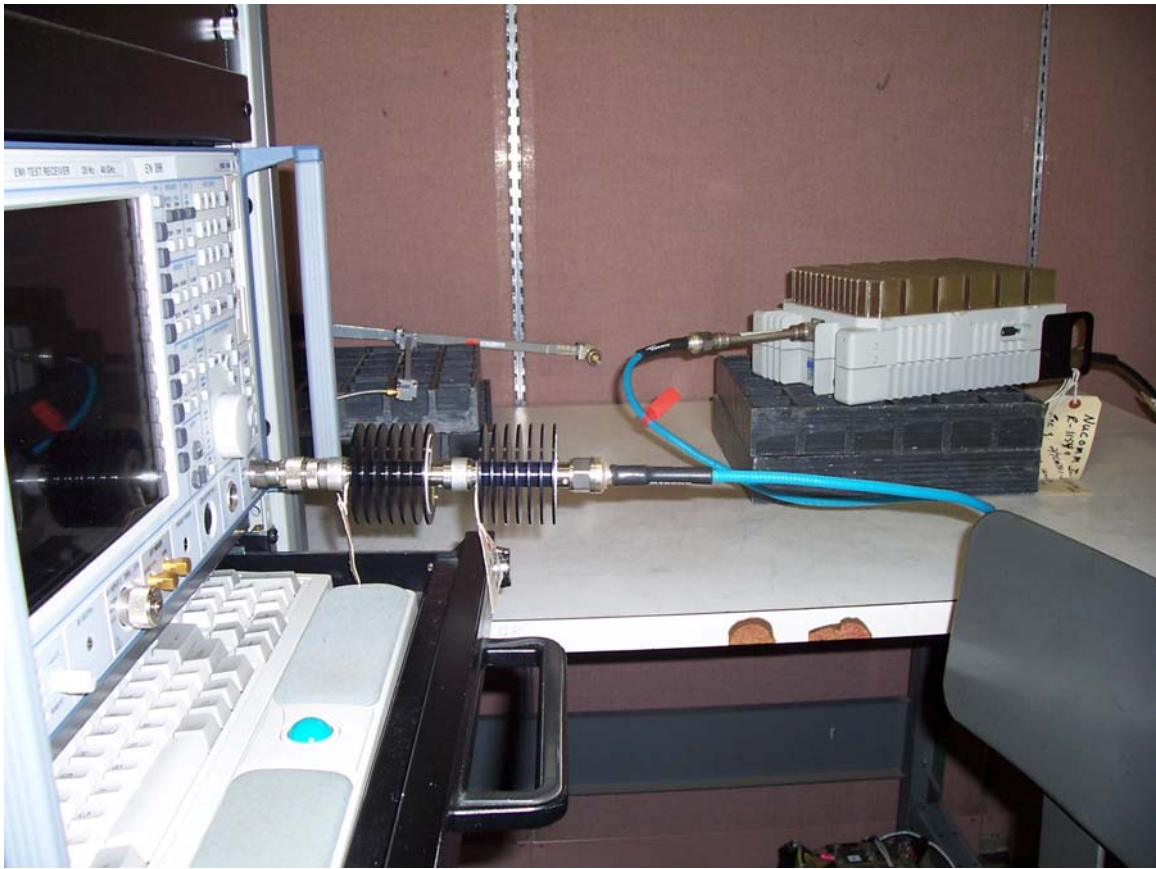
High Power Unit Antenna Conducted Emissions 30 MHz to 18 GHz
