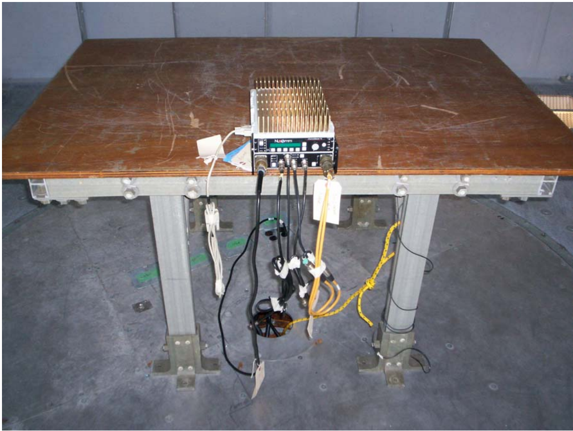
low Power Unit Spurious Emissions Setup Back
