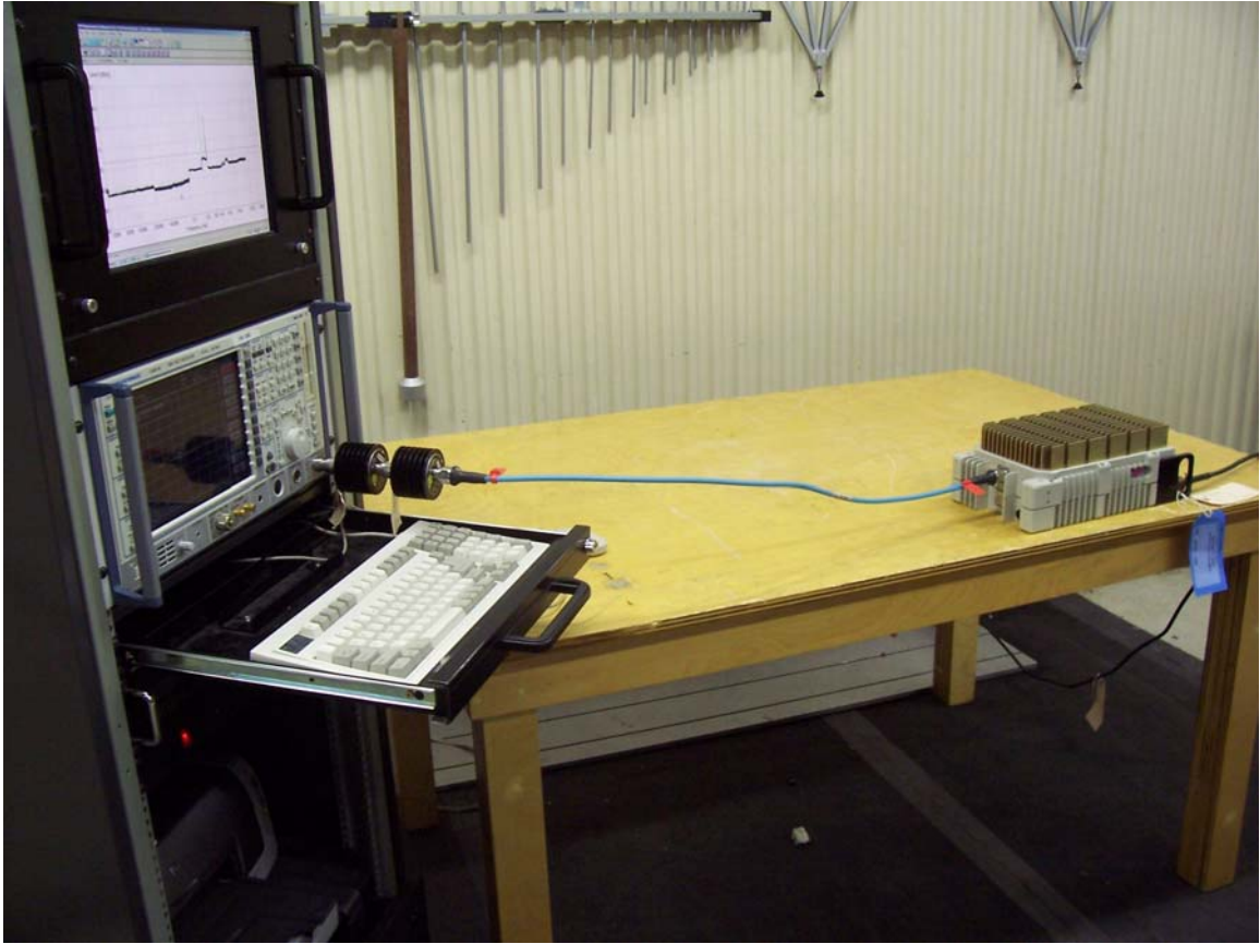
low Power Unit Antenna Conducted Emissions 30 MHz to 18 GHz
