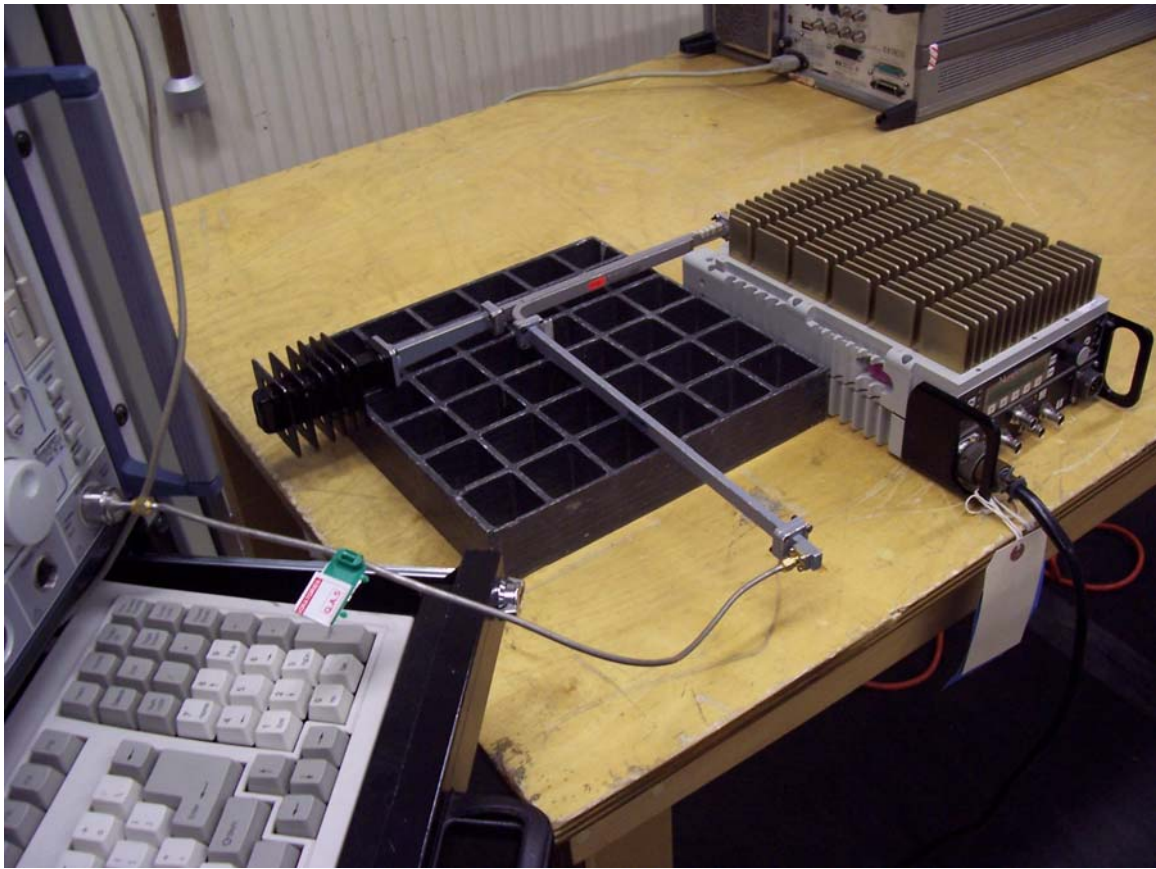
low Power Unit Antenna Conducted Emissions 18 GHz to 40 GHz
