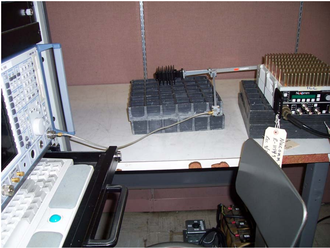
High Power Unit Antenna Conducted Emissions 18 GHz to 40 GHz
