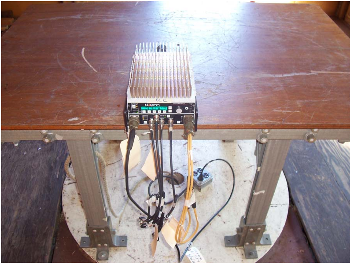
High Power Unit Spurious Emissions Setup Back
