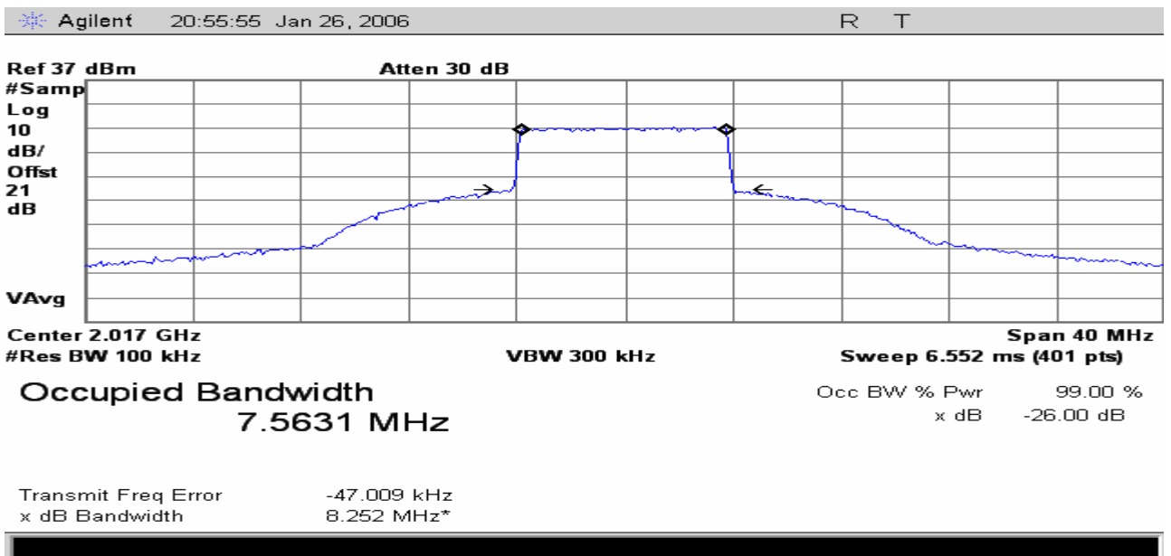
Figure 14 Occupied Bandwidth measurement; Modulation overlaying Mask and measured Power Bandwidth. COFDM modulation, 8 MHz 16QAM, Color Bars with Audio
