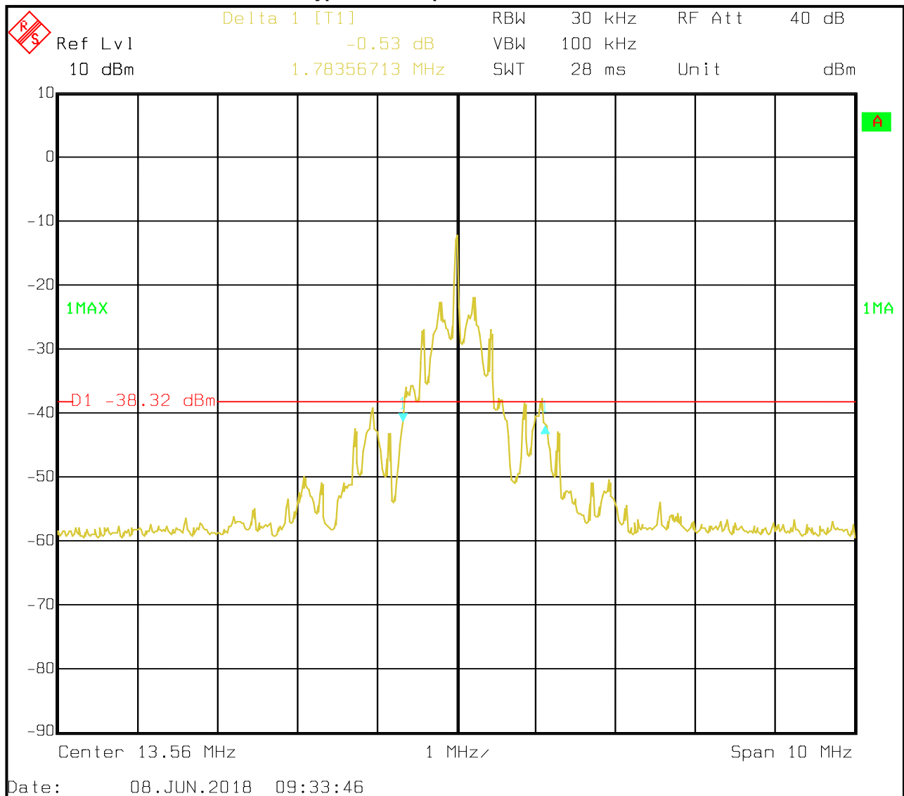
Plot 5-2: 99% Bandwidth – Type A 212 Kbps
