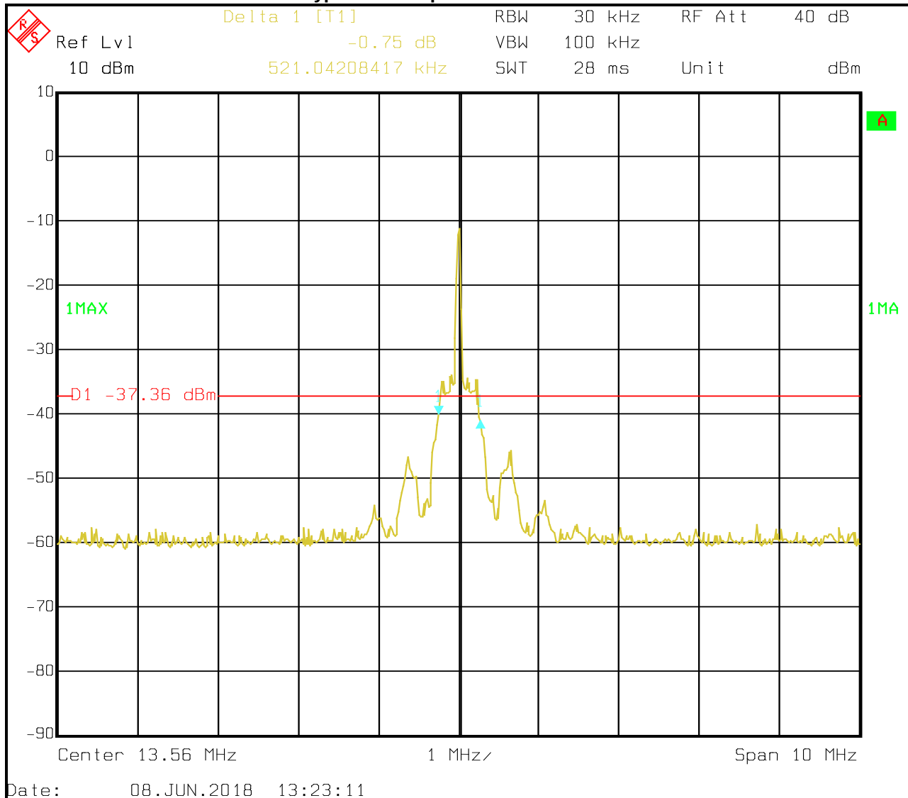
Plot 5-7: 99% Bandwidth – Type F 212 Kbps
