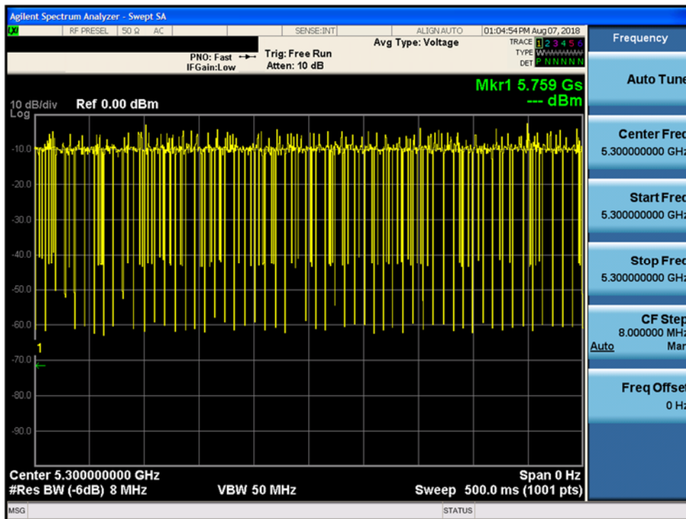
Figure 5-2. Traffic Plot
