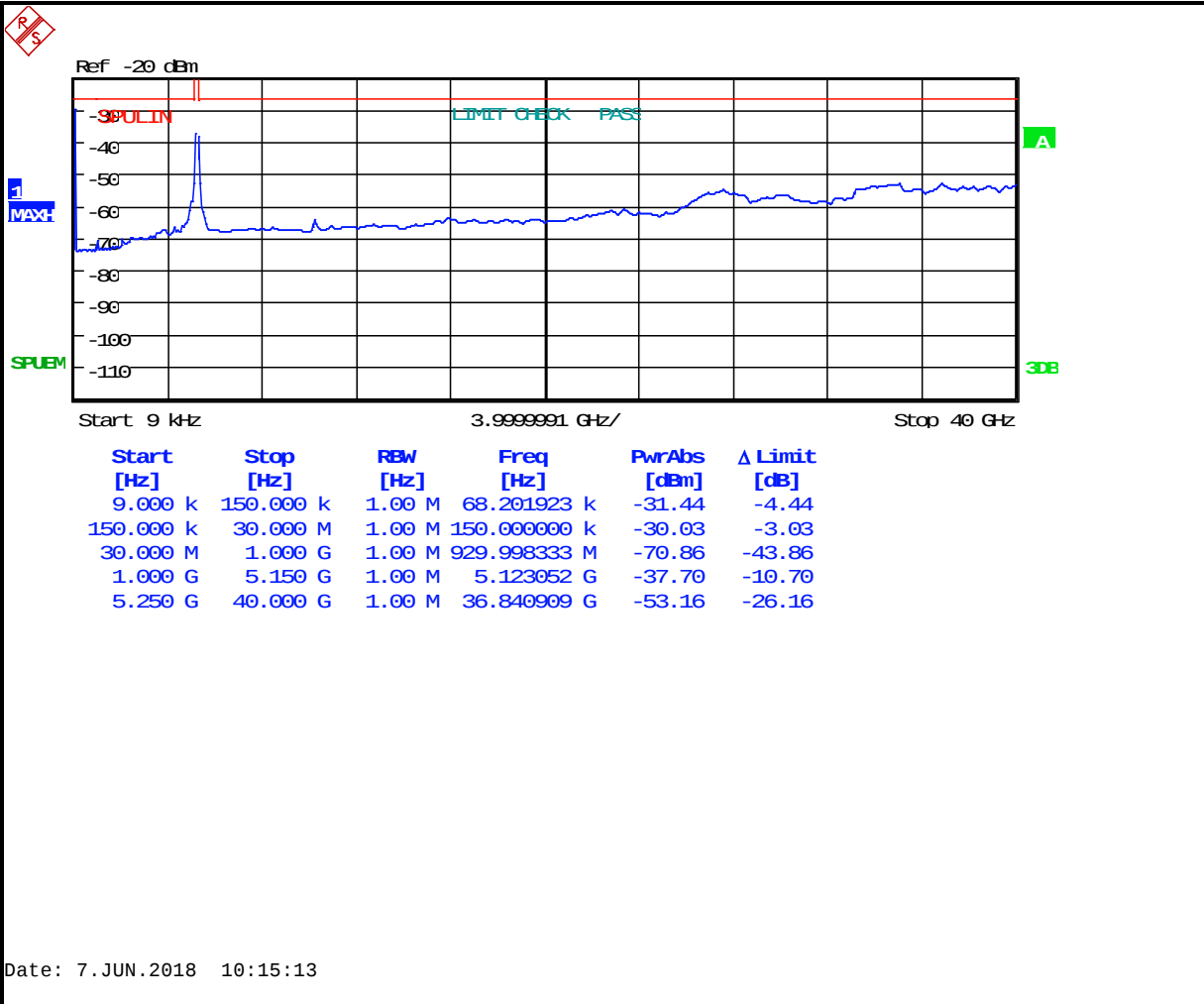
Plot 5-6: Antenna Conducted Spurious Emissions – 5200 MHz 802.11n 40 MHz BW
