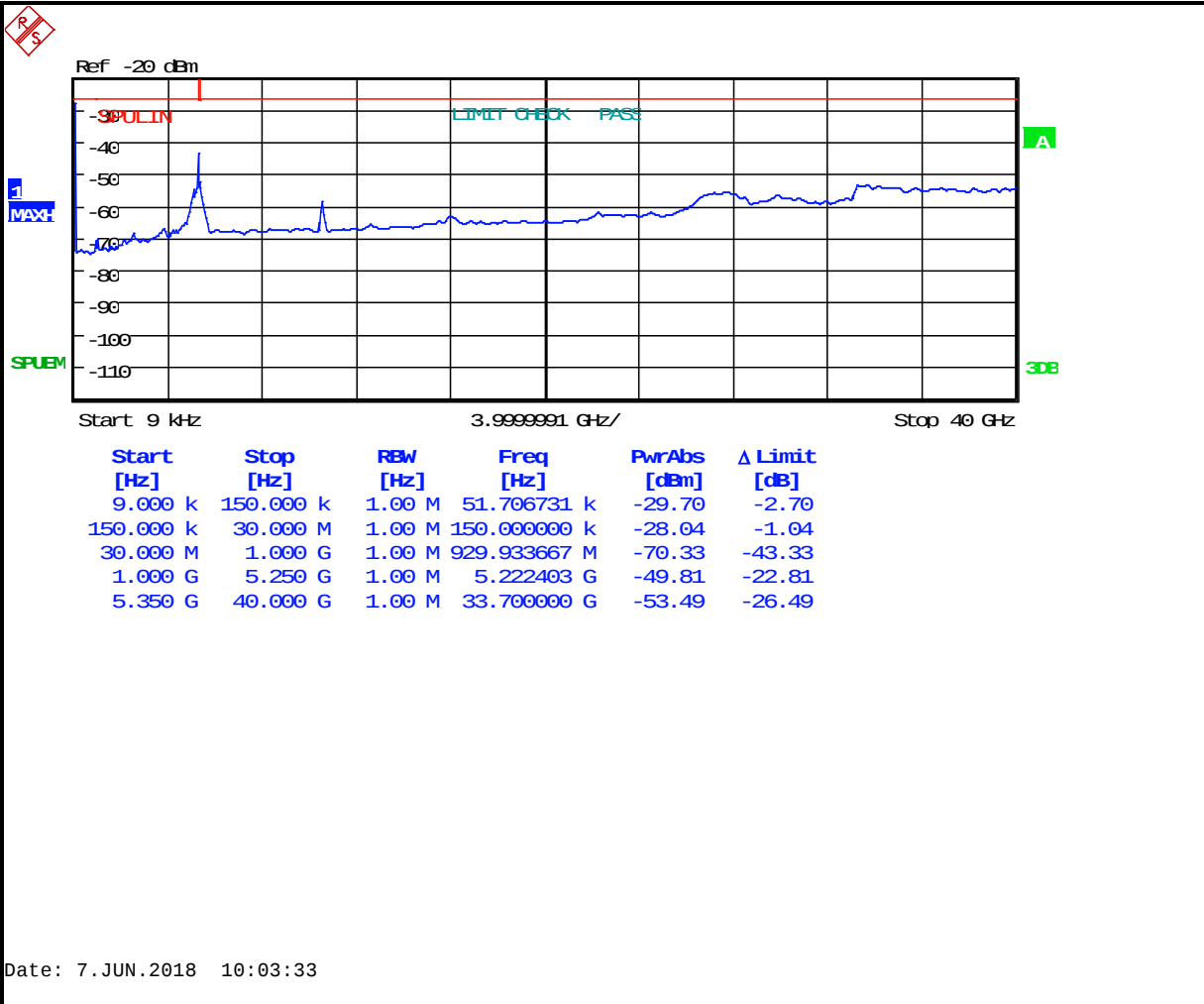
Plot 5-17: Antenna Conducted Spurious Emissions – 5280 MHz 802.11a 20 MHz BW
