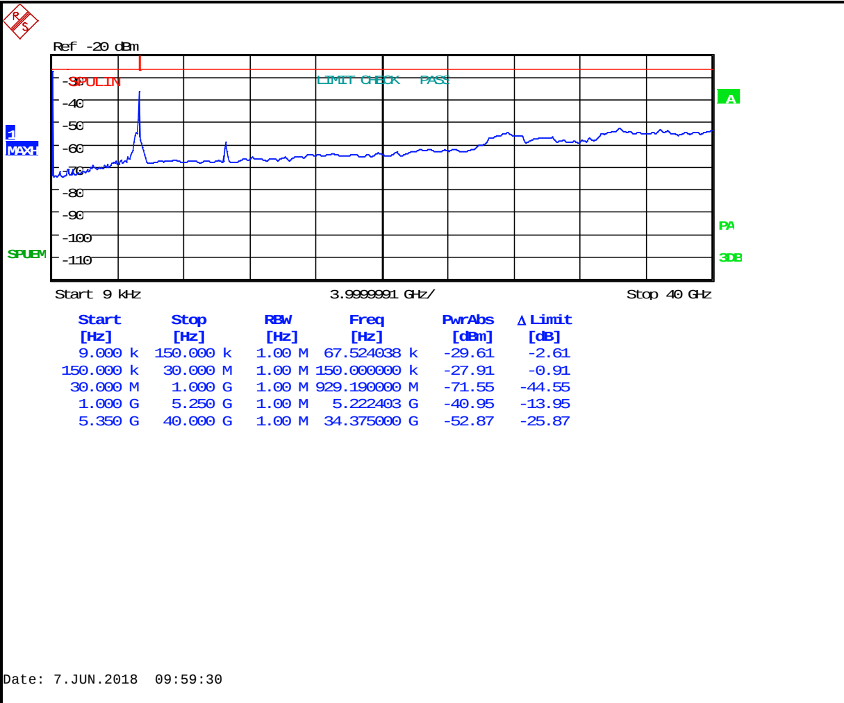
Plot 5-14: Antenna Conducted Spurious Emissions – 5260 MHz 802.11a 20 MHz BW
