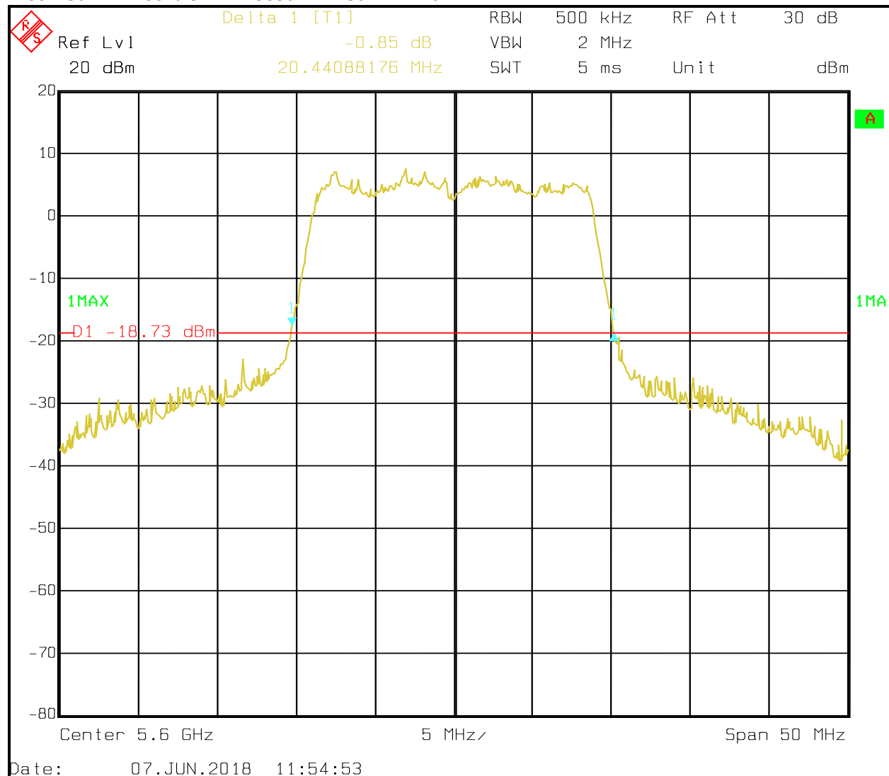
Plot 7-30: 99% OBW – 5650 MHz 802.11n 20 MHz BW
