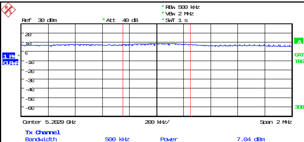
Plot 8-4: PSD – 5200 MHz 802.11a 20 MHz
