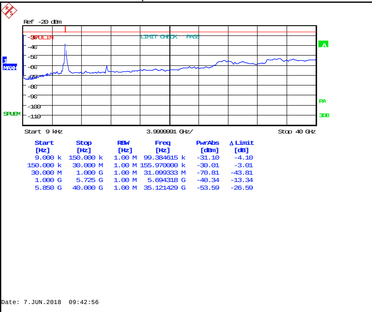
Plot 5-38: Antenna Conducted Spurious Emissions – 5745 MHz 802.11n 40 MHz BW
