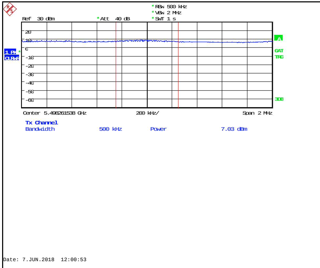
Plot 8-25: PSD – 5500 MHz 802.11n 20 MHz
