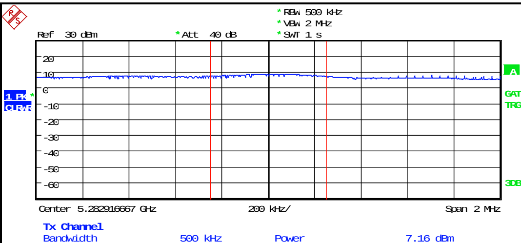
Plot 8-17: PSD – 5280 MHz 802.11a 20 MHz
