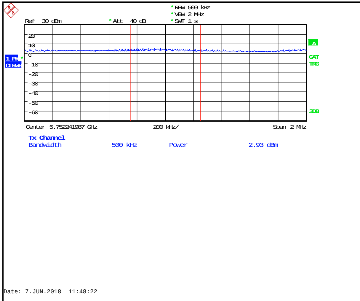
Plot 8-38: PSD – 5745 MHz 802.11n 40 MHz
