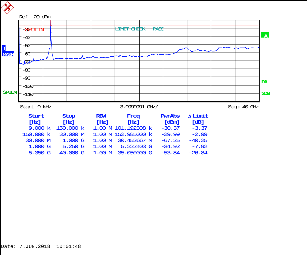
Plot 5-16: Antenna Conducted Spurious Emissions – 5260 MHz 802.11n 40 MHz BW
