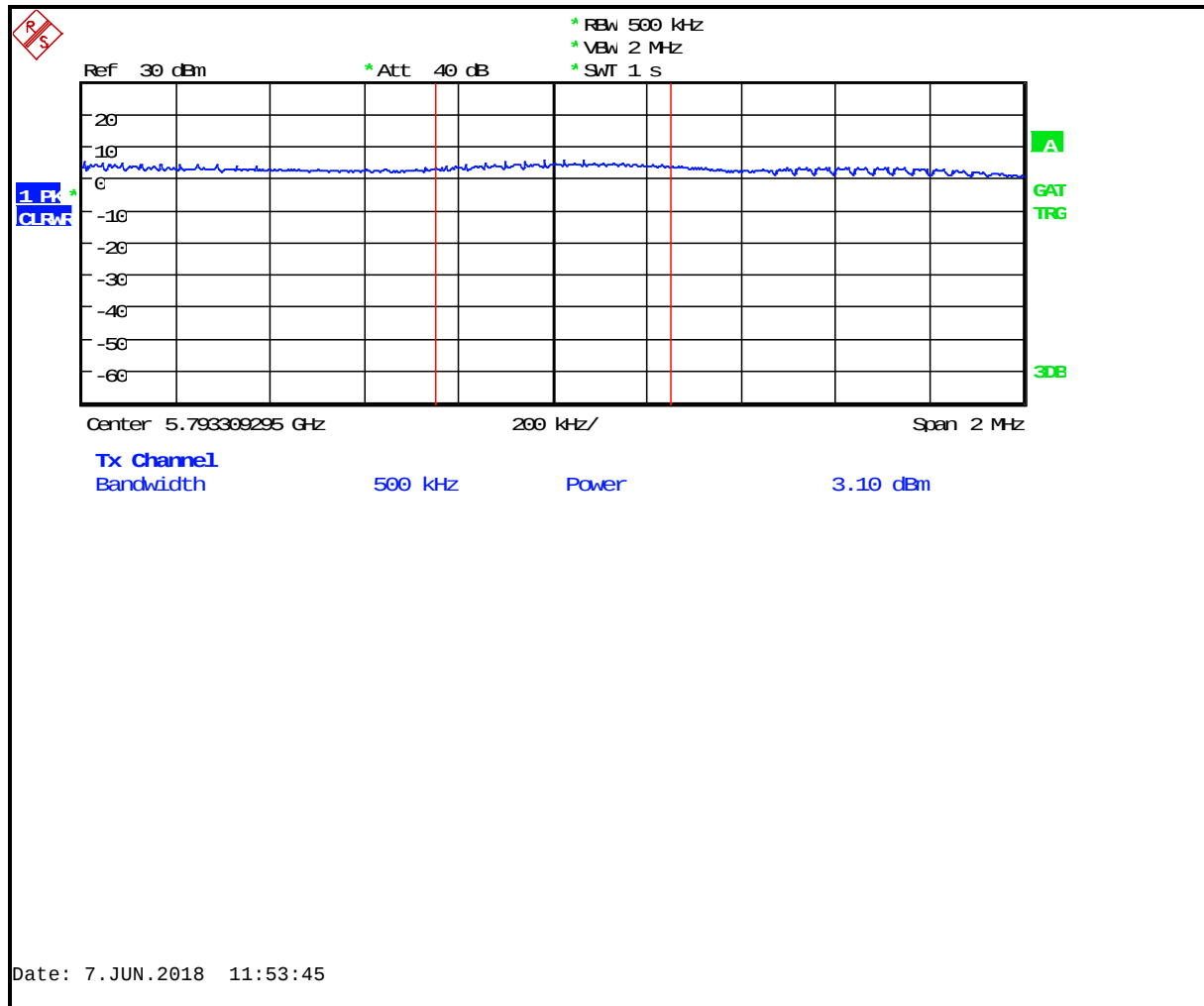
Plot 8-41: PSD – 5785 MHz 802.11n 40 MHz
