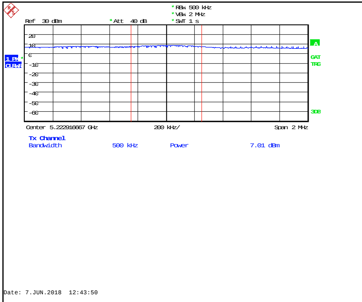
Plot 8-7: PSD – 5220 MHz 802.11a 20 MHz
