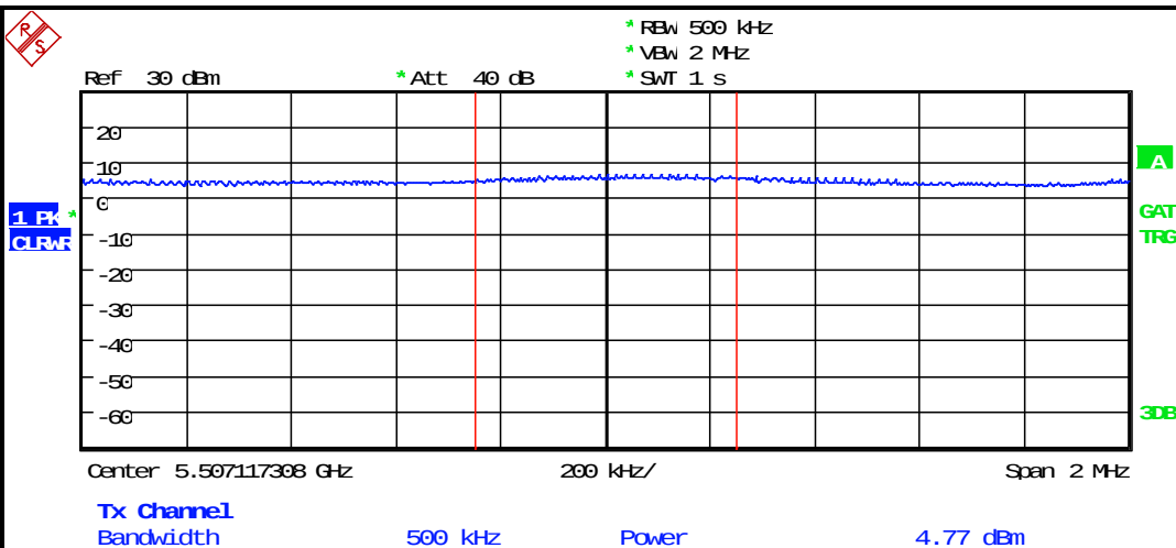
Plot 8-26: PSD – 5500 MHz 802.11n 40 MHz
