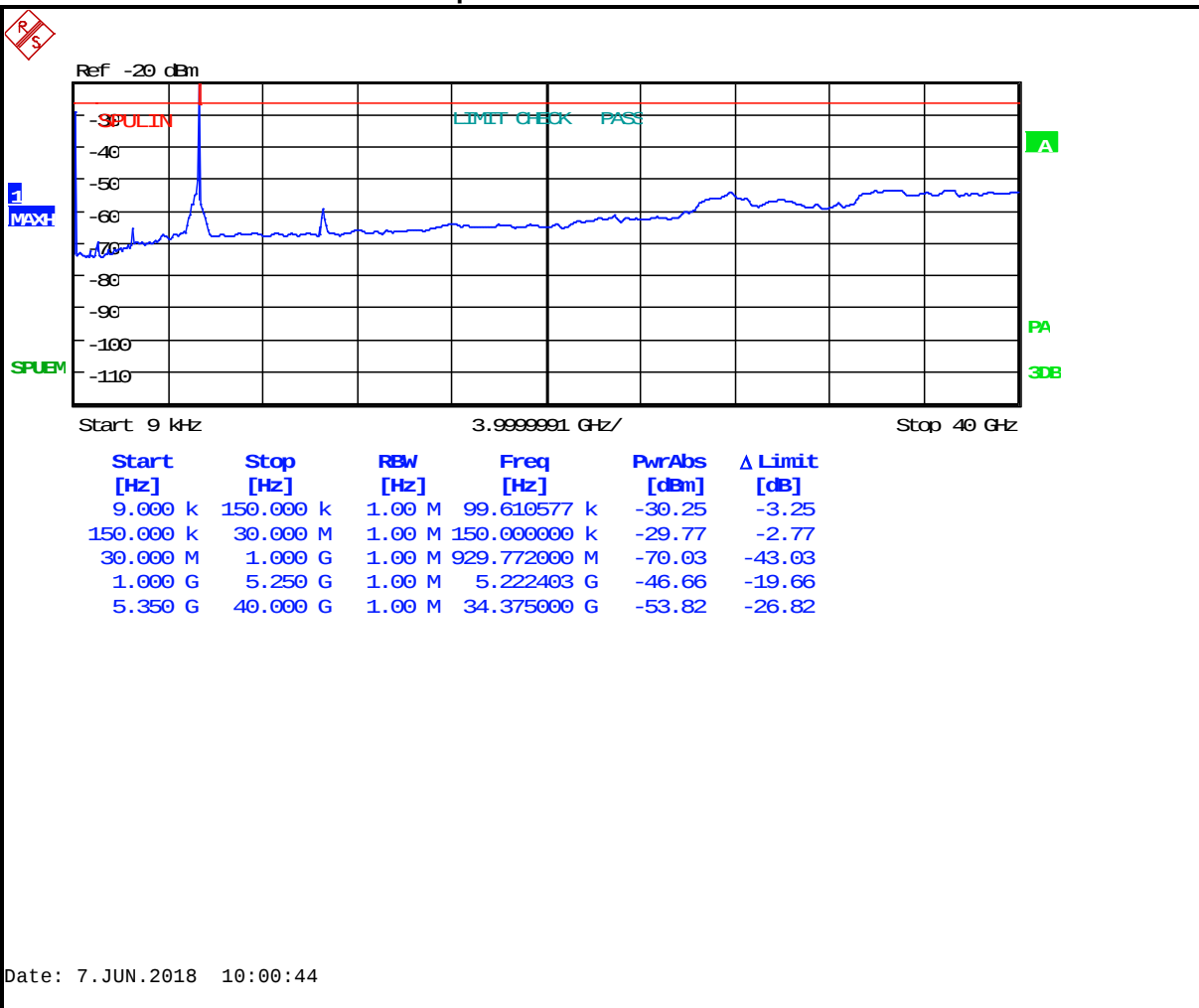
Plot 5-15: Antenna Conducted Spurious Emissions – 5260 MHz 802.11n 20 MHz BW
