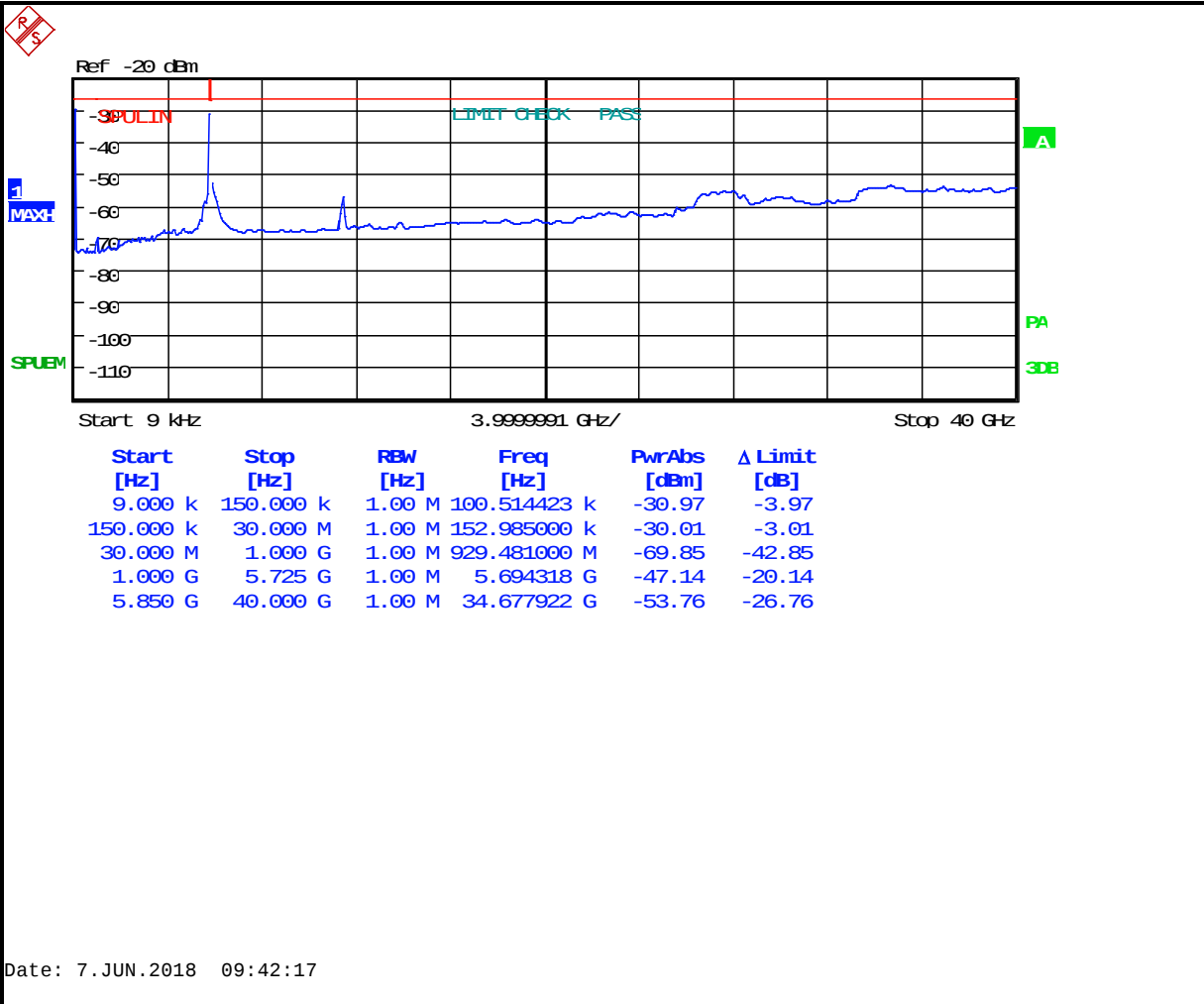
Plot 5-37: Antenna Conducted Spurious Emissions – 5745 MHz 802.11n 20 MHz BW
