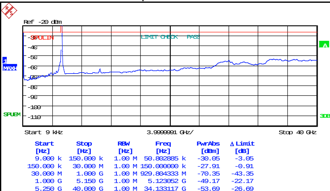
Plot 5-9: Antenna Conducted Spurious Emissions – 5220 MHz 802.11n 40 MHz BW
