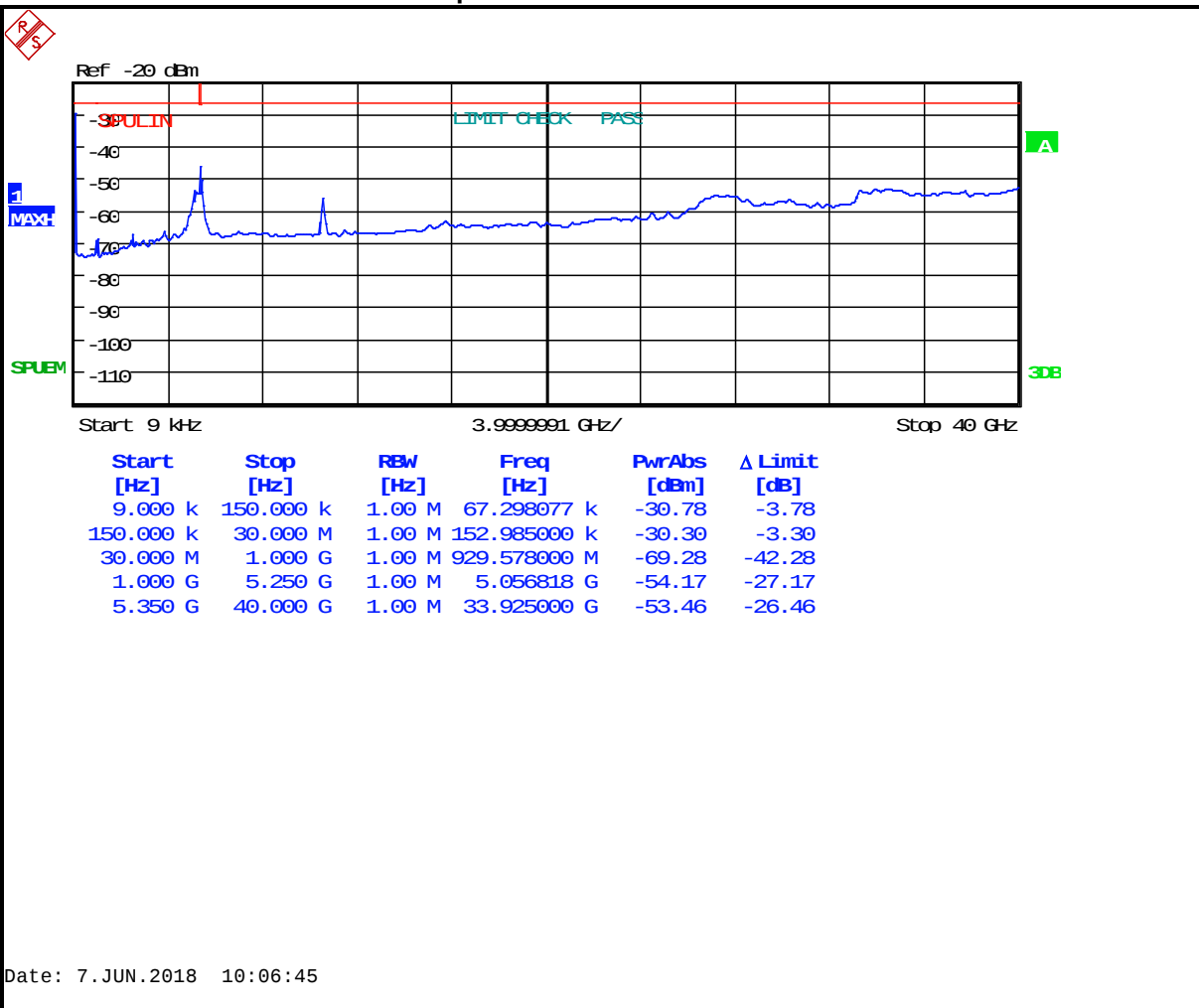
Plot 5-20: Antenna Conducted Spurious Emissions – 5320 MHz 802.11a 20 MHz BW
