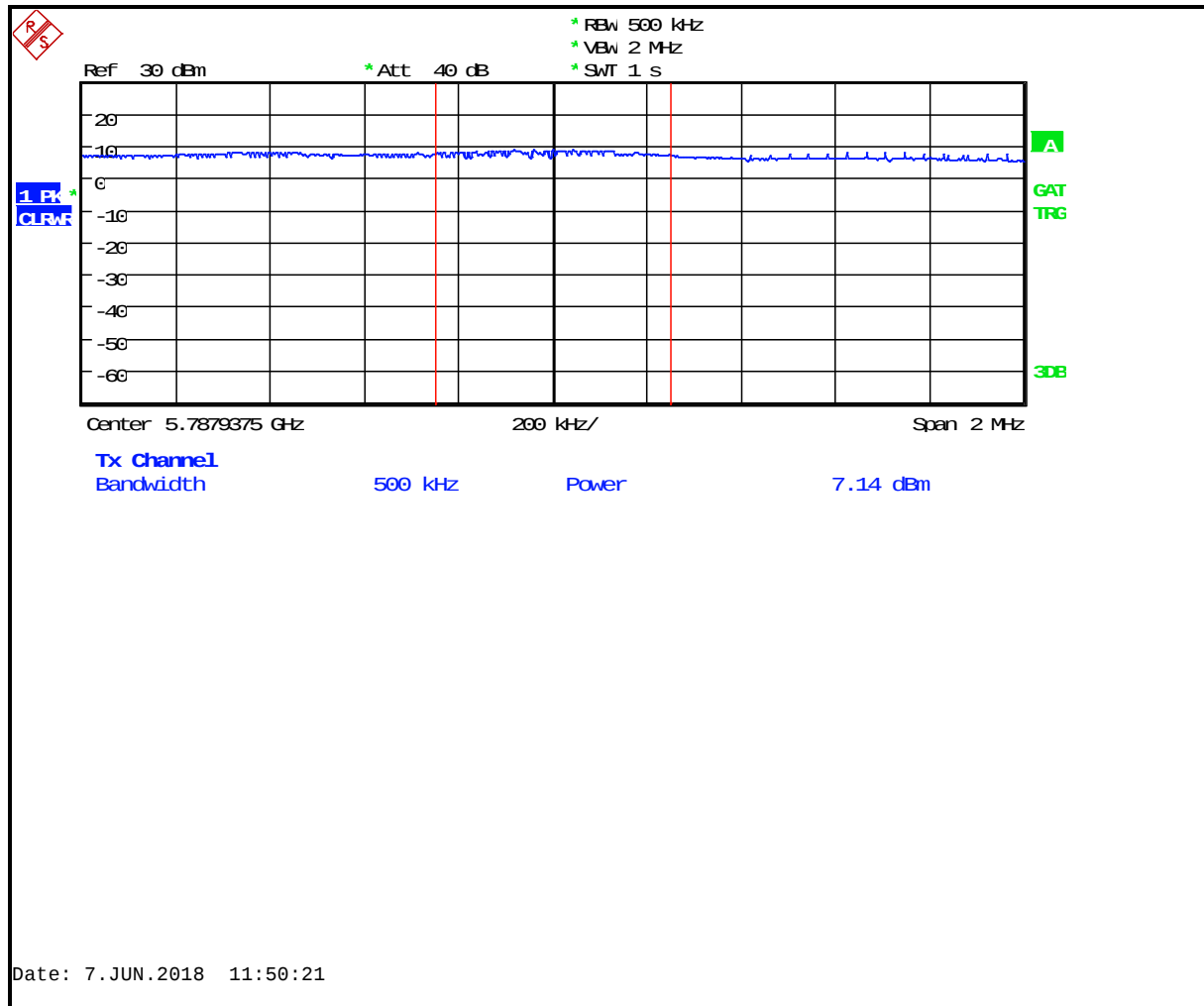
Plot 8-39: PSD – 5785 MHz 802.11a 20 MHz
