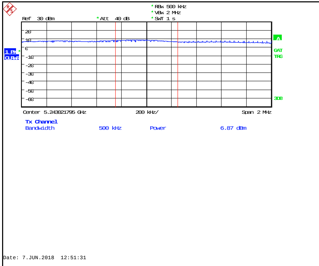
Plot 8-10: PSD – 5240 MHz 802.11a 20 MHz
