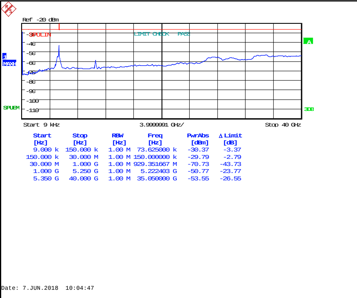
Plot 5-18: Antenna Conducted Spurious Emissions – 5280 MHz 802.11n 20 MHz BW
