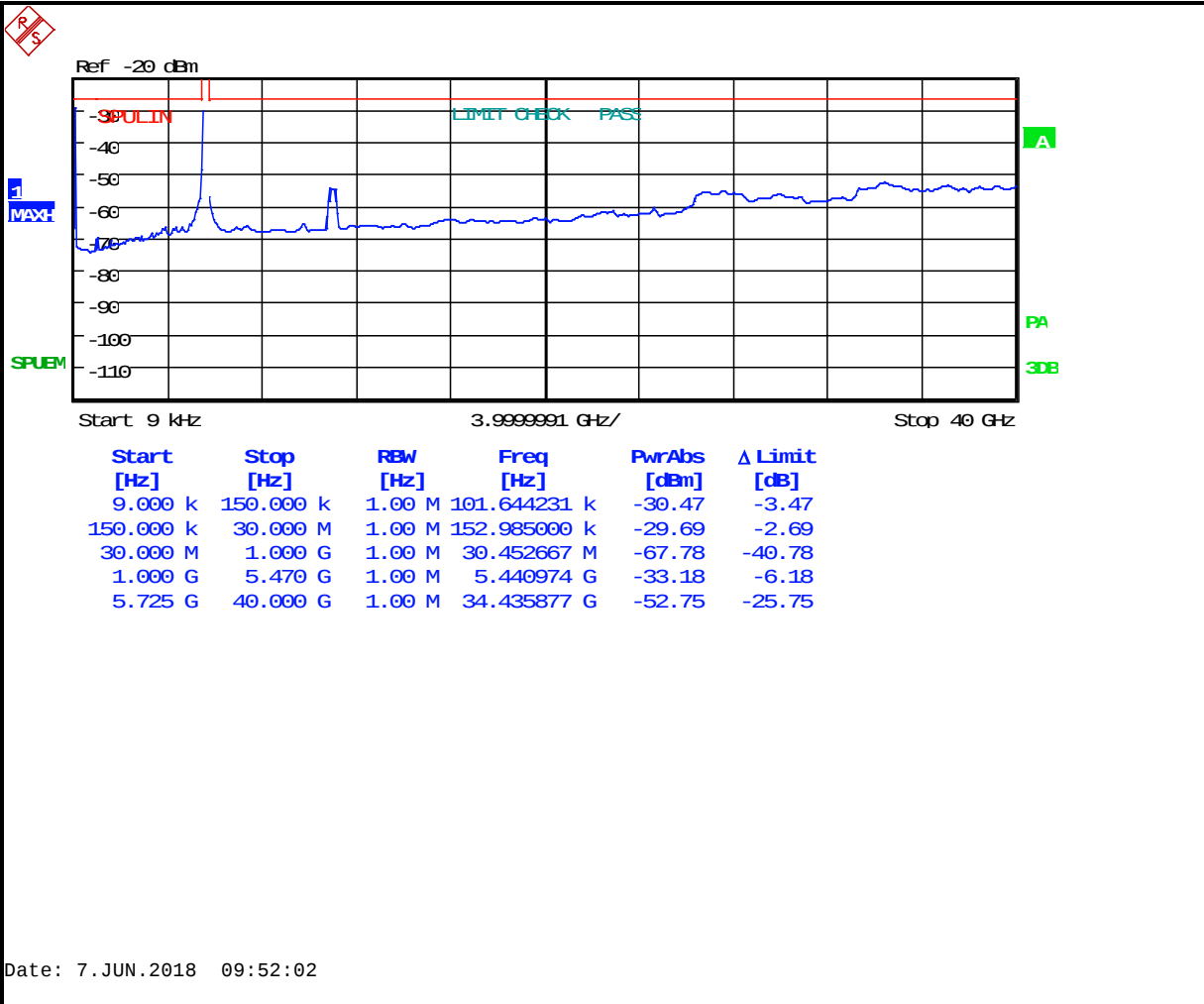
Plot 5-26: Antenna Conducted Spurious Emissions – 5500 MHz 802.11n 40 MHz BW
