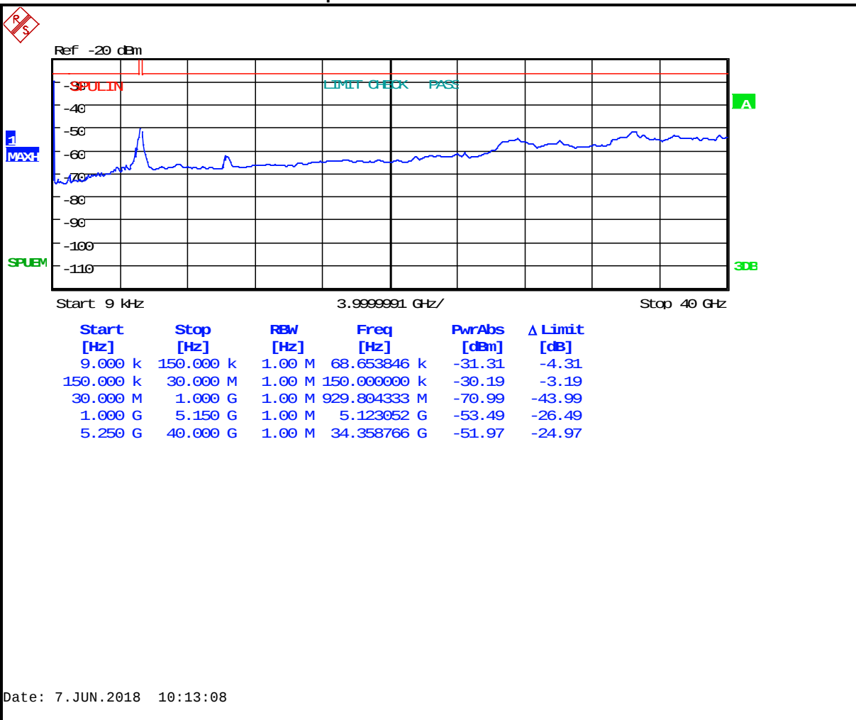
Plot 5-4: Antenna Conducted Spurious Emissions – 5200 MHz 802.11a 20 MHz BW
