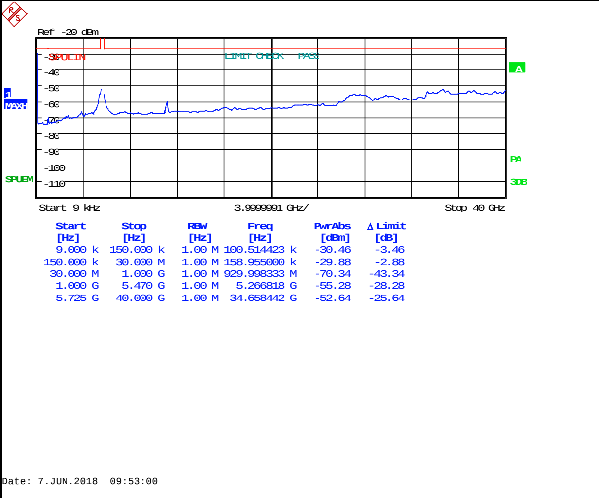
Plot 5-27: Antenna Conducted Spurious Emissions – 5600 MHz 802.11a 20 MHz BW
