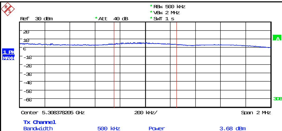
Plot 8-23: PSD – 5290 MHz 802.11ac 80 MHz
