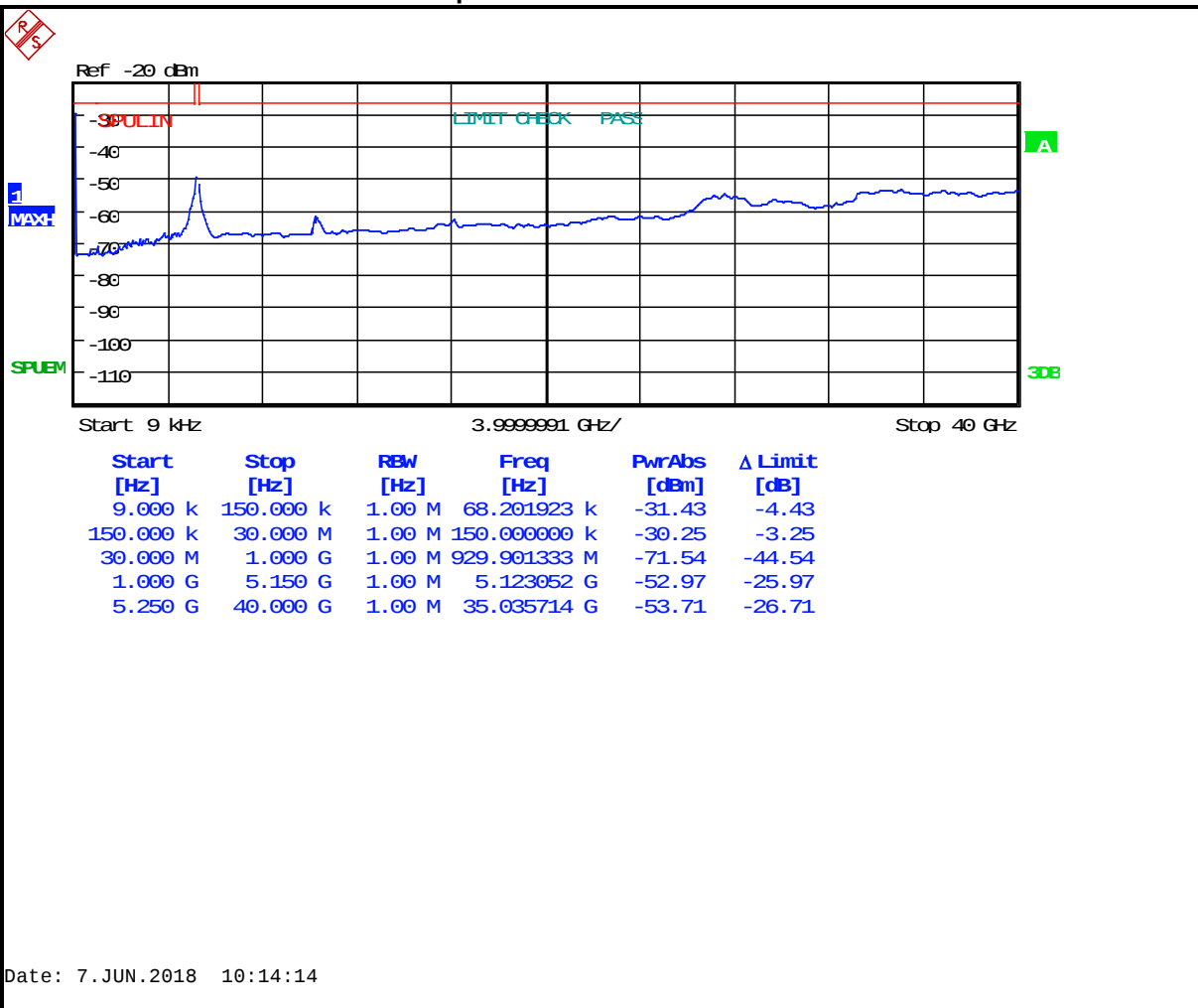
Plot 5-5: Antenna Conducted Spurious Emissions – 5200 MHz 802.11n 20 MHz BW
