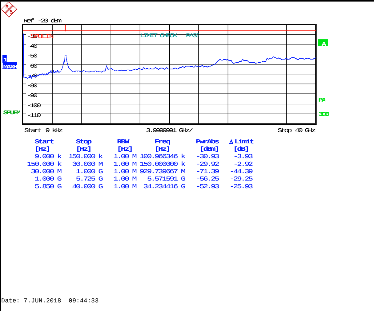
Plot 5-40: Antenna Conducted Spurious Emissions – 5785 MHz 802.11n 20 MHz BW
