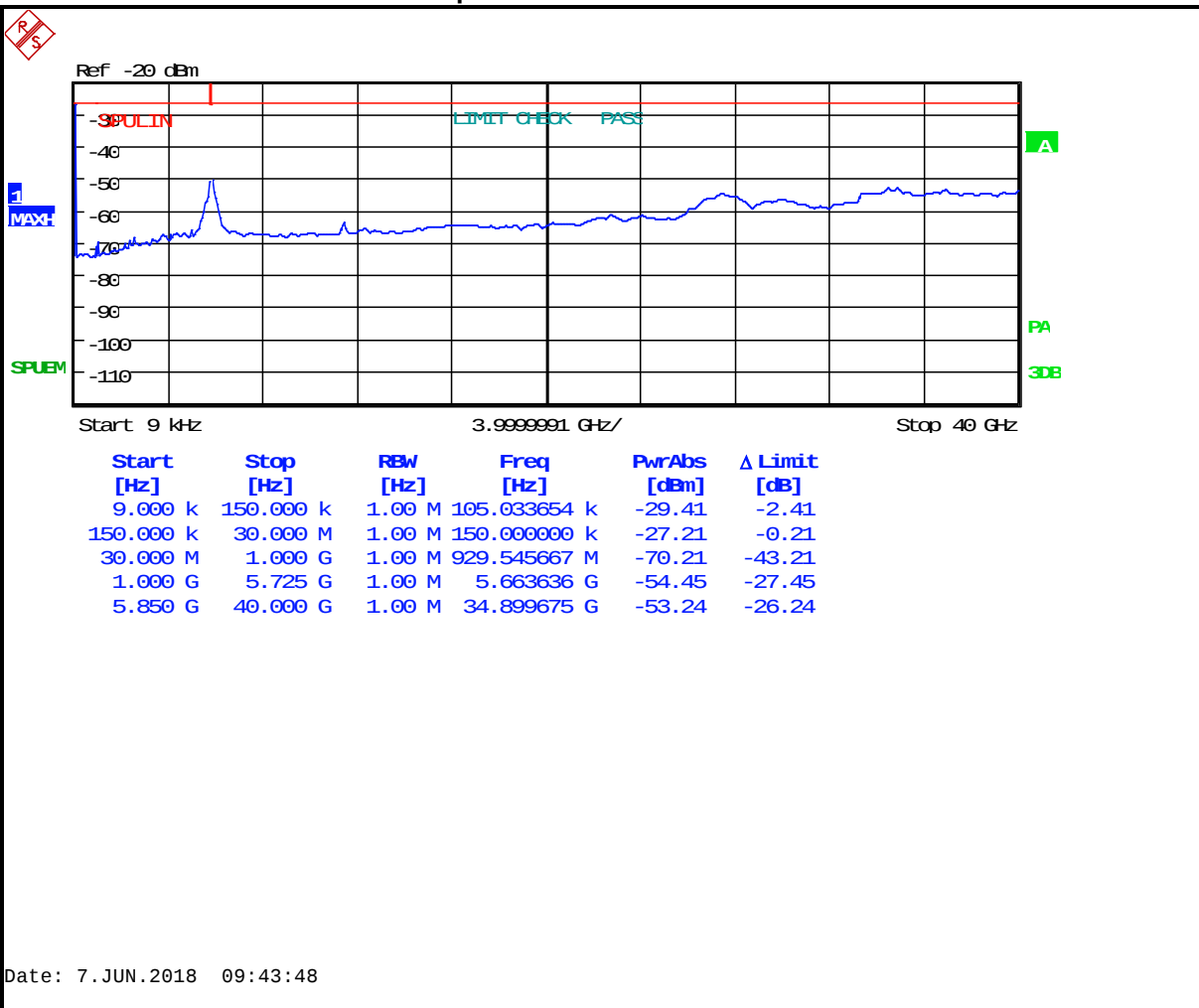
Plot 5-39: Antenna Conducted Spurious Emissions – 5785 MHz 802.11a 20 MHz BW
