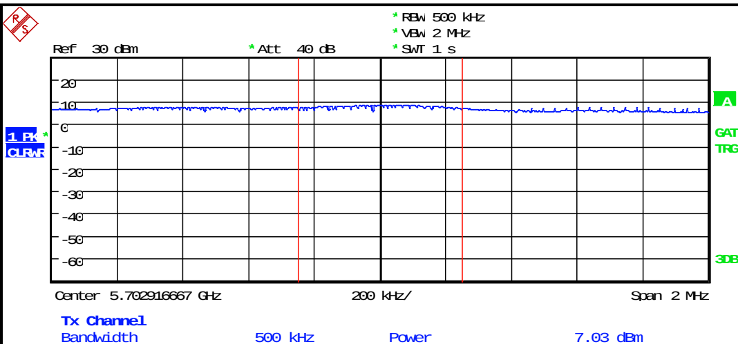
Plot 8-30: PSD – 5700 MHz 802.11a 20 MHz
