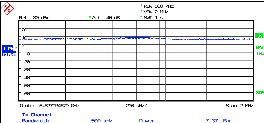
Plot 8-42: PSD – 5825 MHz 802.11a 20 MHz
