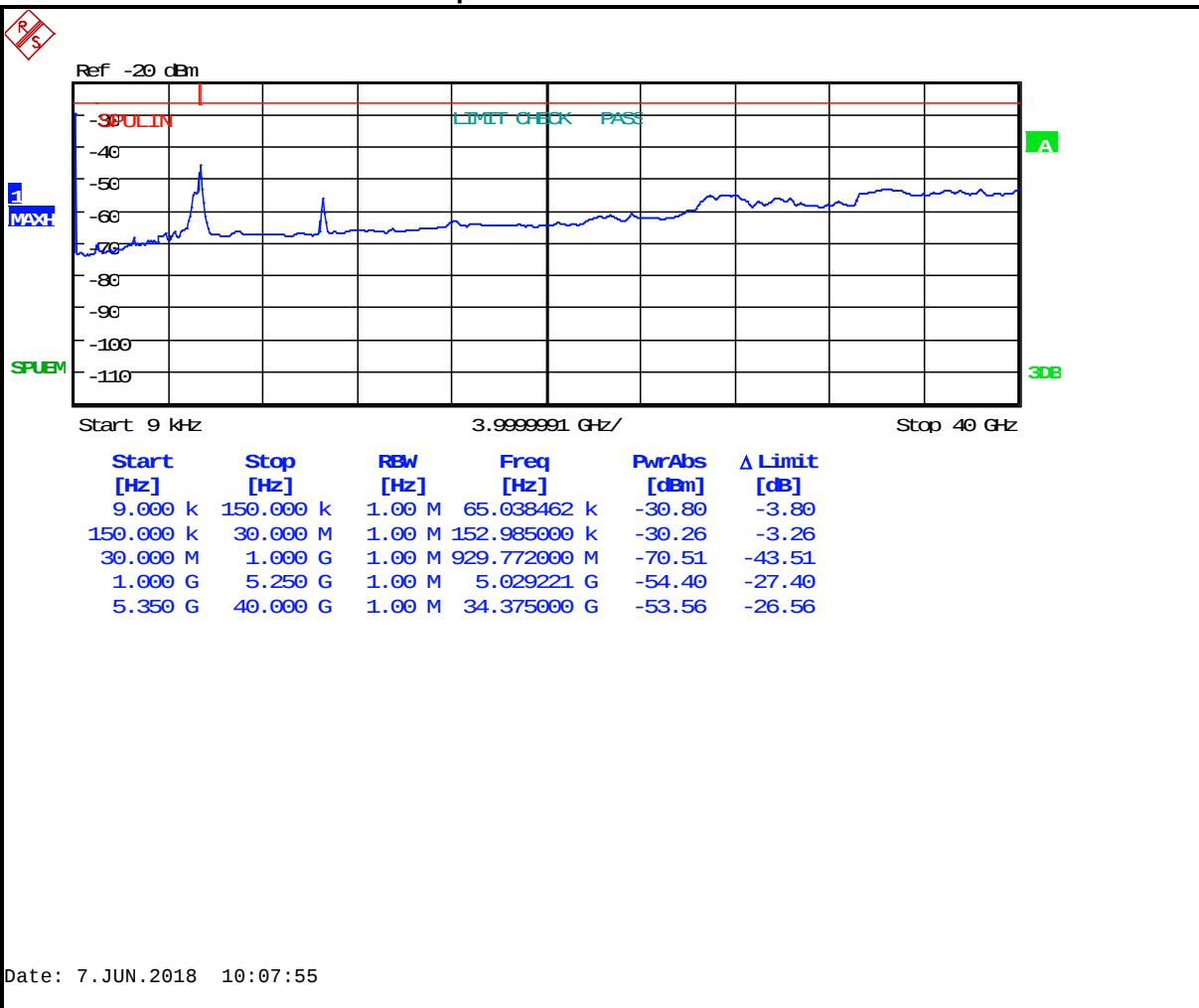
Plot 5-21: Antenna Conducted Spurious Emissions – 5320 MHz 802.11n 20 MHz BW
