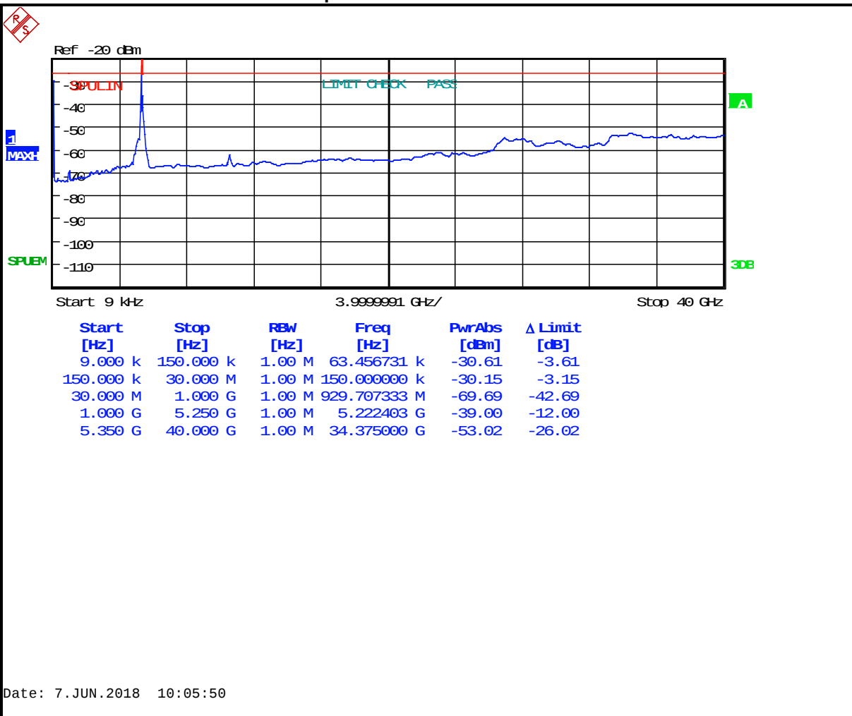
Plot 5-19: Antenna Conducted Spurious Emissions – 5280 MHz 802.11n 40 MHz BW
