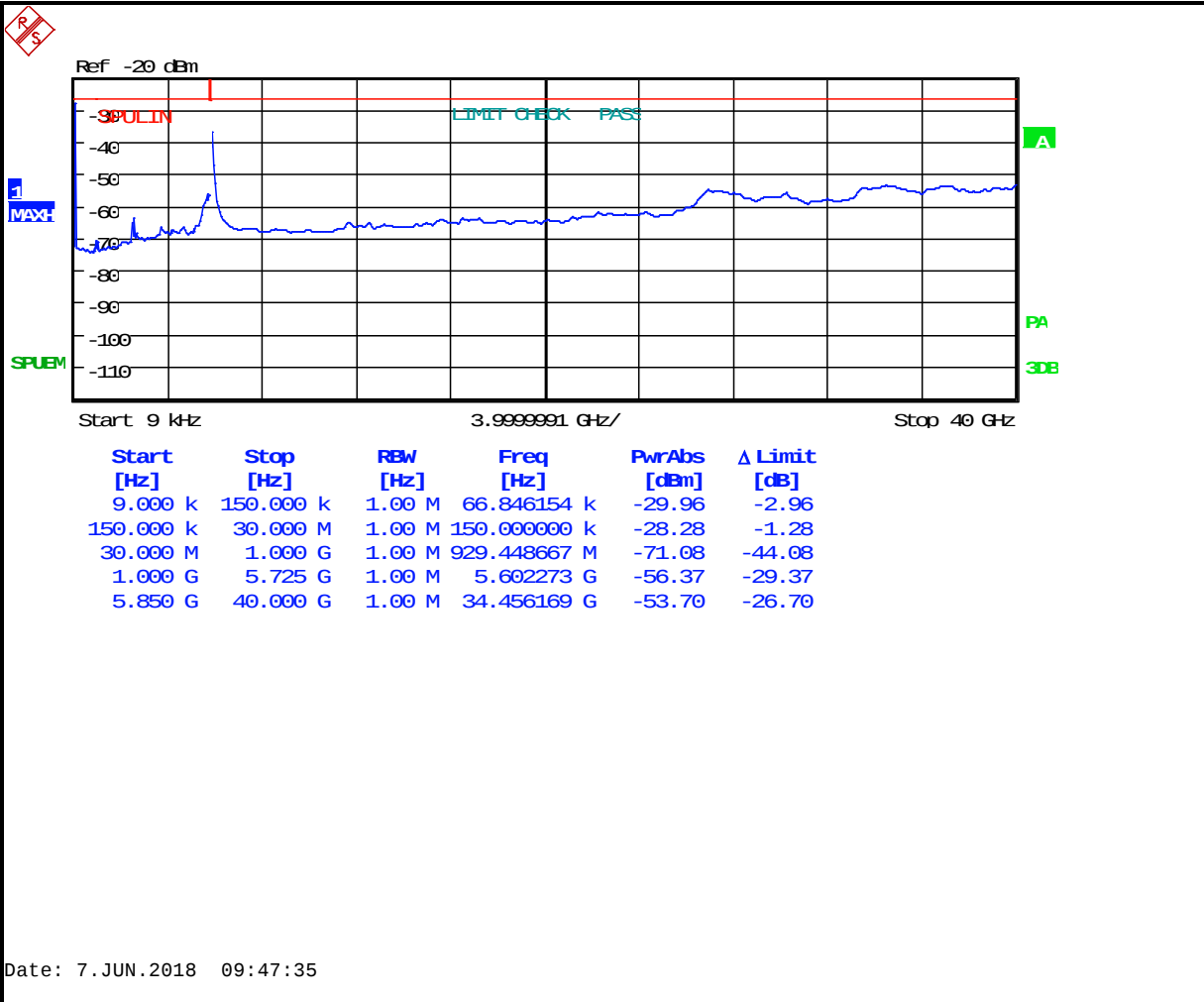
Plot 5-43: Antenna Conducted Spurious Emissions – 5825 MHz 802.11n 20 MHz BW
