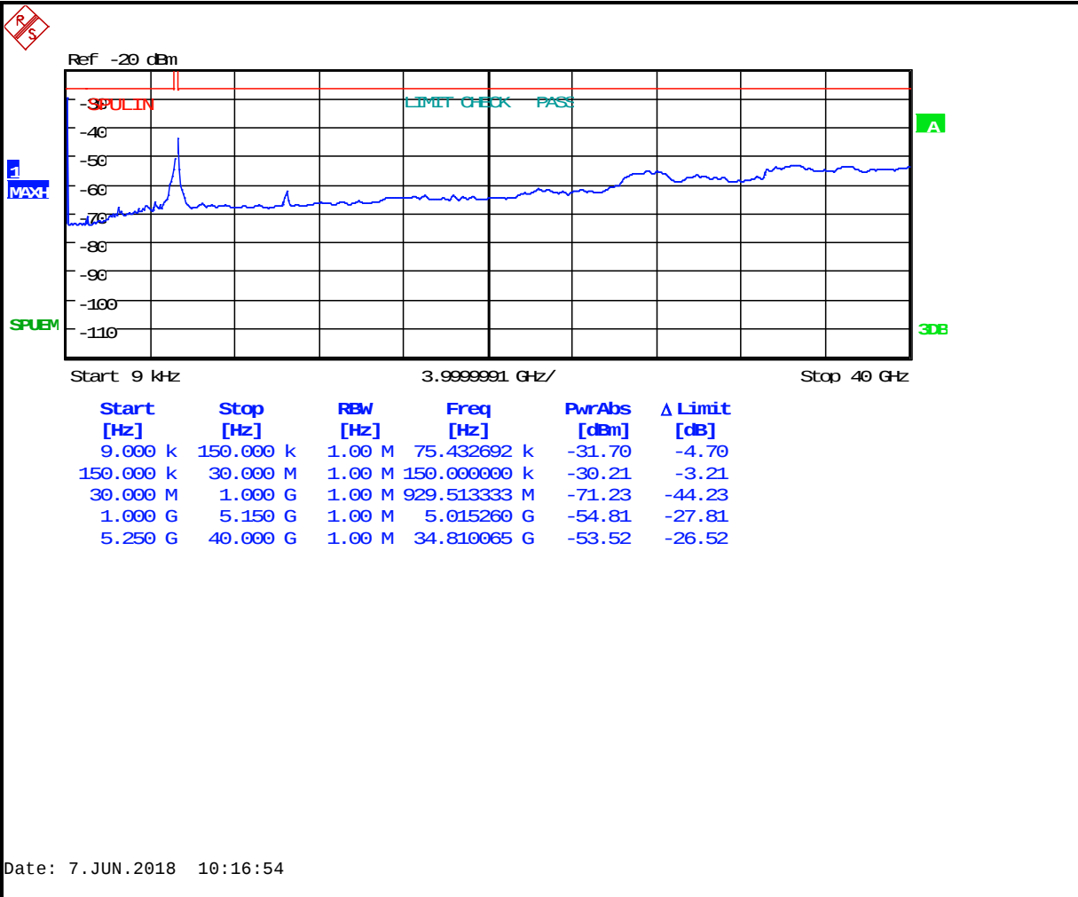
Plot 5-8: Antenna Conducted Spurious Emissions – 5220 MHz 802.11n 20 MHz BW
