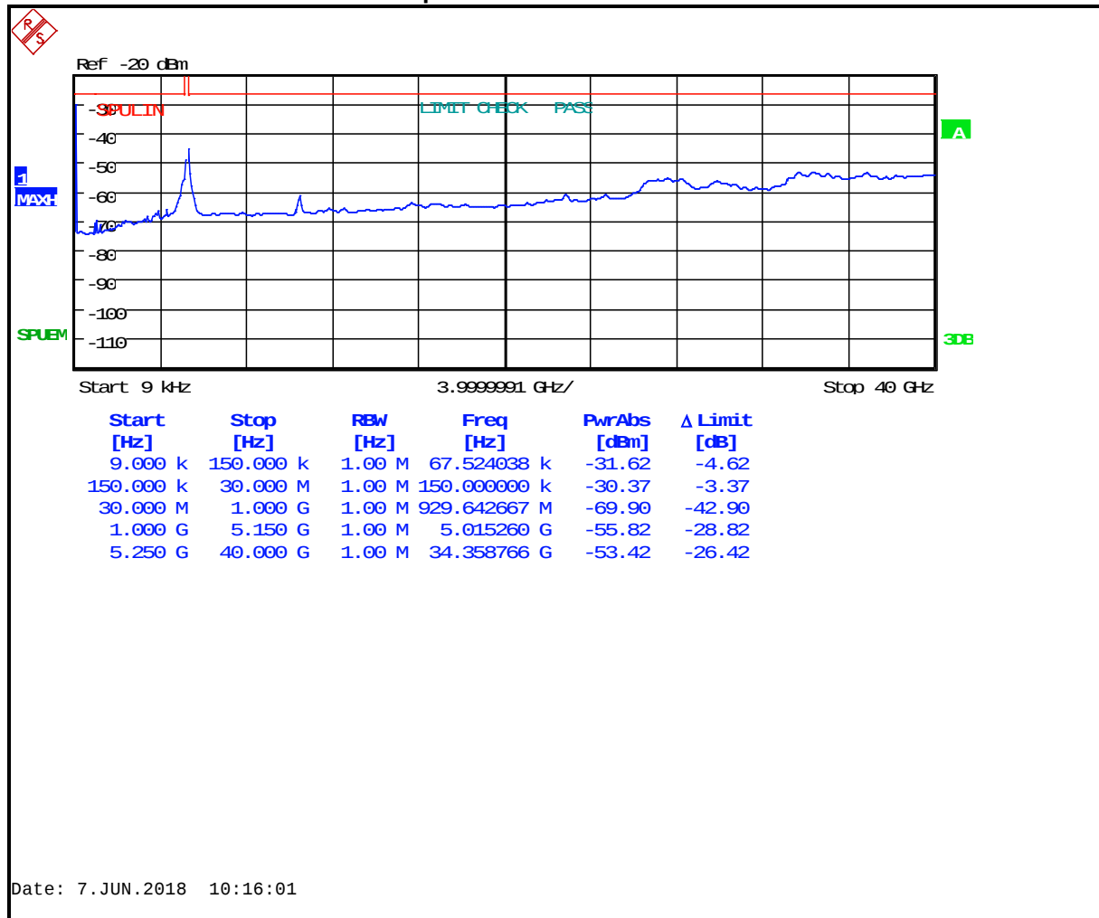
Plot 5-7: Antenna Conducted Spurious Emissions – 5220 MHz 802.11a 20 MHz BW
