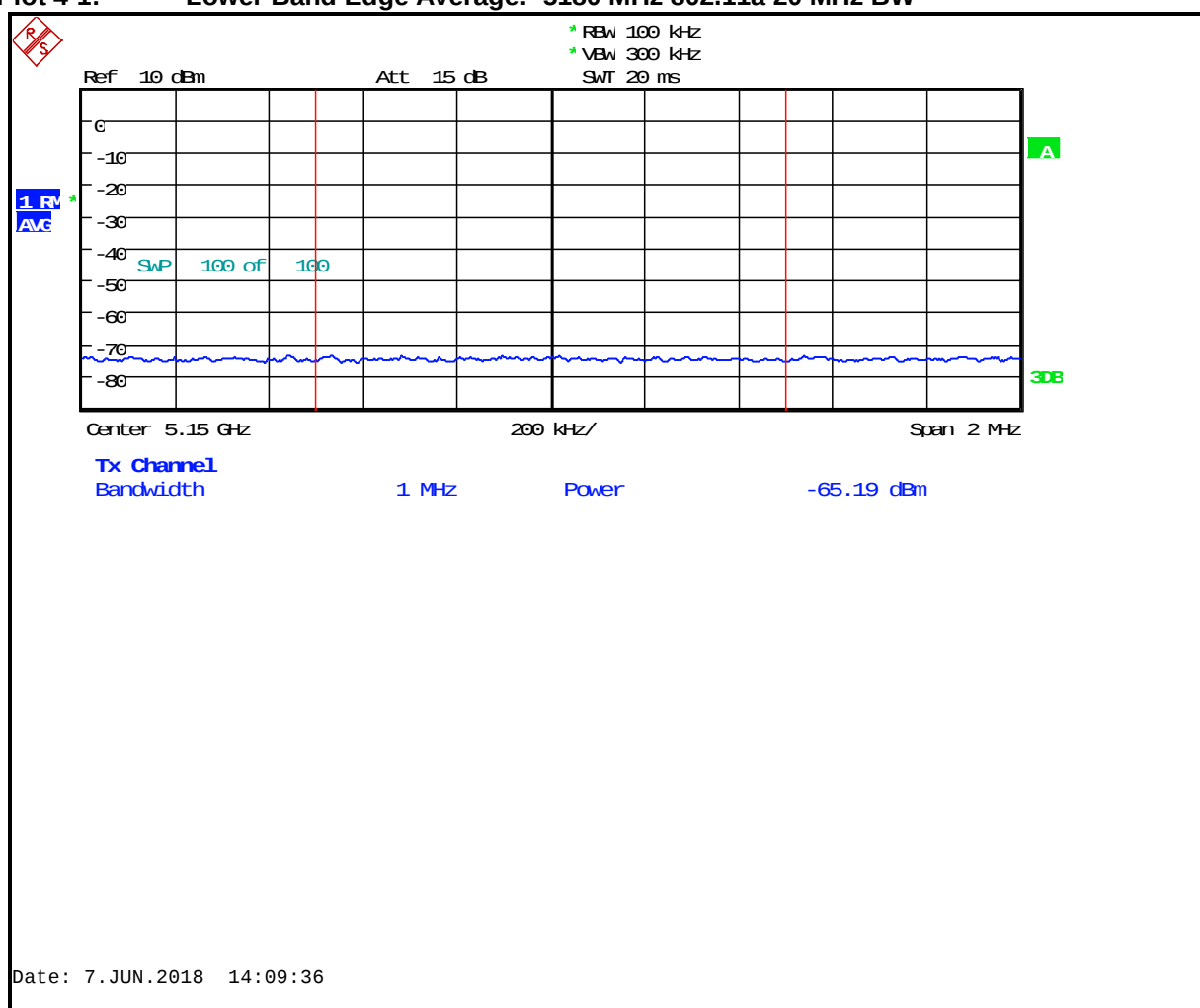
Plot 4-1: Lower Band Edge Average: 5180 MHz 802.11a 20 MHz BW
