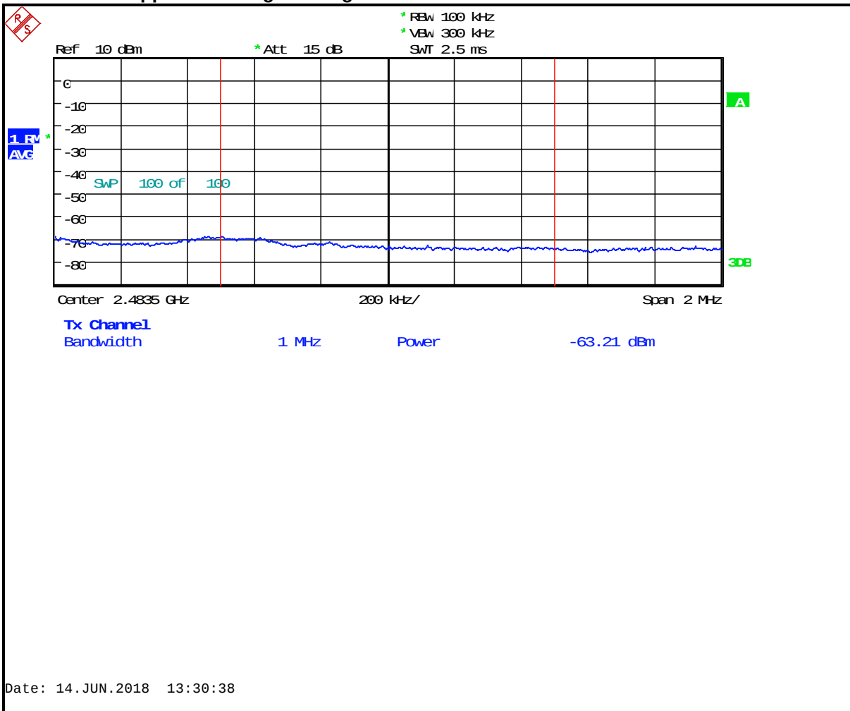
Plot 4-9: Upper Band Edge Average: BLE
