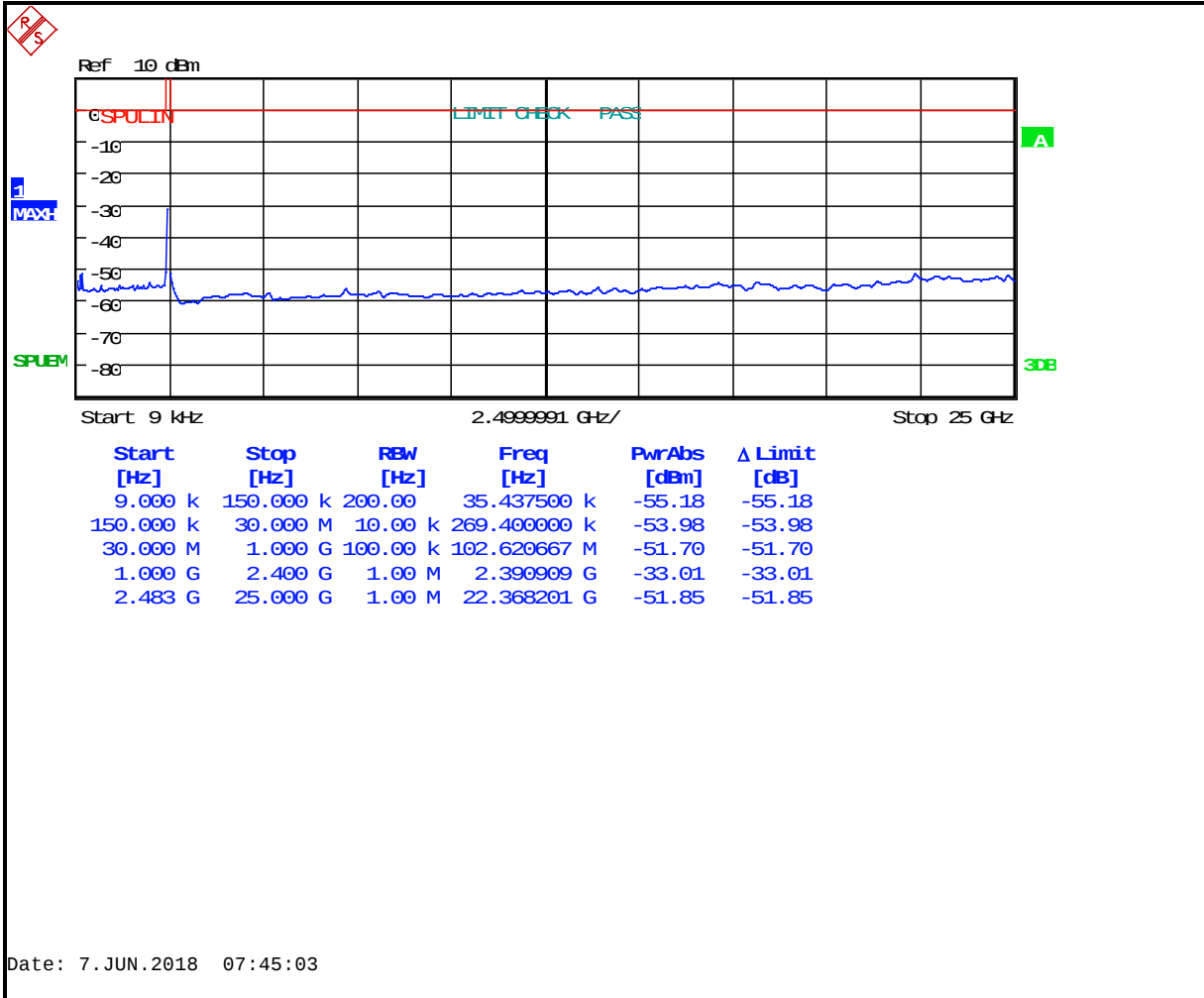
Plot 5-6: Conducted Spurious – 802.11n (MCS7) – 2412 MHz
