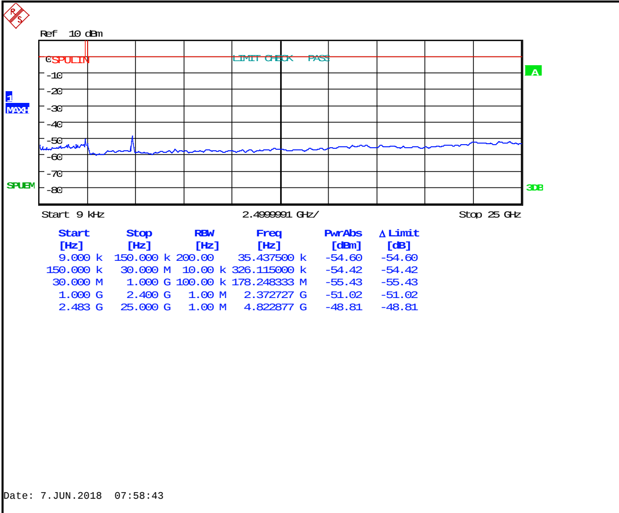
Plot 5-2: Conducted Spurious – BLE – 2440 MHz
