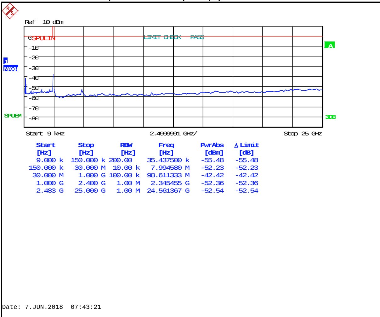
Plot 5-4: Conducted Spurious – 802.11b (11 Mbps) – 2412 MHz
