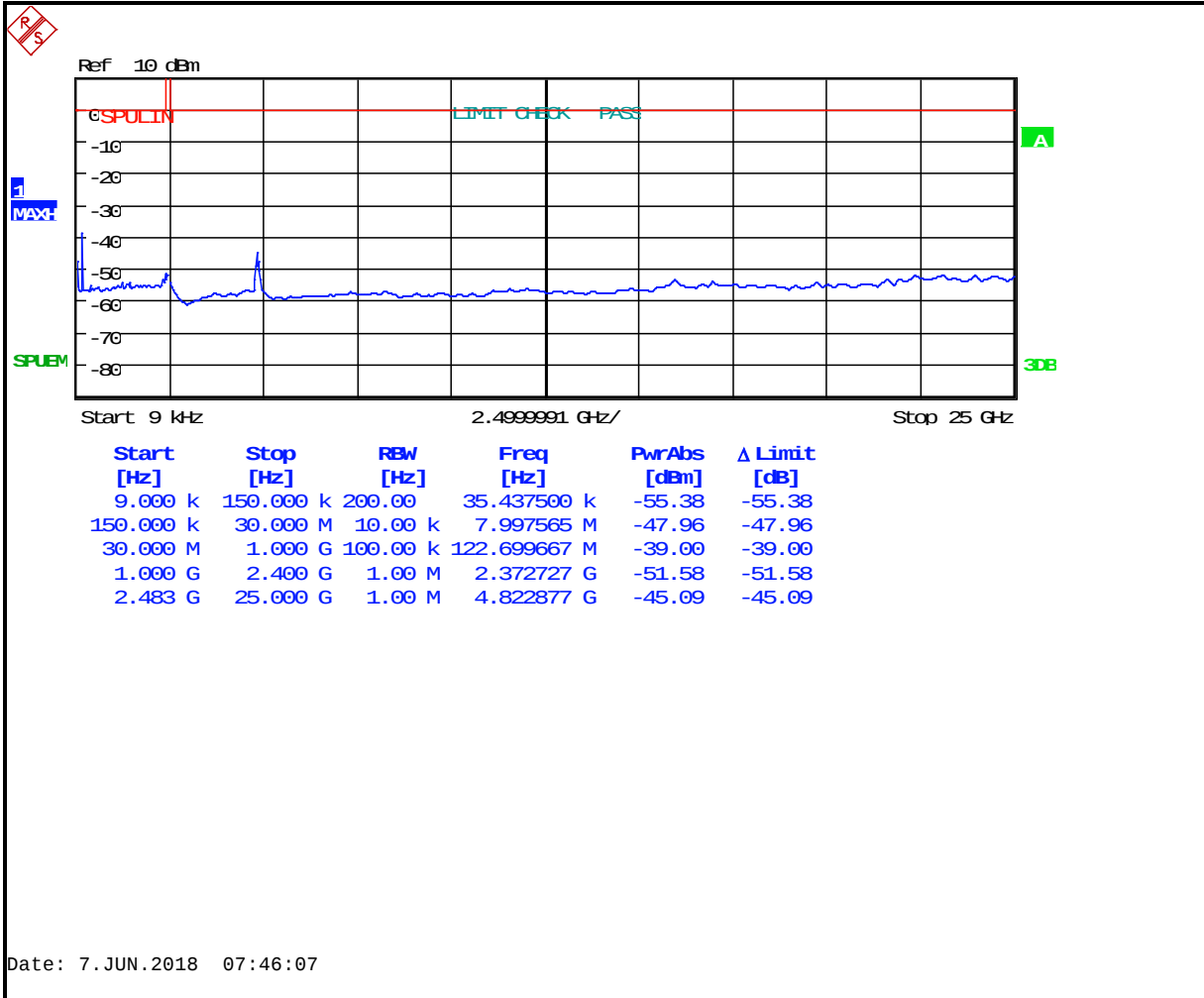
Plot 5-7: Conducted Spurious – 802.11b (11 Mbps) – 2437 MHz
