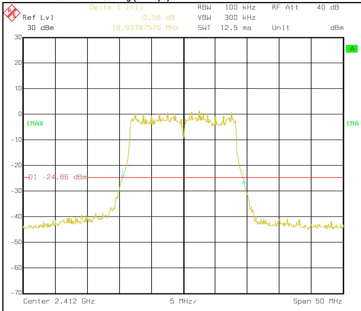
Plot 7-7: 99% OBW – 802.11g (54 Mbps) – 2412 MHz
