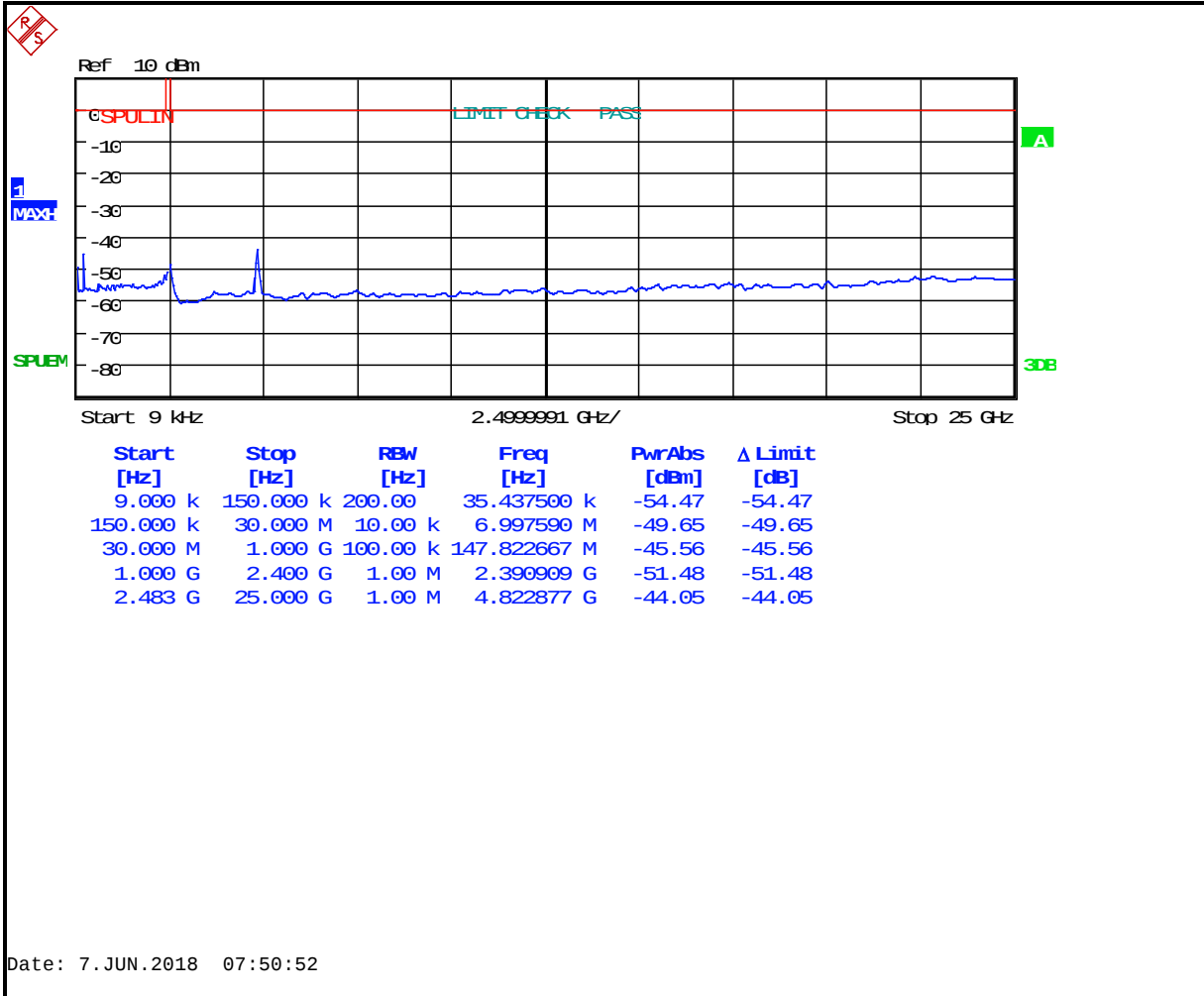
Plot 5-10: Conducted Spurious – 802.11b (11 Mbps) – 2462 MHz
