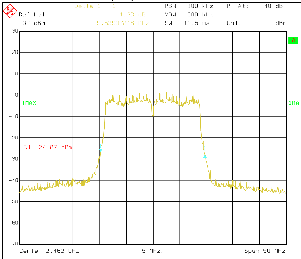
Plot 7-12: 99% OBW – 802.11n (MCS7) – 2462 MHz
