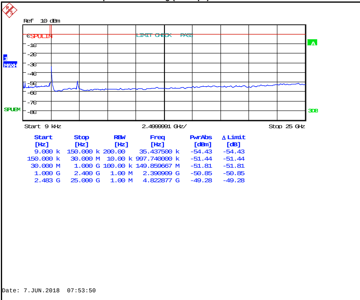
Plot 5-11: Conducted Spurious – 802.11g (54 Mbps) – 2462 MHz
