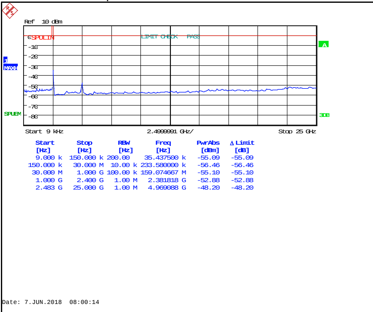
Plot 5-3: Conducted Spurious – BLE – 2480 MHz
