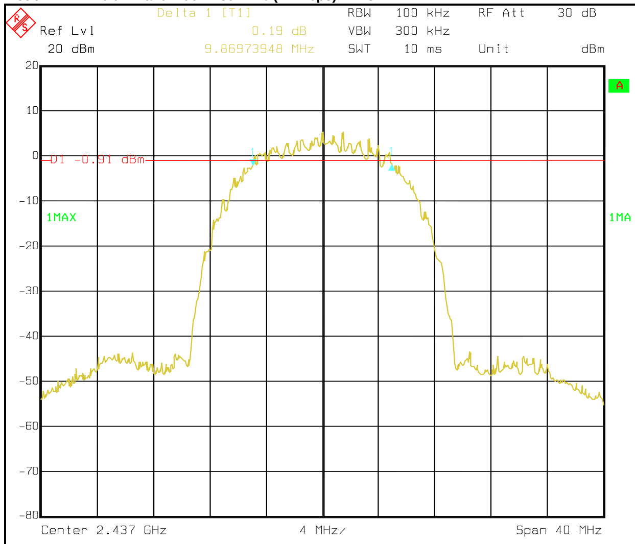
Plot 6-7: 6 dB Bandwidth – 802.11b (11 Mbps) – 2437 MHz
