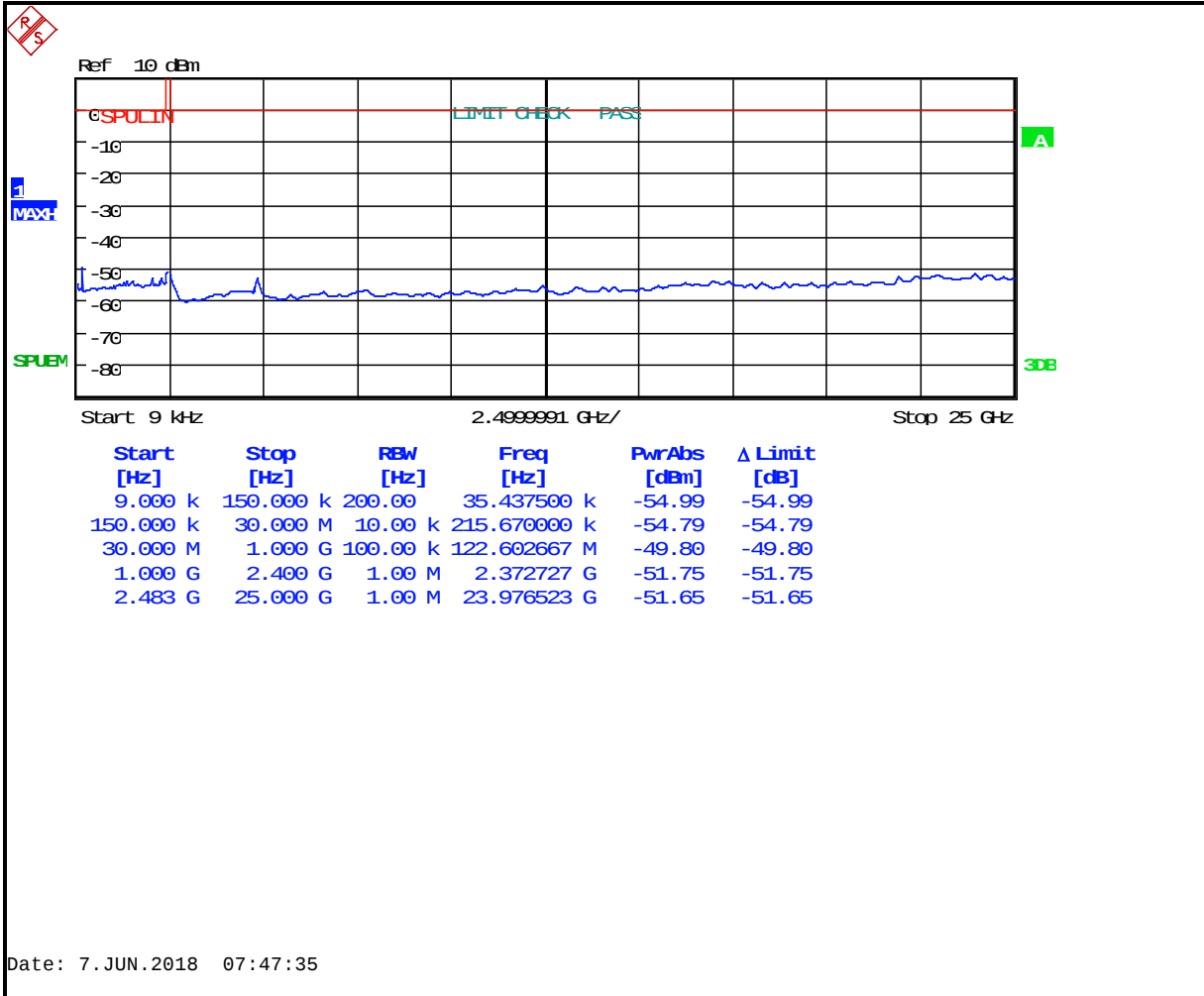
Plot 5-8: Conducted Spurious – 802.11g (54 Mbps) – 2437 MHz
