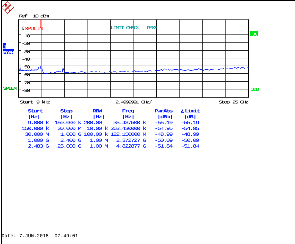
Plot 5-9: Conducted Spurious – 802.11b (MCS7) – 2437 MHz
