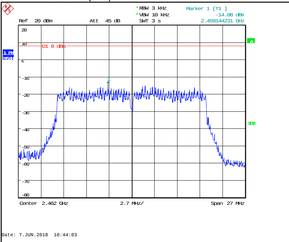
Plot 8-12: PSD – 802.11n (MCS7) – 2462 MHz
