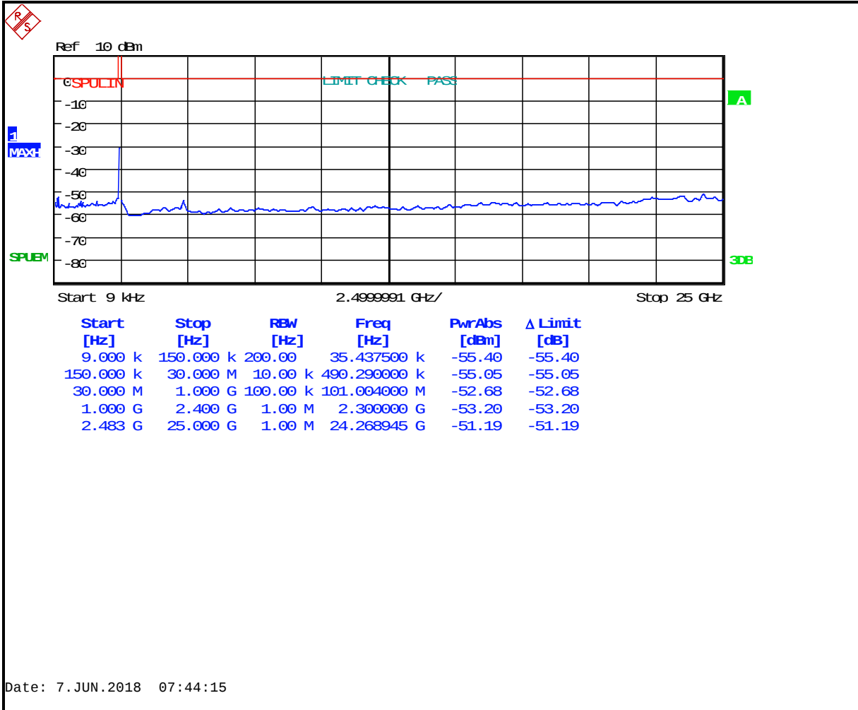
Plot 5-5: Conducted Spurious – 802.11g (54 Mbps) – 2412 MHz
