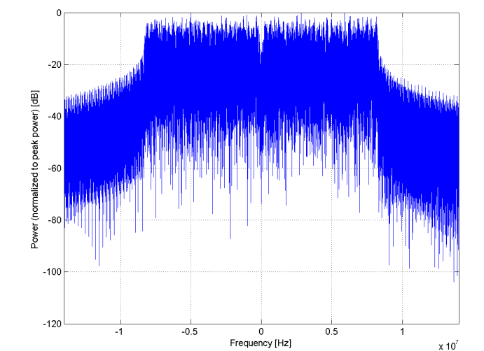
Frequency Domain
