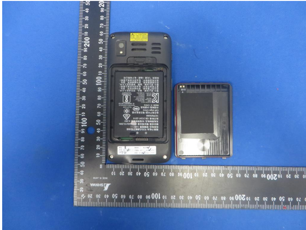
(1) EUT Photo
