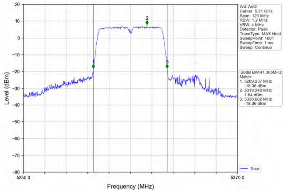
802.11n(HT40)_HCH_5310MHz_Ant2_NTNV
