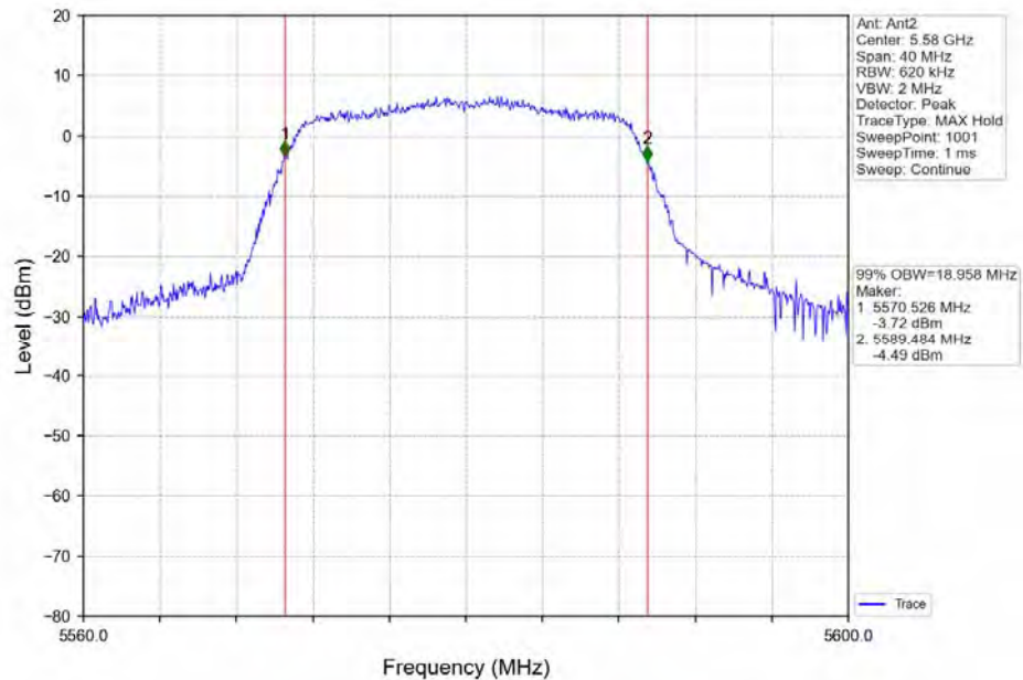
802.11ac(VHT20) MCH_5580MHz_Ant2_NTNV
