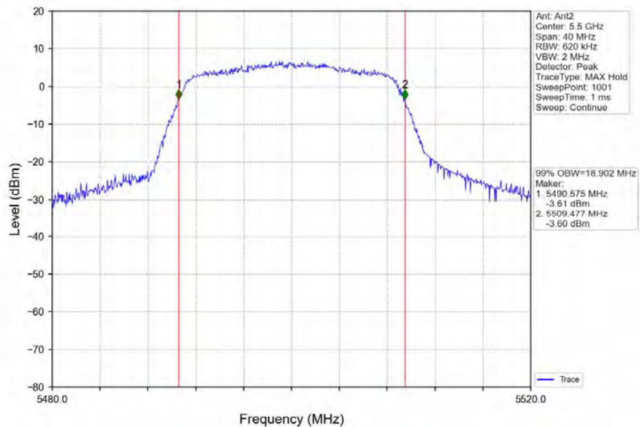
802.11ac(VHT20)_LCH_5500MHz_Ant2_NTNV
