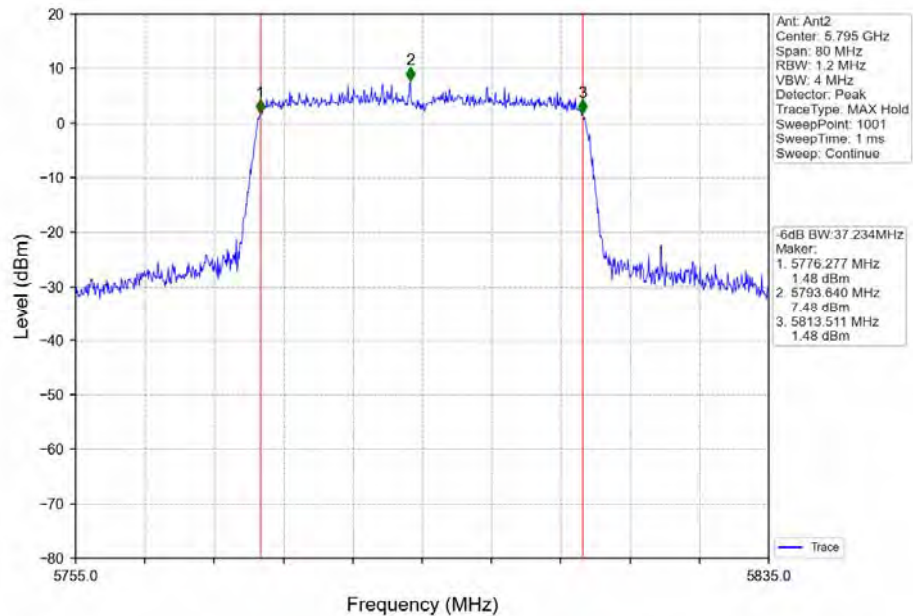
802.11ax(HEW40) HCH_5795MHz_Ant2_NTNV
