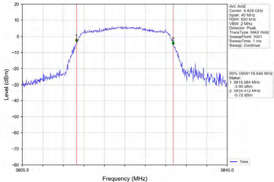
802.11ac(VHT20) HCH_5825MHz_Ant2_NTNV
