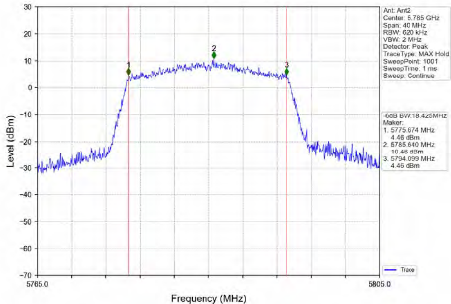
802.11ax(HEW20)_MCH_5785MHz_Ant2_NTNV
