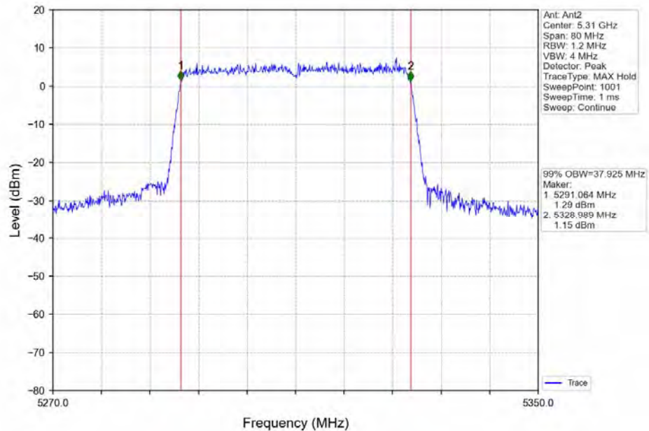
802.11ax(HEW40) HCH_5310MHz_Ant2_NTNV
