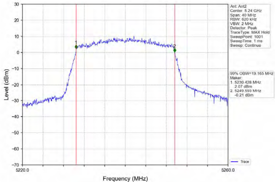
802.11ax(HEW20)_HCH_5240MHz_Ant2_NTNV
