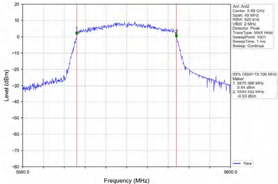
802.11ax(HEW20)_MCH_5580MHz_Ant2_NTNV
