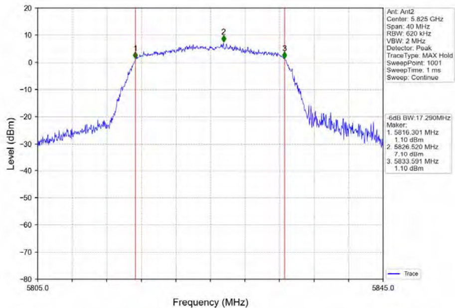
802.11ac(VHT20) HCH_5825MHz_Ant2_NTNV
