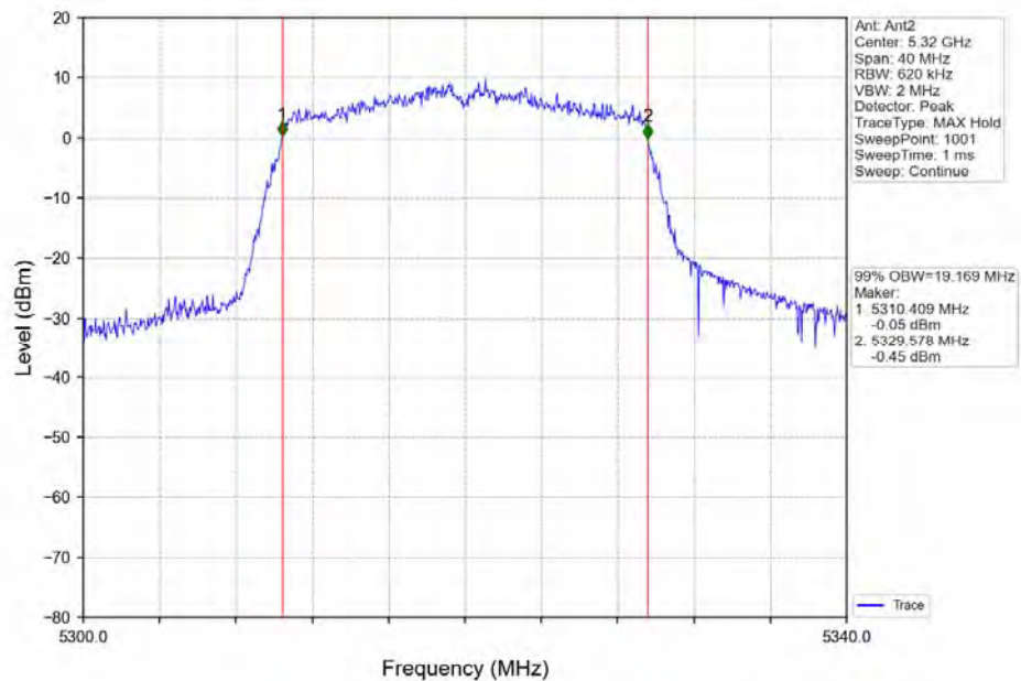
802.11ax(HEW20)_HCH_5320MHz_Ant2_NTNV
