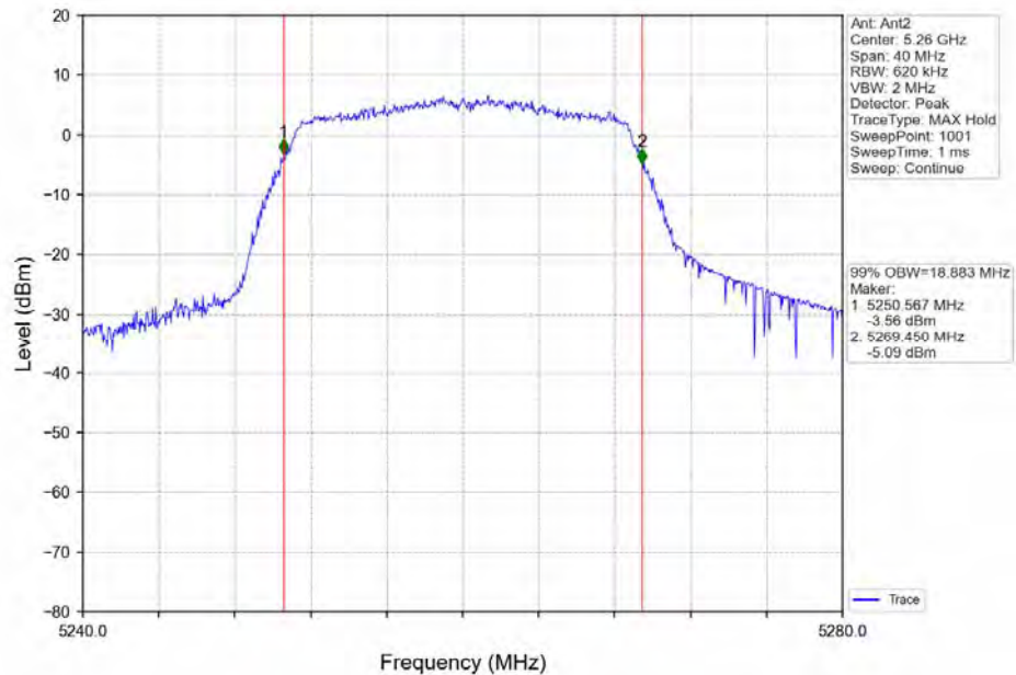
802.11ac(VHT20)_LCH_5260MHz_Ant2_NTNV
