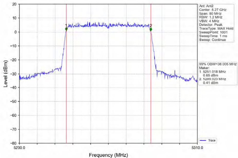
802.11ax(HEW40)_LCH_5270MHz_Ant2_NTNV
