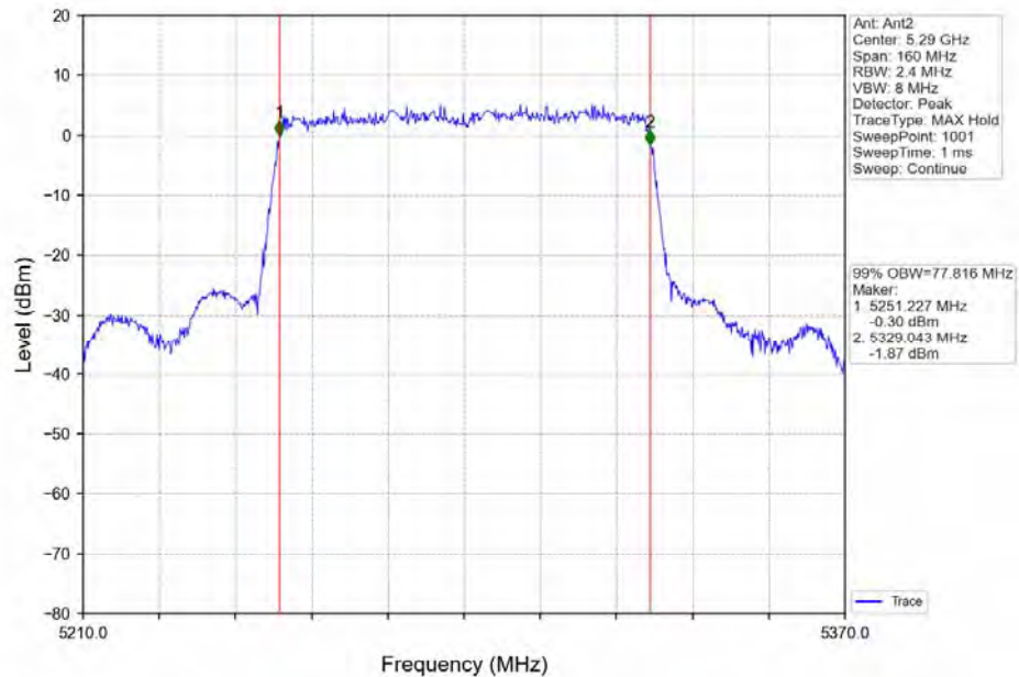
802.11ax(HEW80)_MCH_5290MHz_Ant2_NTNV
