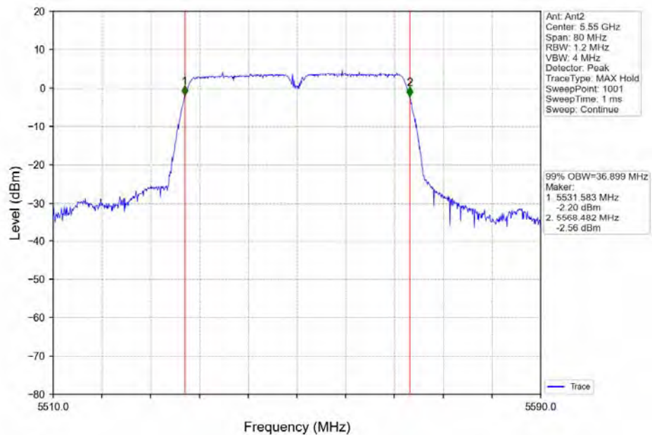
802.11ac(VHT40) MCH_5550MHz_Ant2_NTNV
