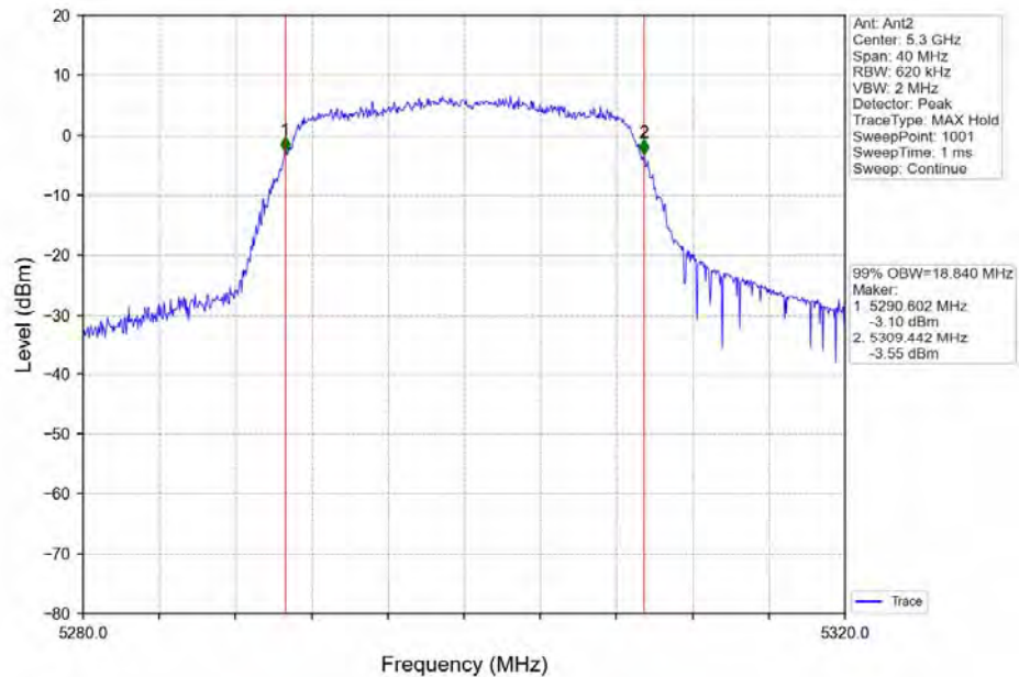
802.11ac(VHT20) MCH_5300MHz_Ant2_NTNV
