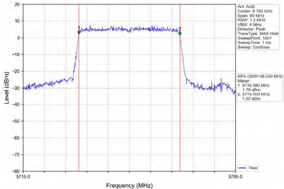
802.11ax(HEW40)_LCH_5755MHz_Ant2_NTNV
