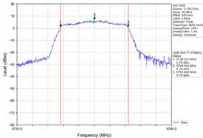
802.11ac(VHT20)_LCH_5745MHz_Ant2_NTNV
