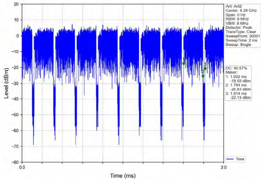
802.11ac(VHT80)_MCH_5290MHz_Ant2_NTNV_MIMO
