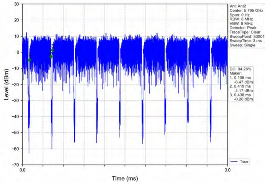
802.11ax(HEW40)_HCH_5795MHz_Ant2_NTNV_MIMO
