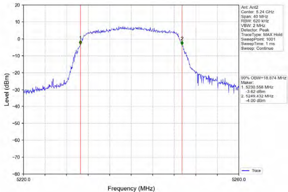
802.11n(HT20)_HCH_5240MHz_Ant2_NTNV
