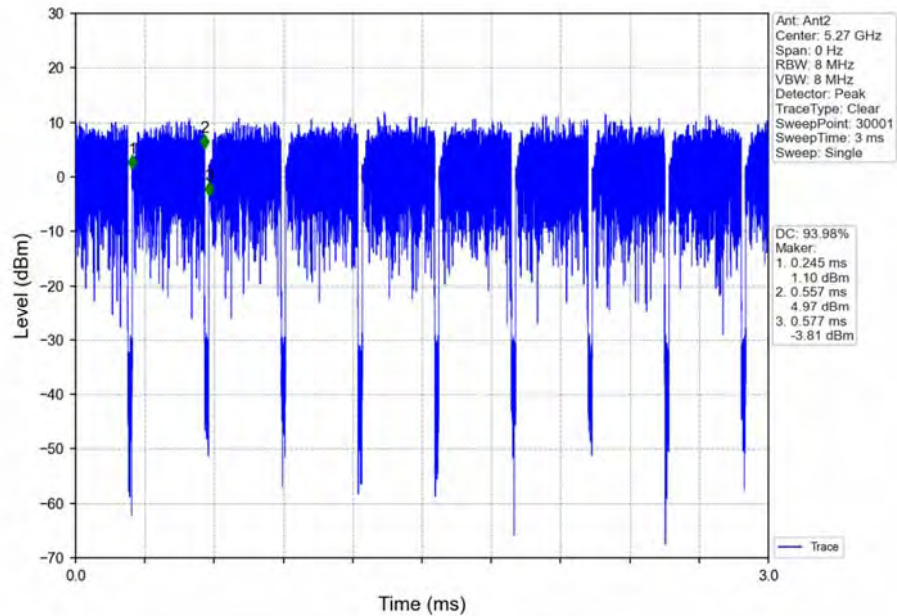
802.11ax(HEW40) LCH_5270MHz_Ant2_NTNV_MIMO
