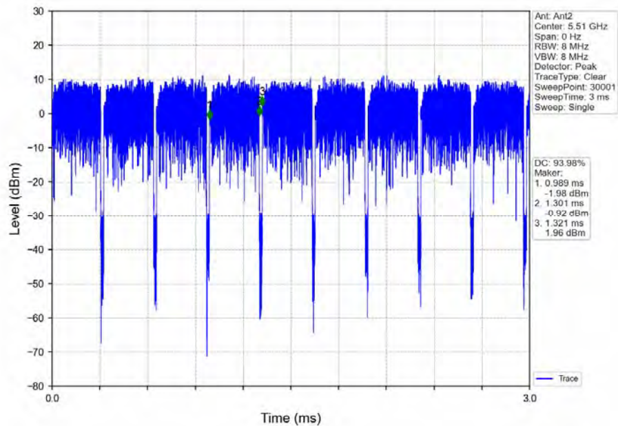
802.11ax(HEW40)_LCH_5510MHz_Ant2_NTNV_MIMO
