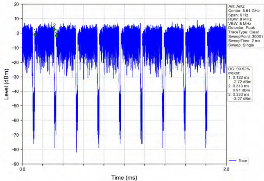
802.11ac(VHT80)_HCH_5610MHz_Ant2_NTNV_MIMO
