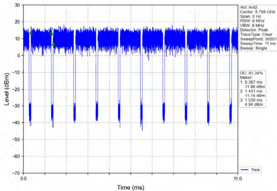
802.11ax(HEW20)_MCH_5785MHz_Ant2_NTNV
