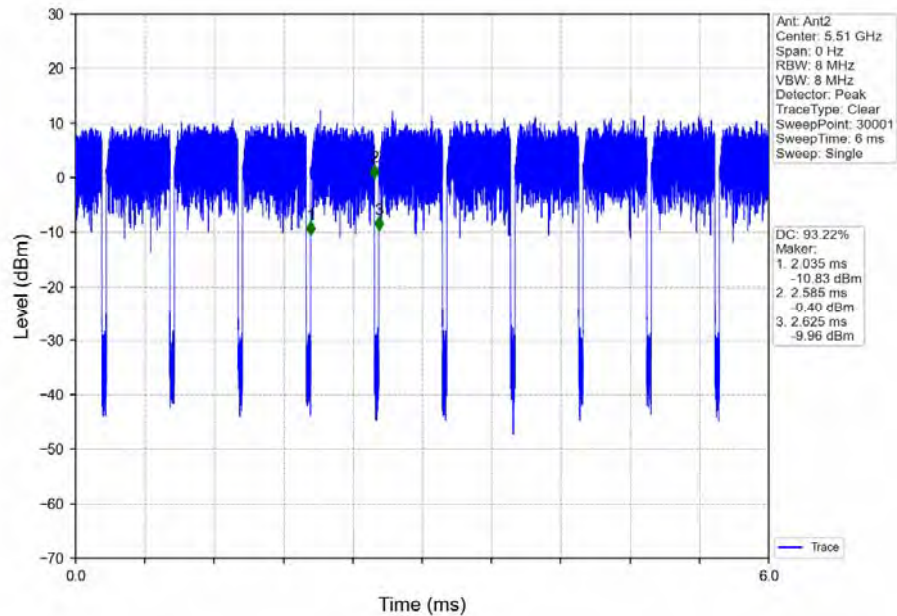
802.11ax(HEW40)_LCH_5510MHz_Ant2_NTNV
