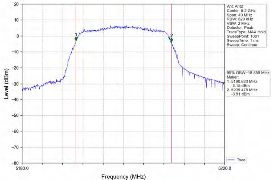
802.11ac(VHT20) MCH_5200MHz_Ant2_NTNV
