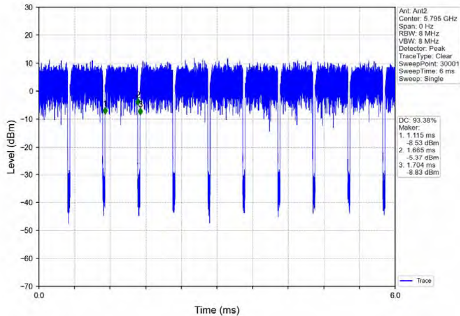
802.11ax(HEW40)_HCH_5795MHz_Ant2_NTNV
