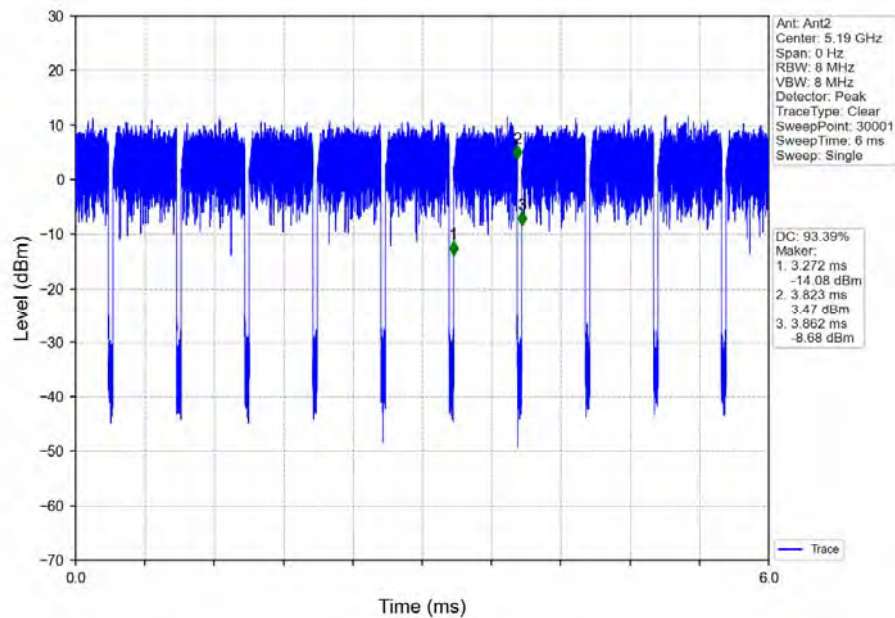
802.11ax(HEW40)_LCH_5190MHz_Ant2_NTNV
