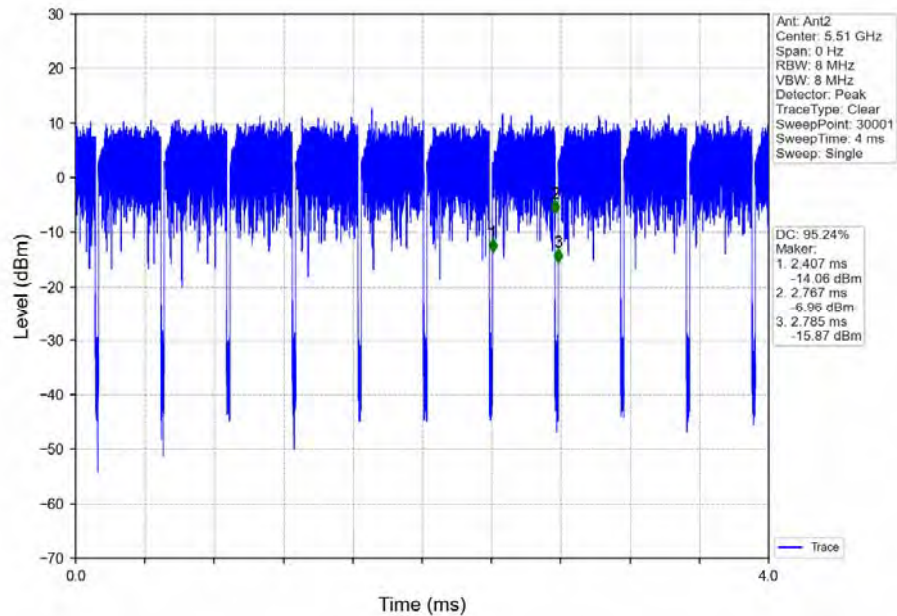
802.11ac(VHT40)_LCH_5510MHz_Ant2_NTNV_MIMO
