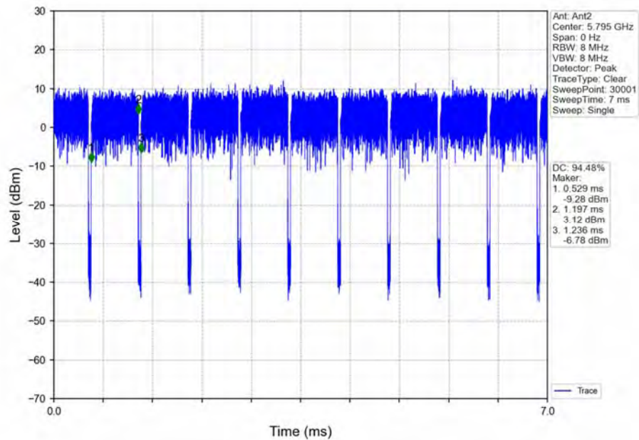
802.11ac(VHT40)_HCH_5795MHz_Ant2_NTNV
