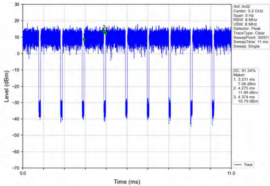
802.11ax(HEW20)_HCH_5240MHz_Ant2_NTNV
