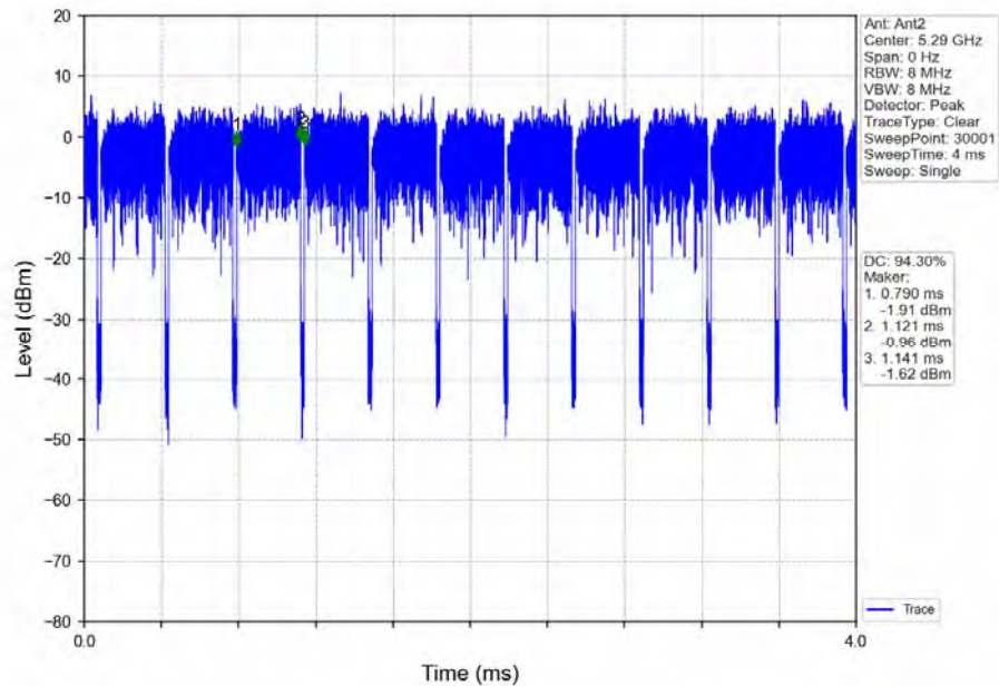
802.11ac(VHT80)_MCH_5290MHz_Ant2_NTNV
