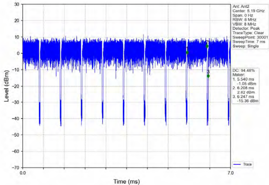
802.11ac(VHT40)_LCH_5190MHz_Ant2_NTNV
