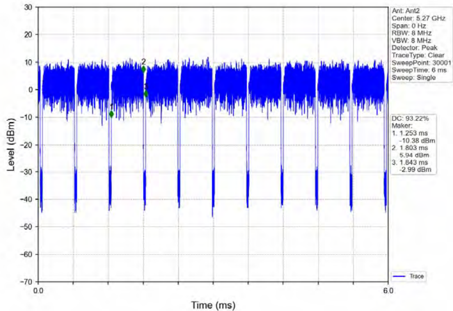
802.11ax(HEW40)_LCH_5270MHz_Ant2_NTNV
