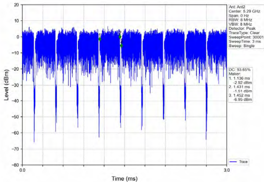
802.11ax(HEW80)_MCH_5290MHz_Ant2_NTNV
