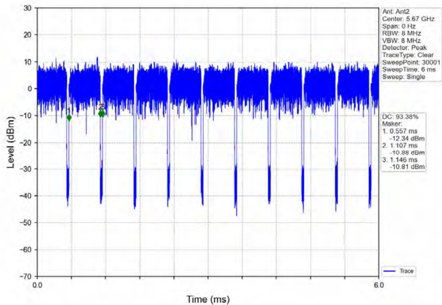
802.11ax(HEW40)_HCH_5670MHz_Ant2_NTNV
