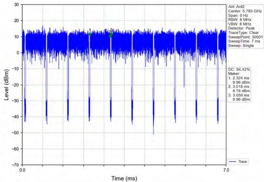
802.11ac(VHT20)_MCH_5785MHz_Ant2_NTNV_MIMO
