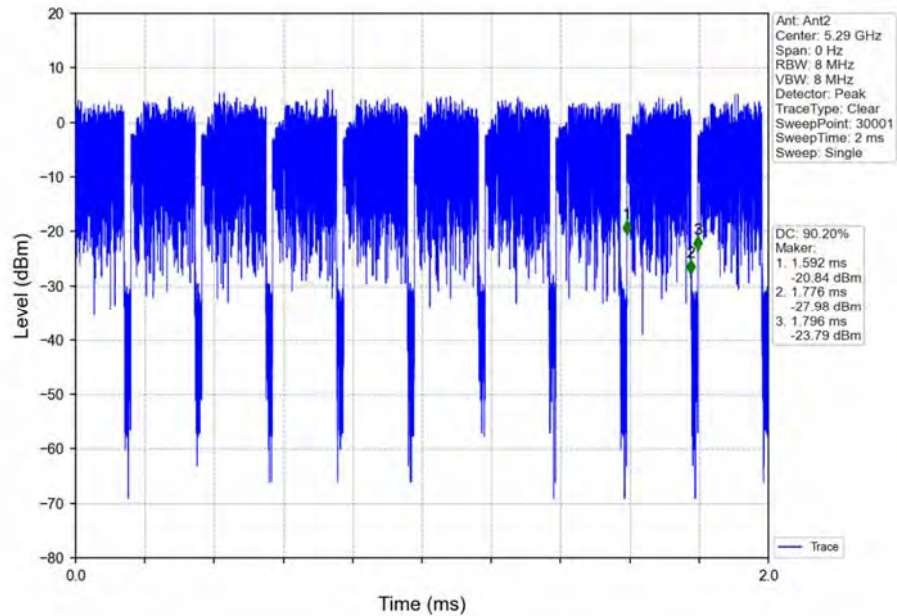
802.11ax(HEW80)_MCH_5290MHz_Ant2_NTNV_MIMO
