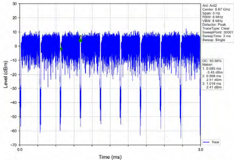
802.11ax(HEW40)_HCH_5670MHz_Ant2_NTNV_MIMO
