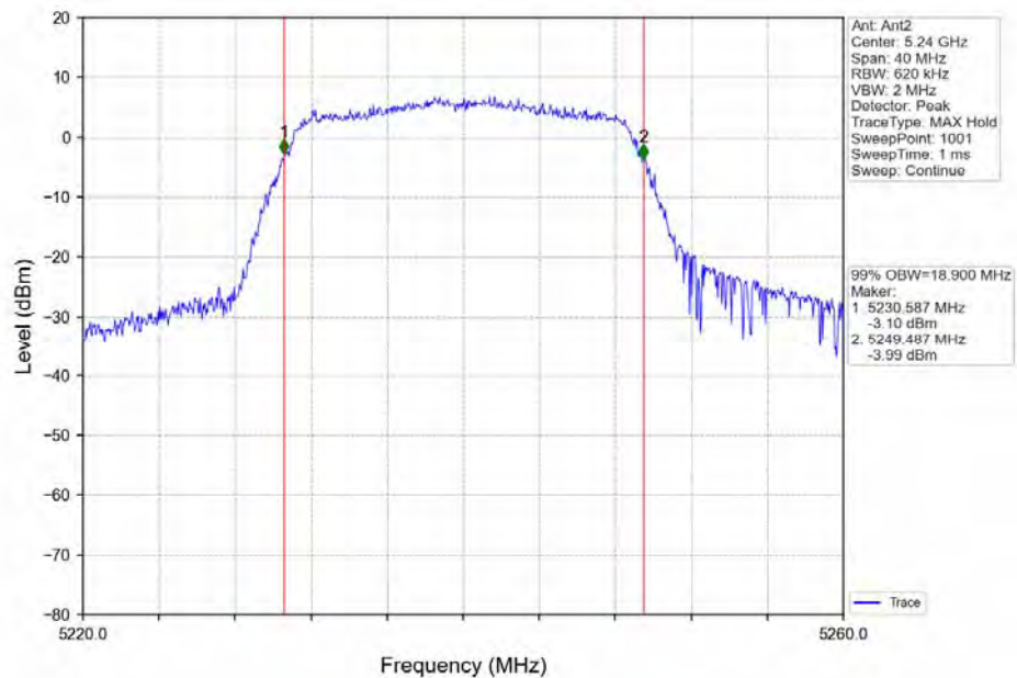
802.11ac(VHT20) HCH_5240MHz_Ant2_NTNV
