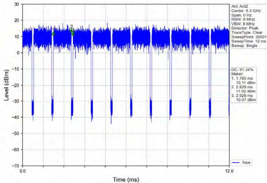
802.11ax(HEW20)_MCH_5300MHz_Ant2_NTNV
