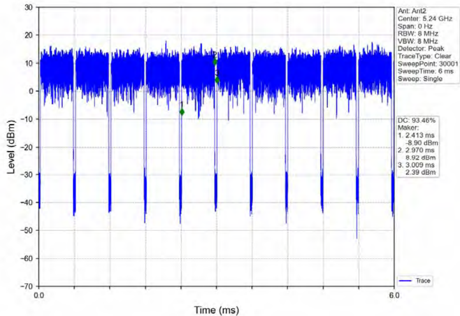
802.11ax(HEW20)_HCH_5240MHz_Ant2_NTNV_MIMO
