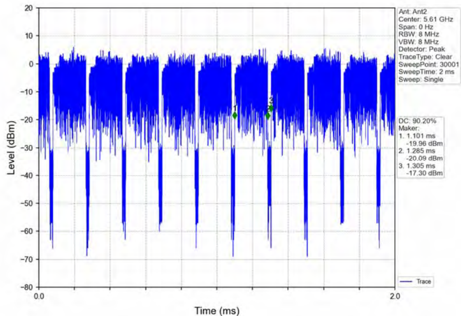
802.11ax(HEW80)_HCH_5610MHz_Ant2_NTNV_MIMO
