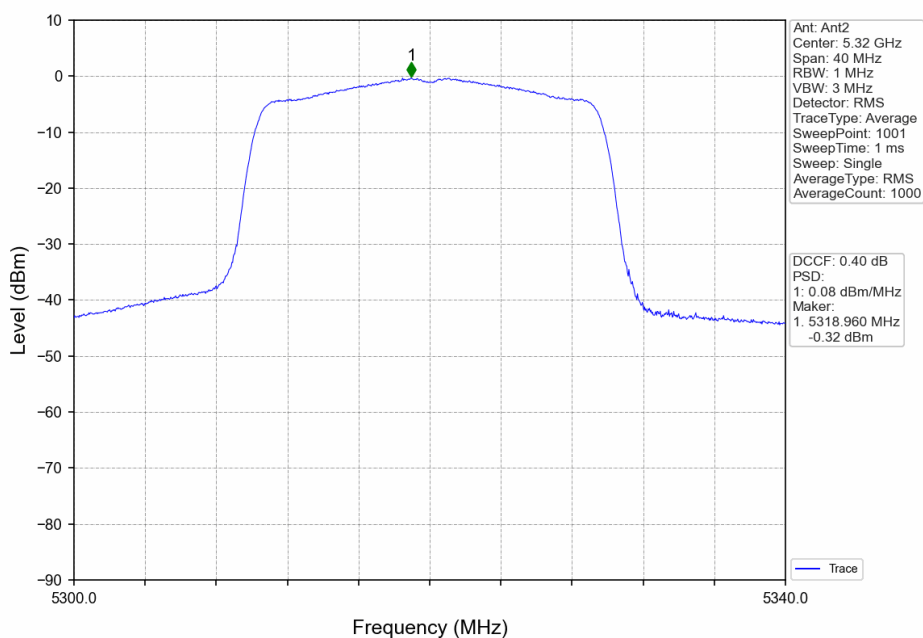
802.11ax(HEW20)_HCH_5320MHz_Ant2_NTNV
