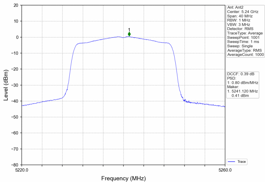
802.11ax(HEW20)_HCH_5240MHz_Ant2_NTNV
