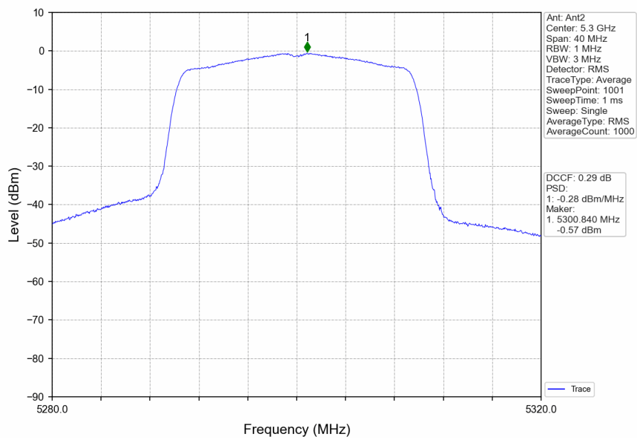
802.11ax(HEW20)_MCH_5300MHz_Ant2_NTNV
