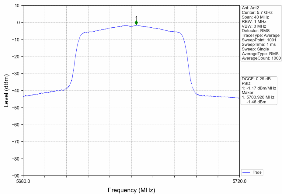
802.11ax(HEW20)_HCH_5700MHz_Ant2_NTNV
