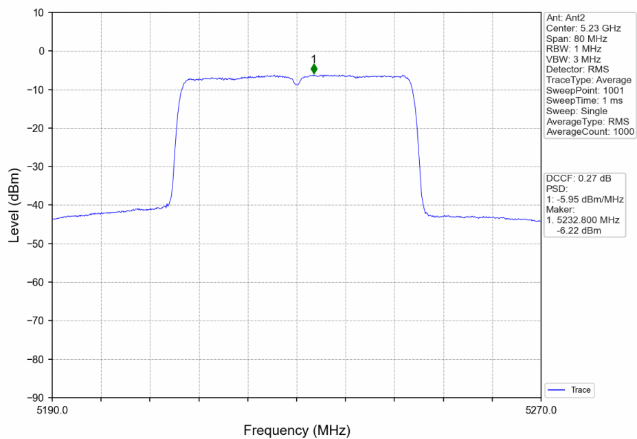
802.11ax(HEW40)_HCH_5230MHz_Ant2_NTNV
