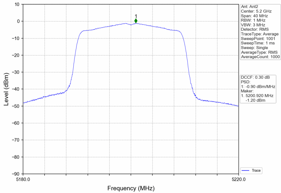
802.11ax(HEW20)_MCH_5200MHz_MIMO_NTNV
