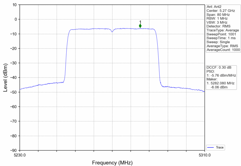
802.11ax(HEW40)_LCH_5270MHz_Ant2_NTNV
