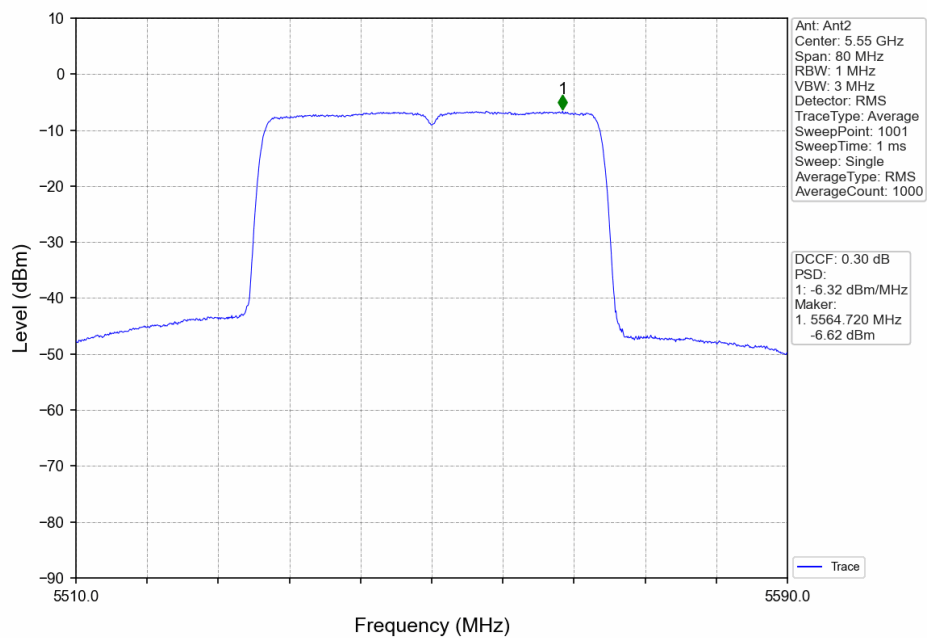
802.11ax(HEW40)_MCH_5550MHz_Ant2_NTNV
