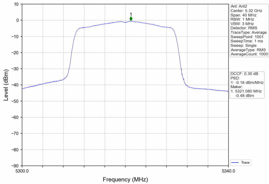
802.11ax(HEW20)_HCH_5320MHz_MIMO_NTNV
