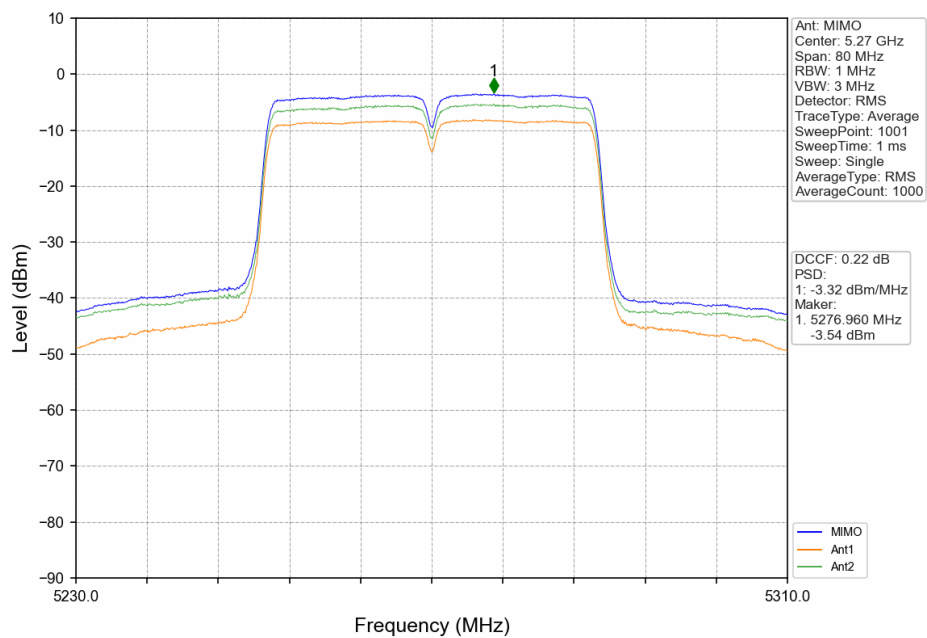
802.11ac(VHT40)_LCH_5270MHz_MIMO_NTNV
