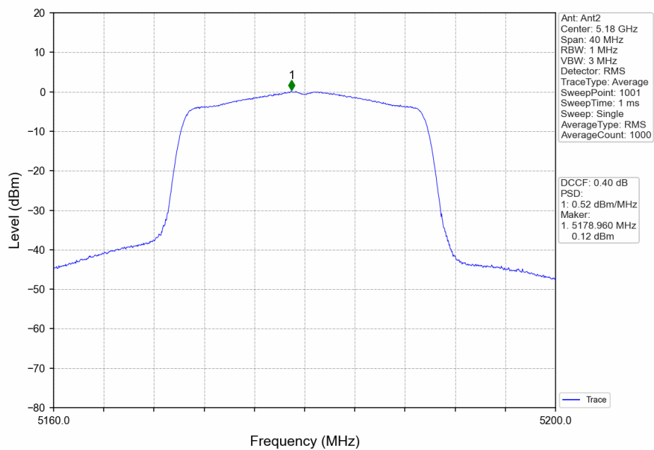
802.11ax(HEW20)_LCH_5180MHz_Ant2_NTNV
