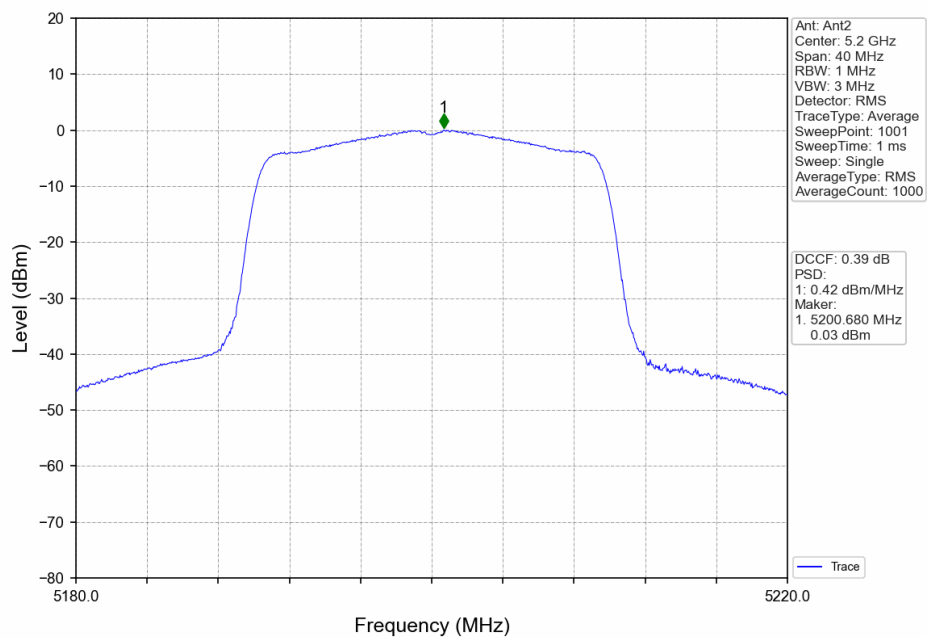
802.11ax(HEW20)_MCH_5200MHz_Ant2_NTNV
