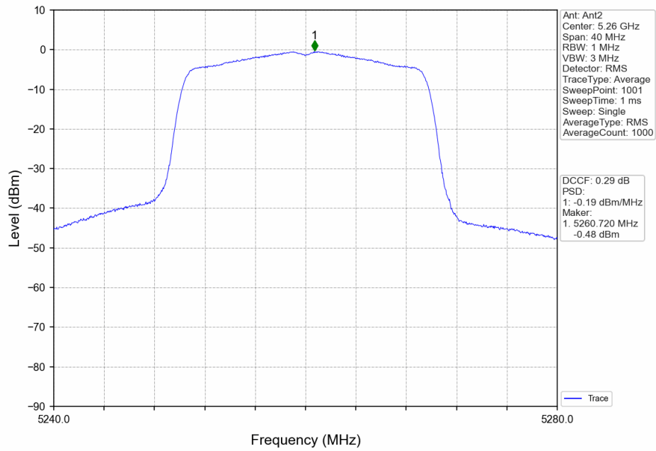
802.11ax(HEW20)_LCH_5260MHz_MIMO_NTNV
