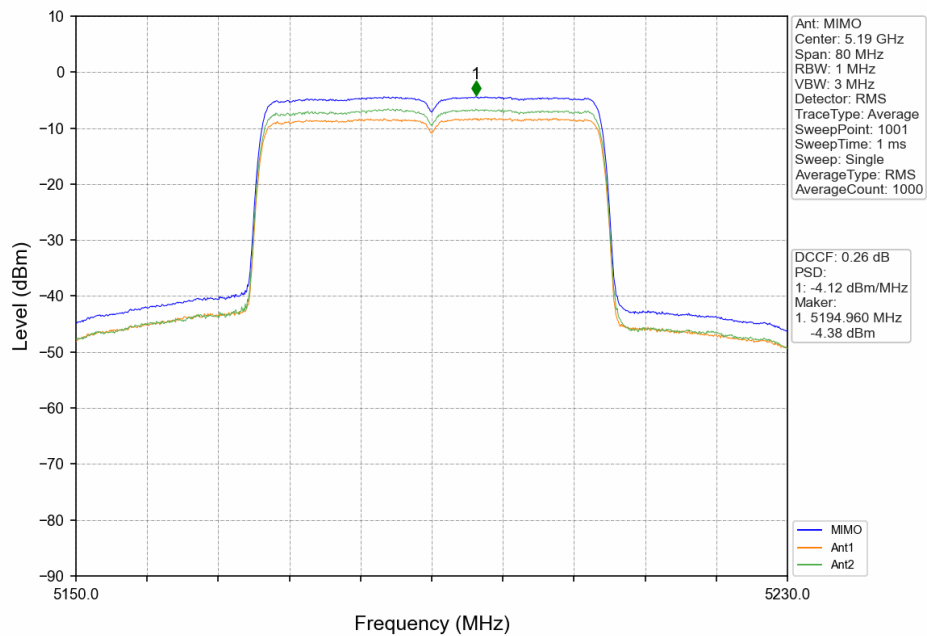
802.11ax(HEW40)_LCH_5190MHz_MIMO_NTNV
