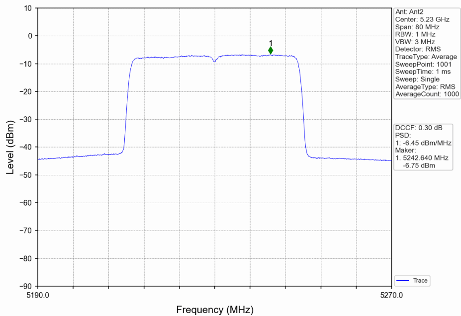
802.11ax(HEW40)_HCH_5230MHz_Ant2_NTNV
