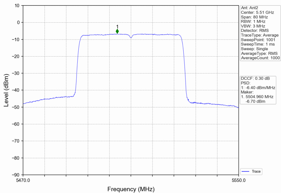
802.11ax(HEW40)_LCH_5510MHz_Ant2_NTNV
