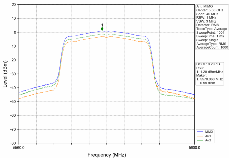
802.11ax(HEW20)_MCH_5580MHz_MIMO_NTNV
