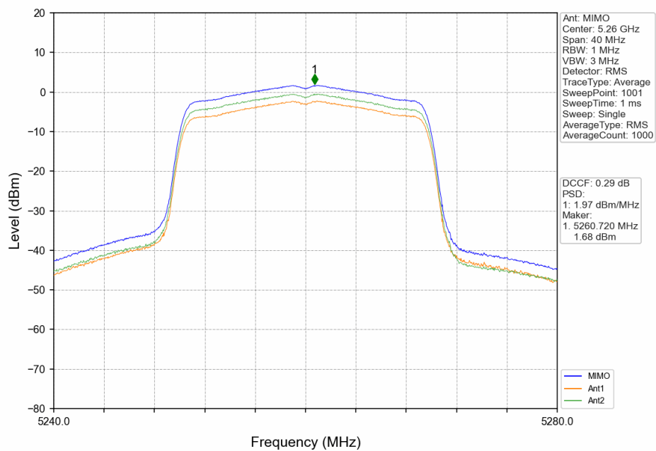
802.11ax(HEW20)_LCH_5260MHz_MIMO_NTNV
