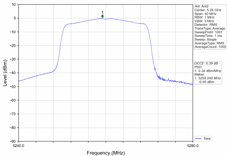
802.11ax(HEW20)_LCH_5260MHz_Ant2_NTNV
