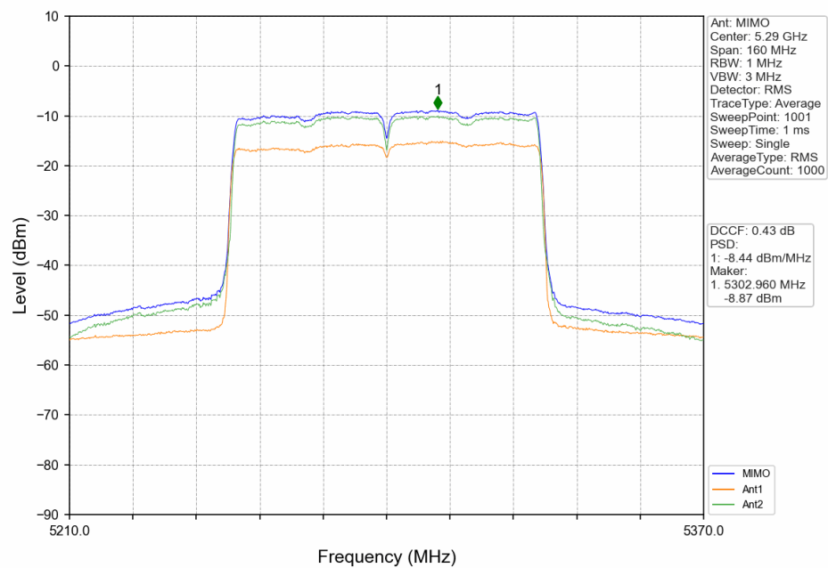
802.11ac(VHT80)_MCH_5290MHz_MIMO_NTNV
