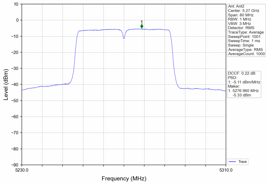
802.11ac(VHT40)_LCH_5270MHz_MIMO_NTNV
