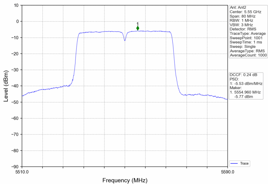
802.11ac(VHT40)_MCH_5550MHz_Ant2_NTNV
