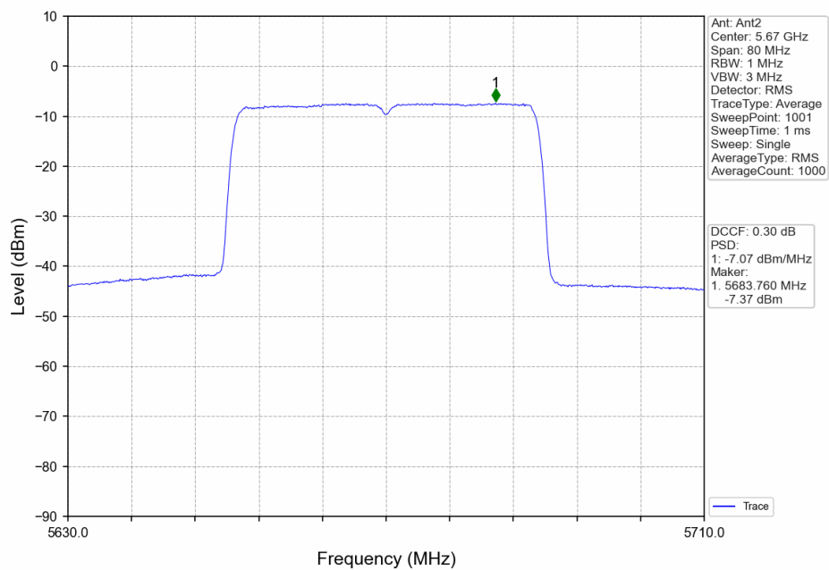
802.11ax(HEW40)_HCH_5670MHz_Ant2_NTNV
