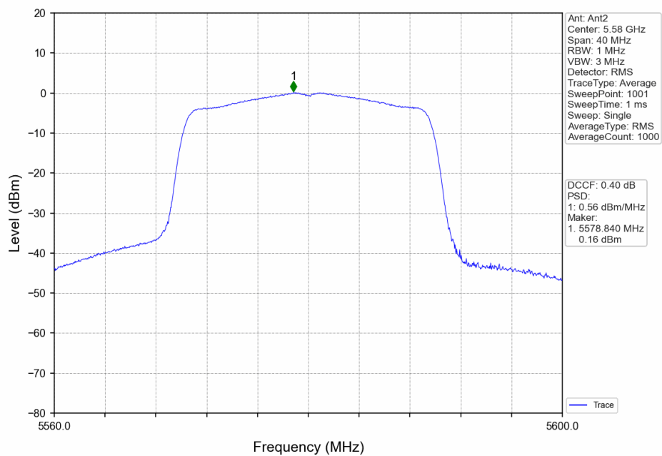
802.11ax(HEW20)_MCH_5580MHz_Ant2_NTNV
