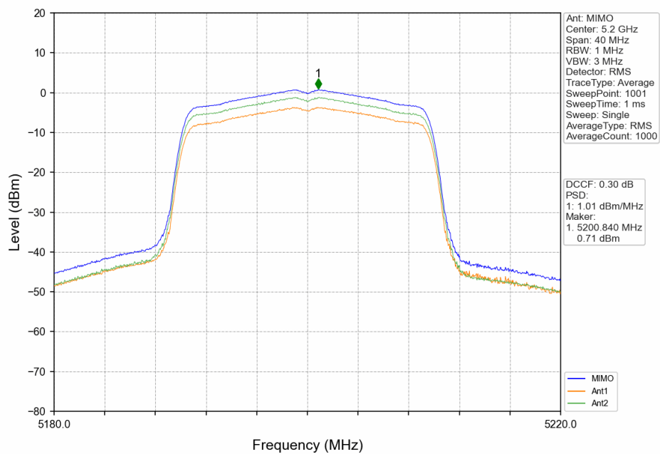
802.11ax(HEW20)_MCH_5200MHz_MIMO_NTNV
