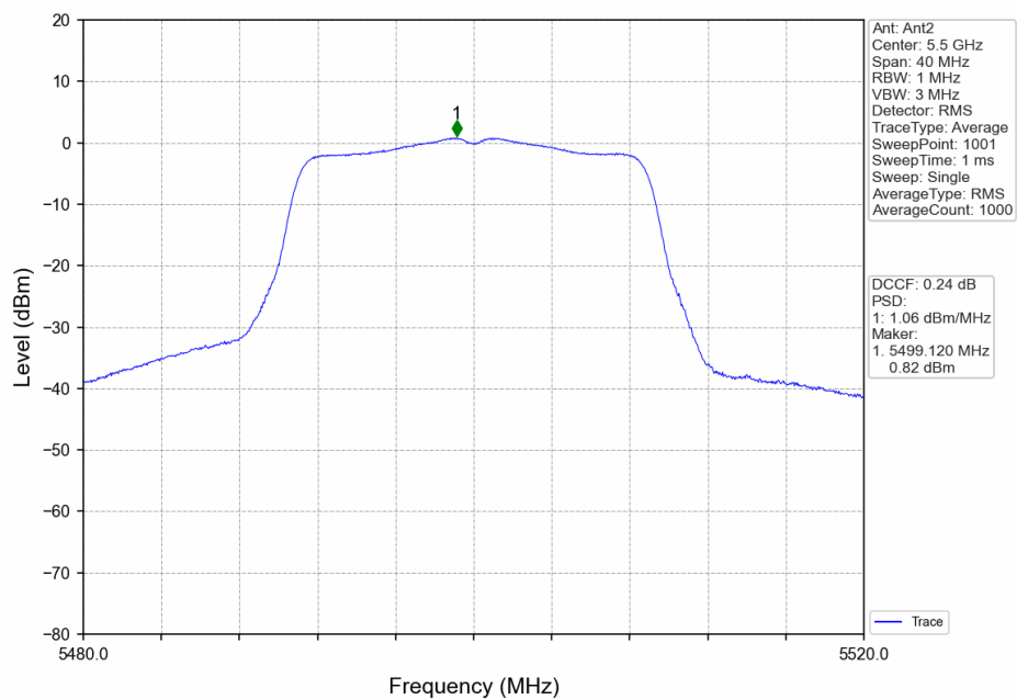
802.11ac(VHT20)_LCH_5500MHz_Ant2_NTNV
