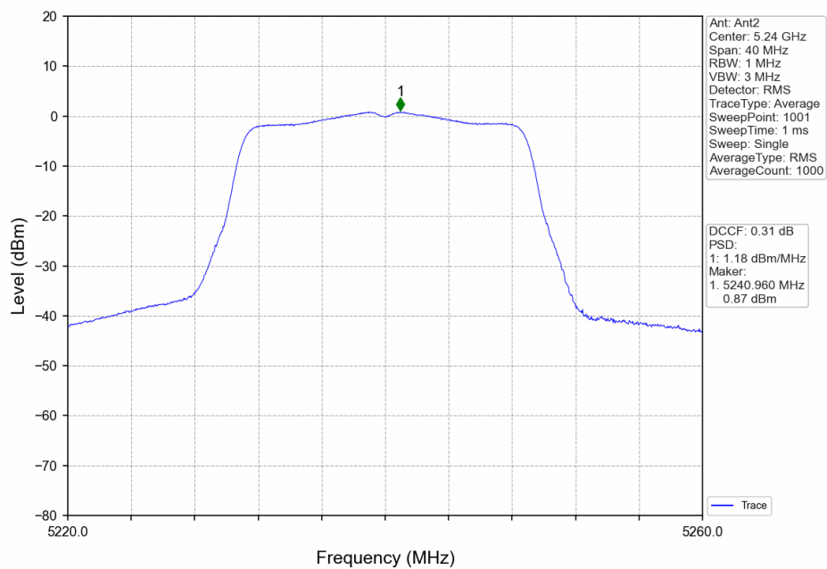
802.11n(HT20)_HCH_5240MHz_Ant2_NTNV
