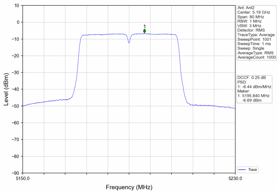
802.11ac(VHT40)_LCH_5190MHz_Ant2_NTNV
