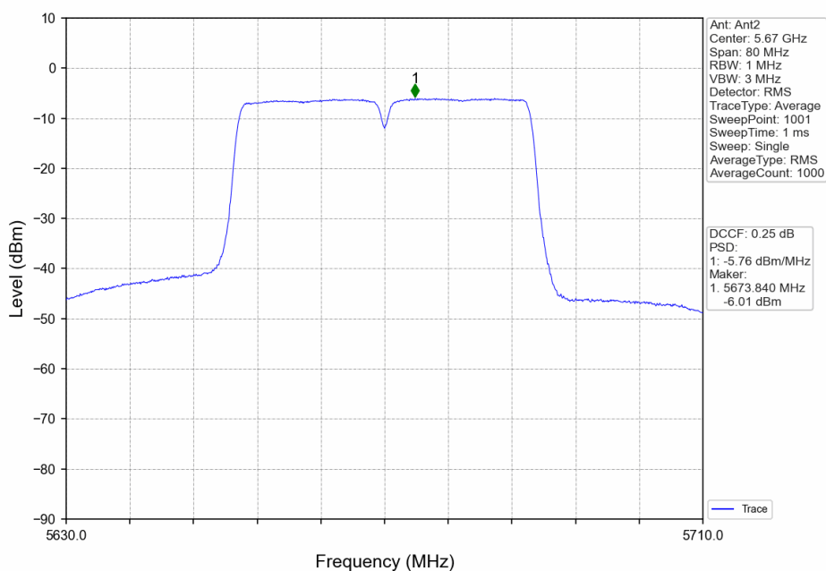
802.11ac(VHT40)_HCH_5670MHz_Ant2_NTNV
