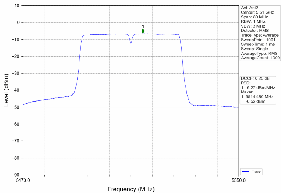
802.11ac(VHT40)_LCH_5510MHz_Ant2_NTNV
