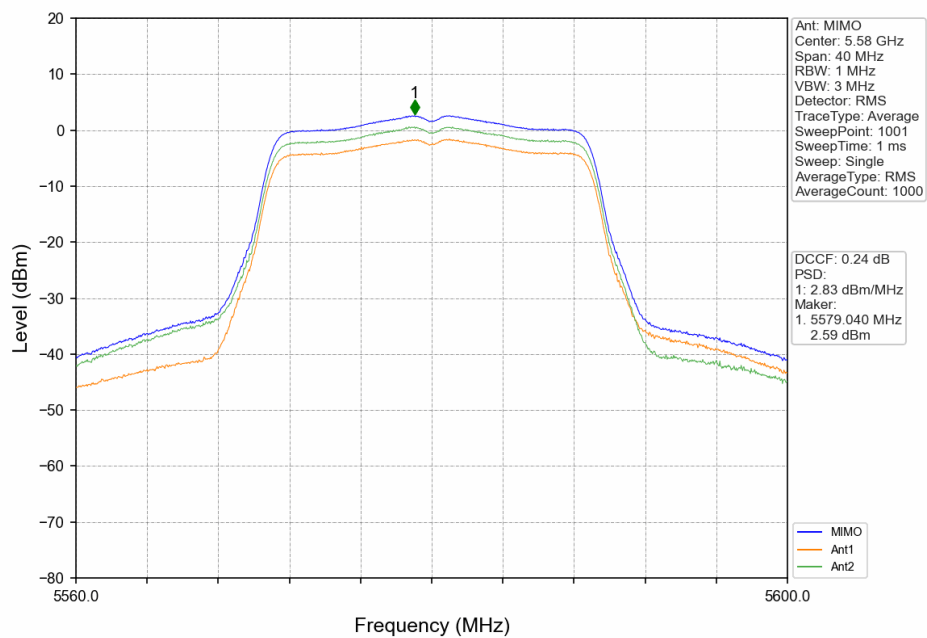
802.11ac(VHT20)_MCH_5580MHz_MIMO_NTNV
