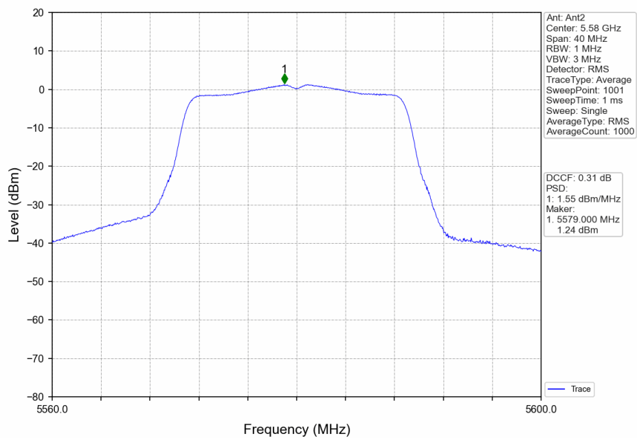
802.11n(HT20)_MCH_5580MHz_Ant2_NTNV
