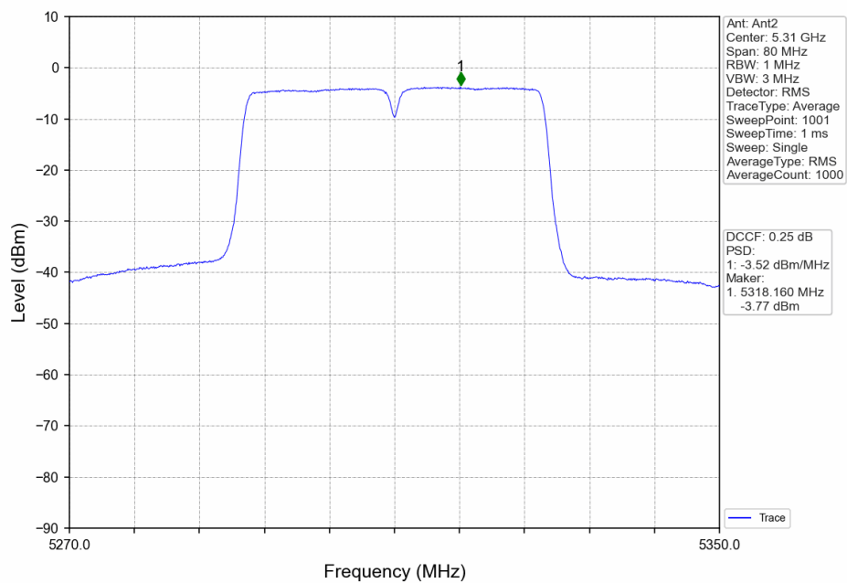
802.11n(HT40)_HCH_5310MHz_Ant2_NTNV
