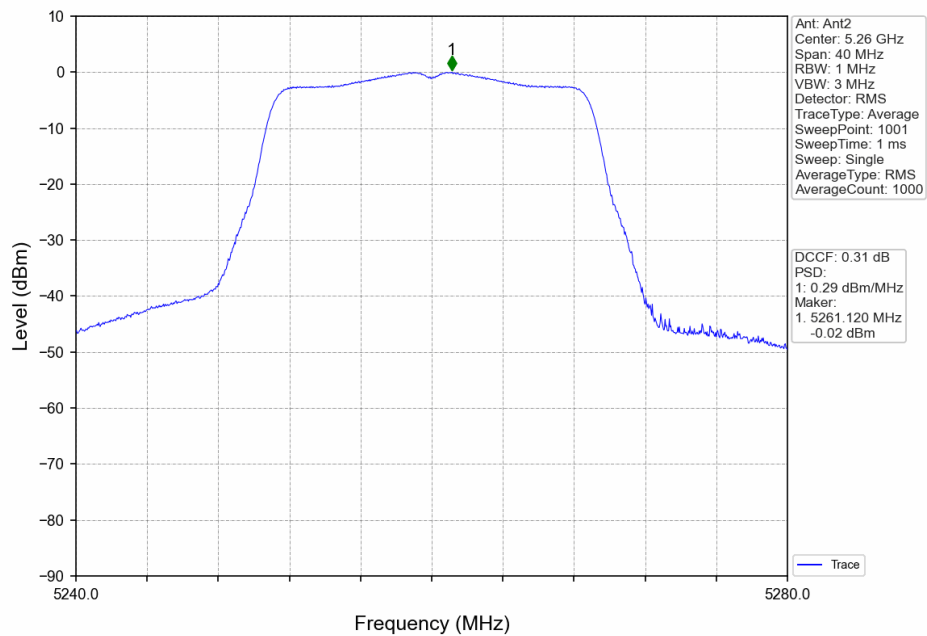
802.11ac(VHT20)_LCH_5260MHz_Ant2_NTNV
