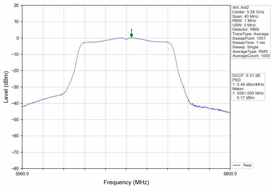
802.11ac(VHT20)_MCH_5580MHz_Ant2_NTNV
