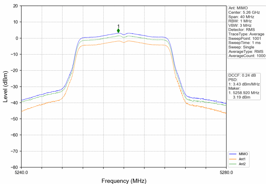
802.11ac(VHT20)_LCH_5260MHz_MIMO_NTNV
