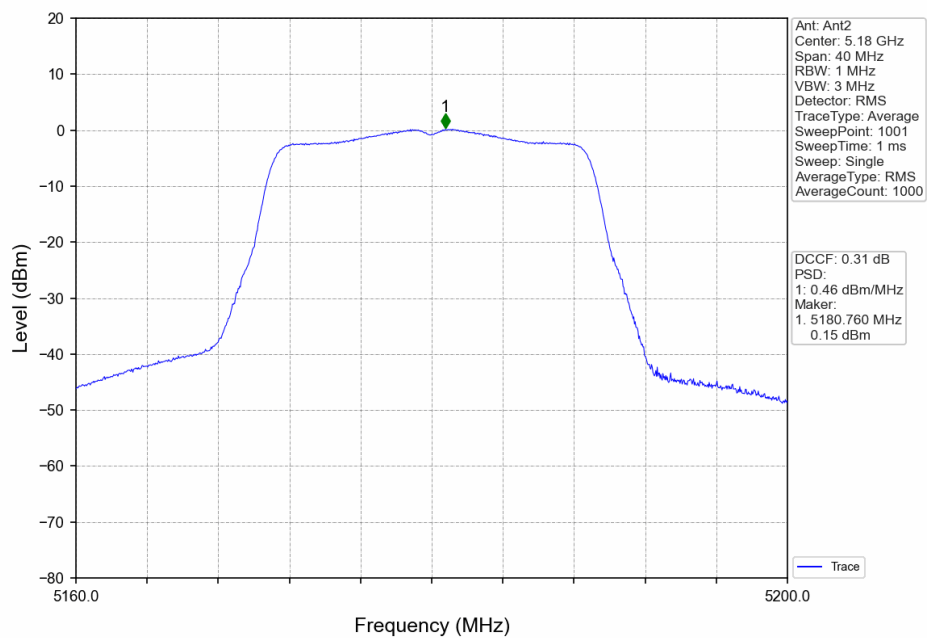
802.11ac(VHT20)_LCH_5180MHz_Ant2_NTNV
