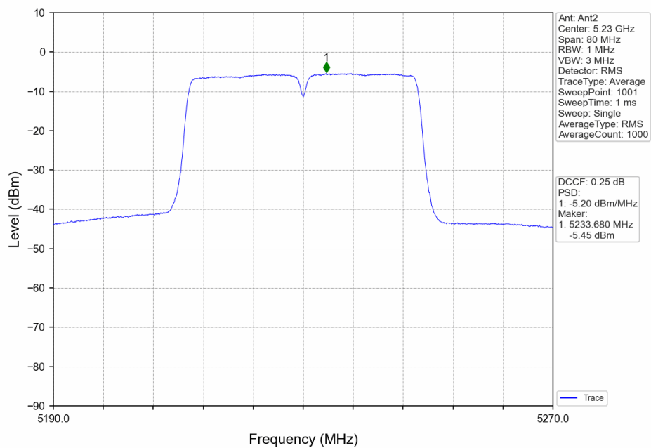
802.11ac(VHT40)_HCH_5230MHz_Ant2_NTNV
