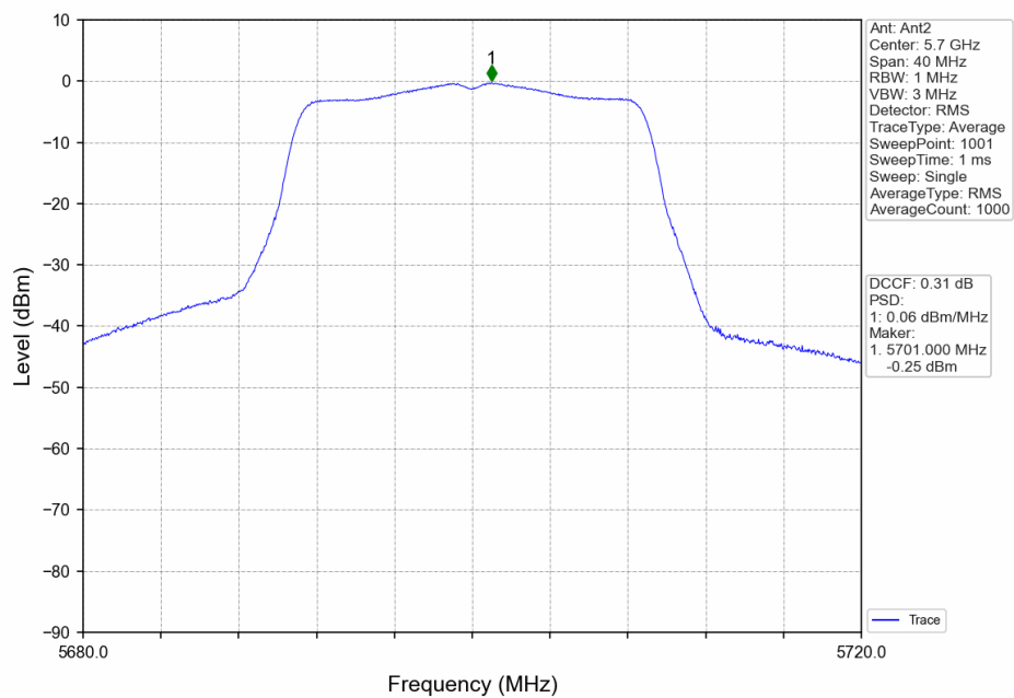
802.11ac(VHT20)_HCH_5700MHz_Ant2_NTNV
