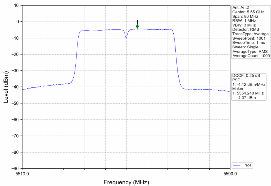
802.11n(HT40)_MCH_5550MHz_Ant2_NTNV
