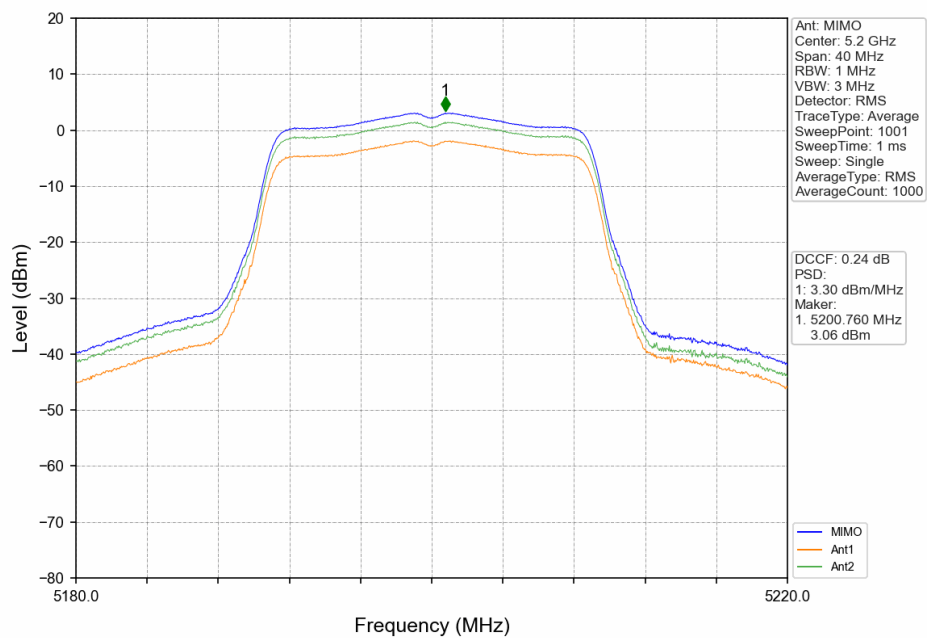
802.11ac(VHT20)_MCH_5200MHz_MIMO_NTNV
