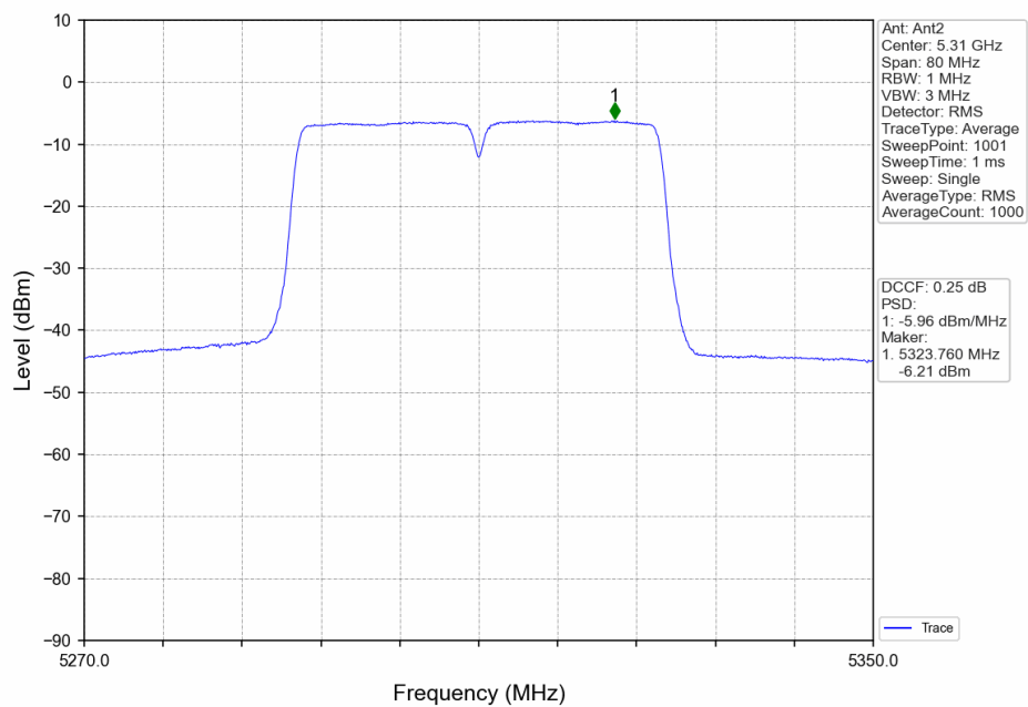
802.11ac(VHT40)_HCH_5310MHz_Ant2_NTNV
