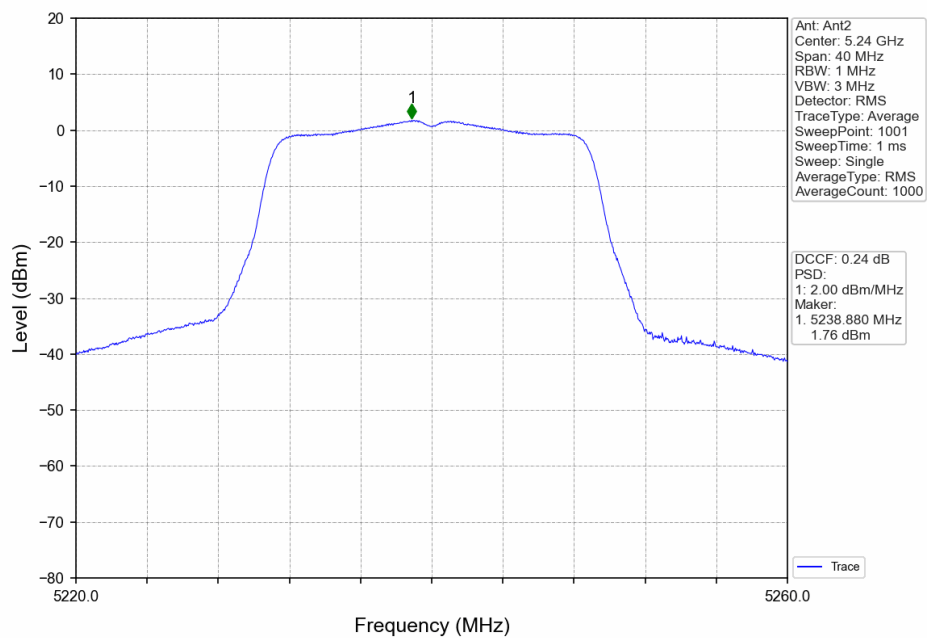
802.11ac(VHT20)_HCH_5240MHz_Ant2_NTNV
