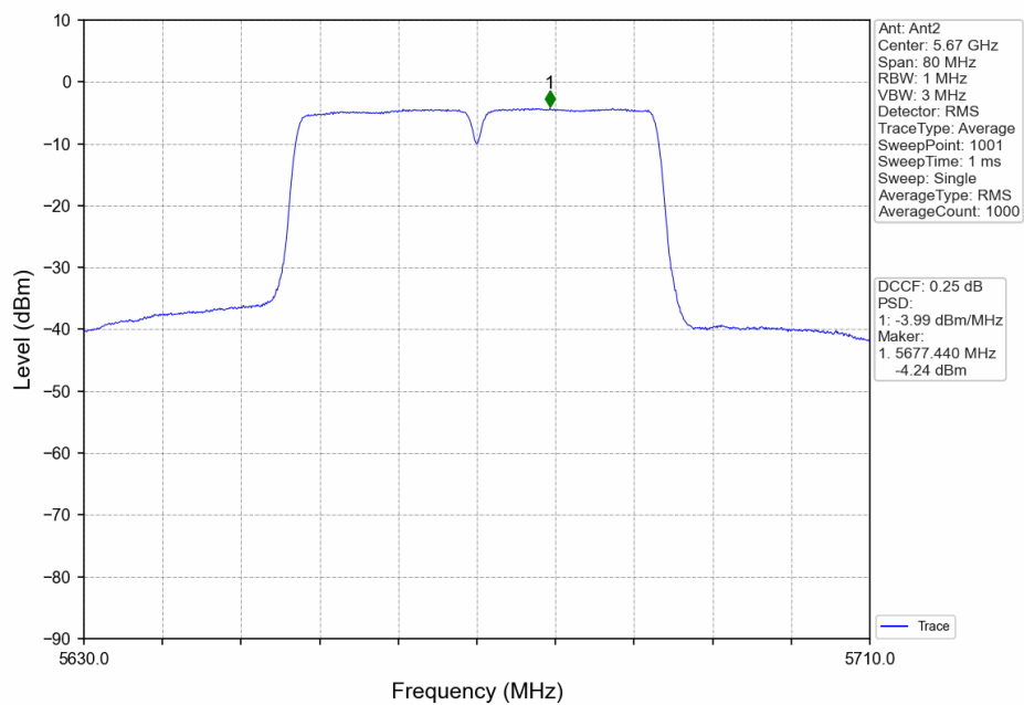
802.11n(HT40)_HCH_5670MHz_Ant2_NTNV
