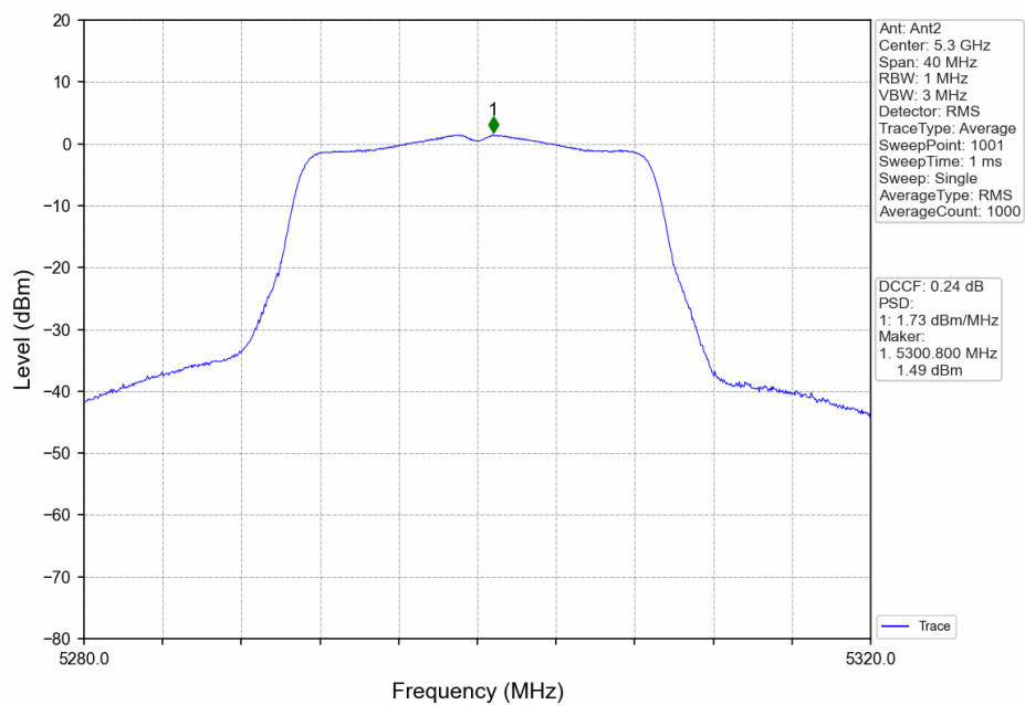
802.11ac(VHT20)_MCH_5300MHz_Ant2_NTNV
