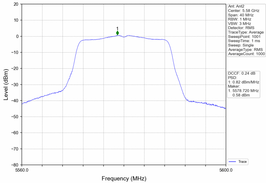
802.11ac(VHT20)_MCH_5580MHz_MIMO_NTNV
