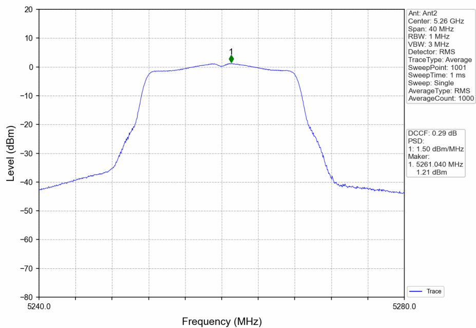
802.11a_LCH_5260MHz_Ant2_NTNV
