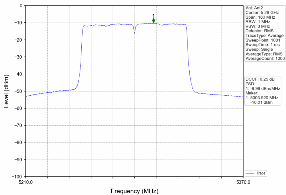
802.11ac(VHT80)_MCH_5290MHz_Ant2_NTNV
