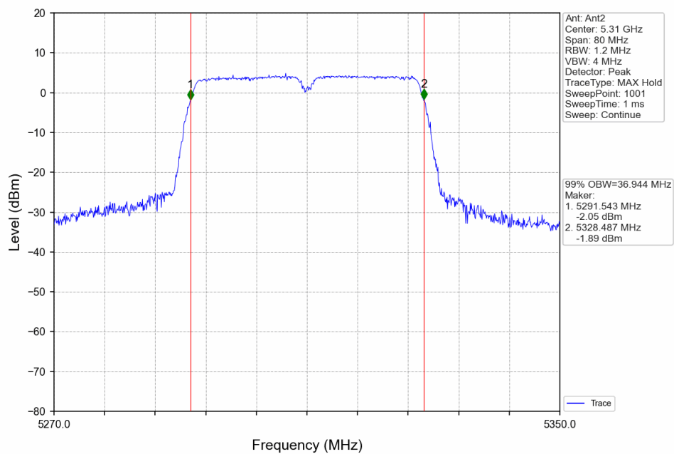
802.11ac(VHT40)_HCH_5310MHz_Ant2_NTNV
