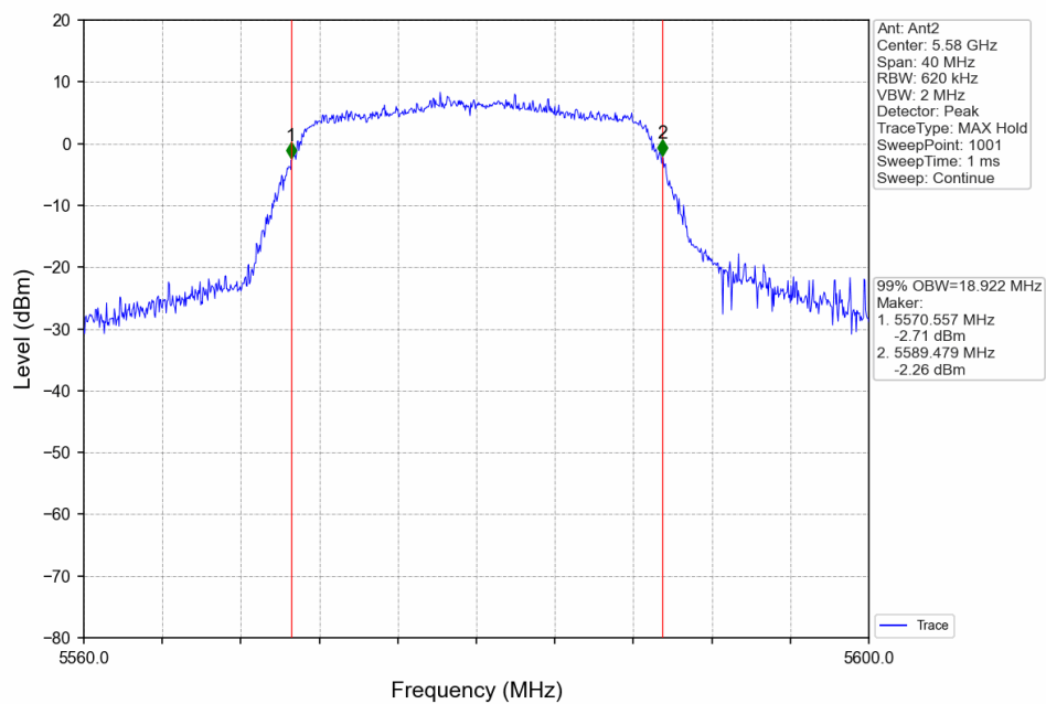
802.11n(HT20)_MCH_5580MHz_Ant2_NTNV
