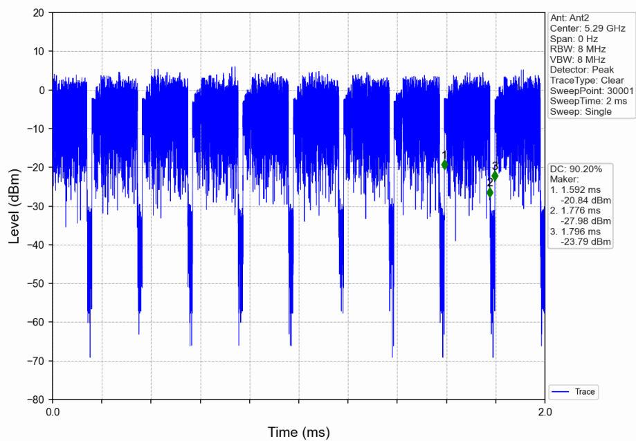
802.11ax(HEW80)_MCH_5290MHz_Ant2_NTNV_MIMO
