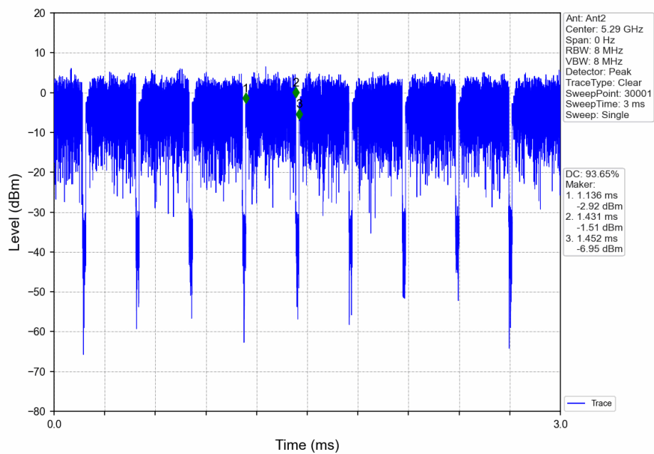
802.11ax(HEW80)_MCH_5290MHz_Ant2_NTNV
