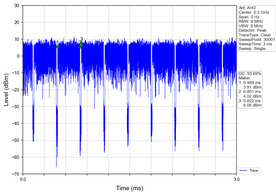
802.11ax(HEW20)_LCH_5500MHz_Ant2_NTNV_MIMO
