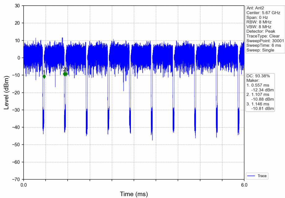
802.11ax(HEW40)_HCH_5670MHz_Ant2_NTNV
