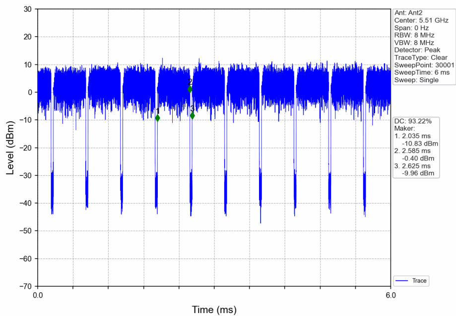
802.11ax(HEW40)_LCH_5510MHz_Ant2_NTNV
