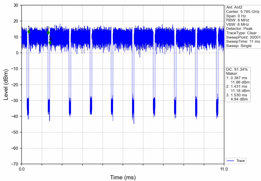
802.11ax(HEW20)_MCH_5785MHz_Ant2_NTNV
