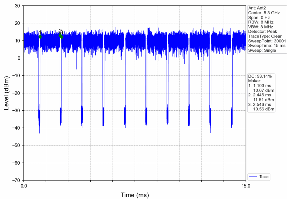
802.11ac(VHT20)_MCH_5300MHz_Ant2_NTNV
