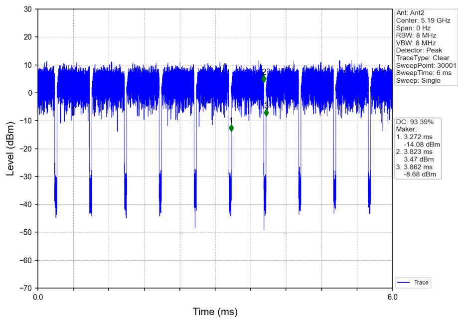
802.11ax(HEW40)_LCH_5190MHz_Ant2_NTNV
