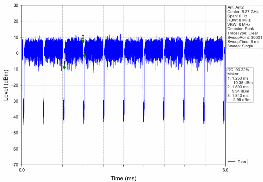
802.11ax(HEW40)_LCH_5270MHz_Ant2_NTNV
