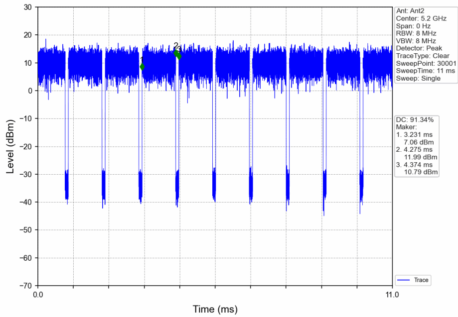
802.11ax(HEW20)_HCH_5240MHz_Ant2_NTNV
