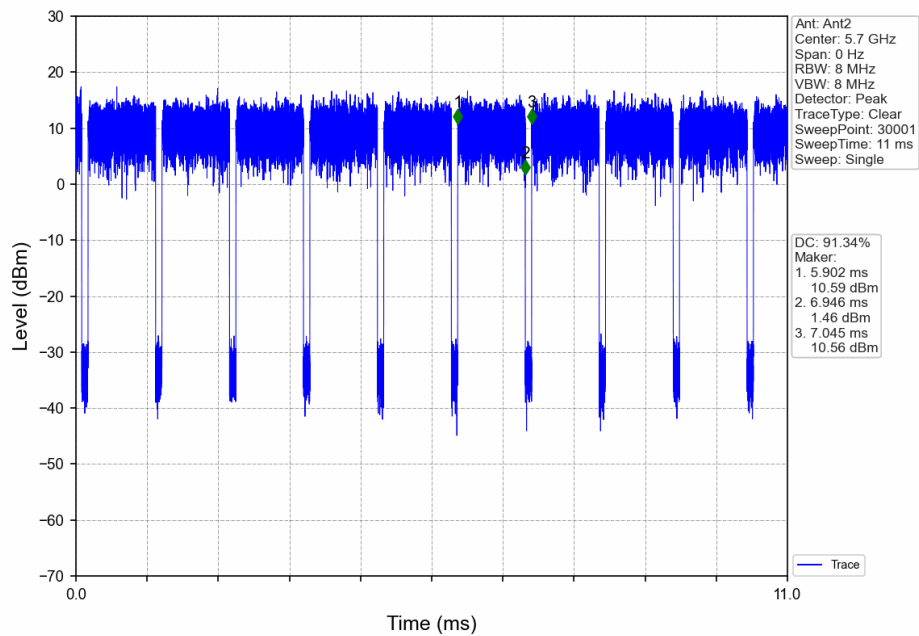
802.11ax(HEW20)_HCH_5700MHz_Ant2_NTNV
