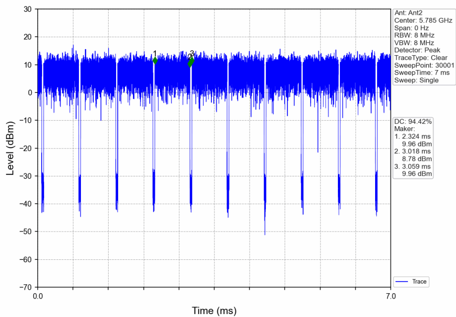
802.11ac(VHT20)_MCH_5785MHz_Ant2_NTNV_MIMO
