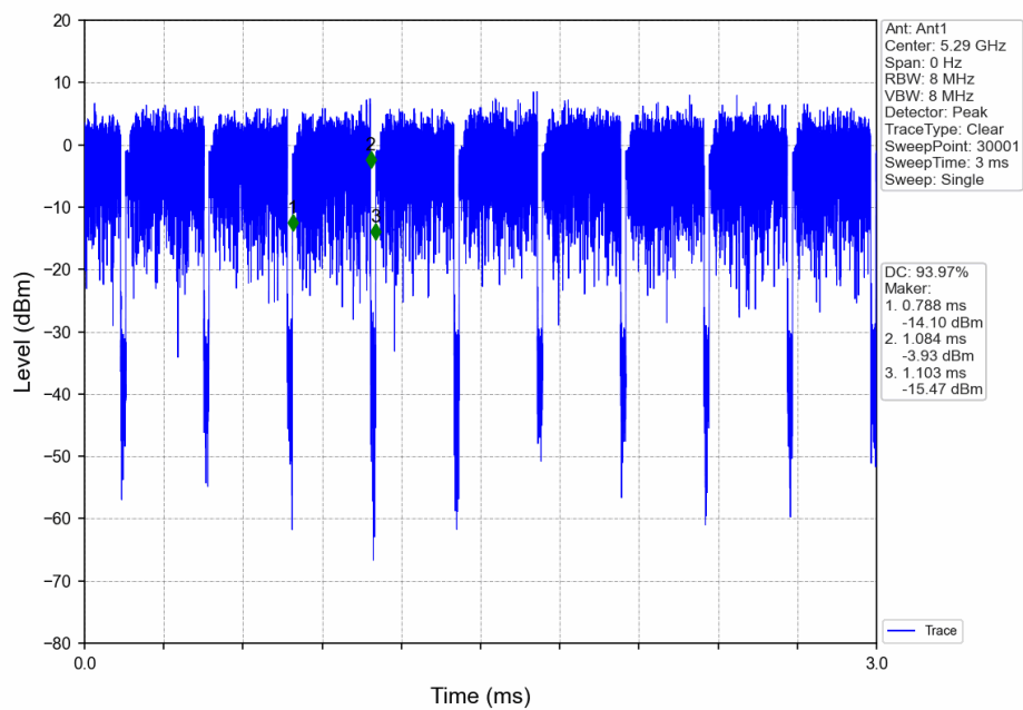
802.11ax(HEW80)_MCH_5290MHz_Ant1_NTNV
