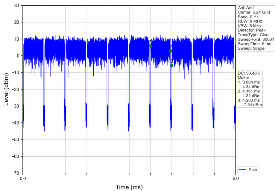
802.11ax(HEW20)_HCH_5240MHz_Ant1_NTNV_MIMO
