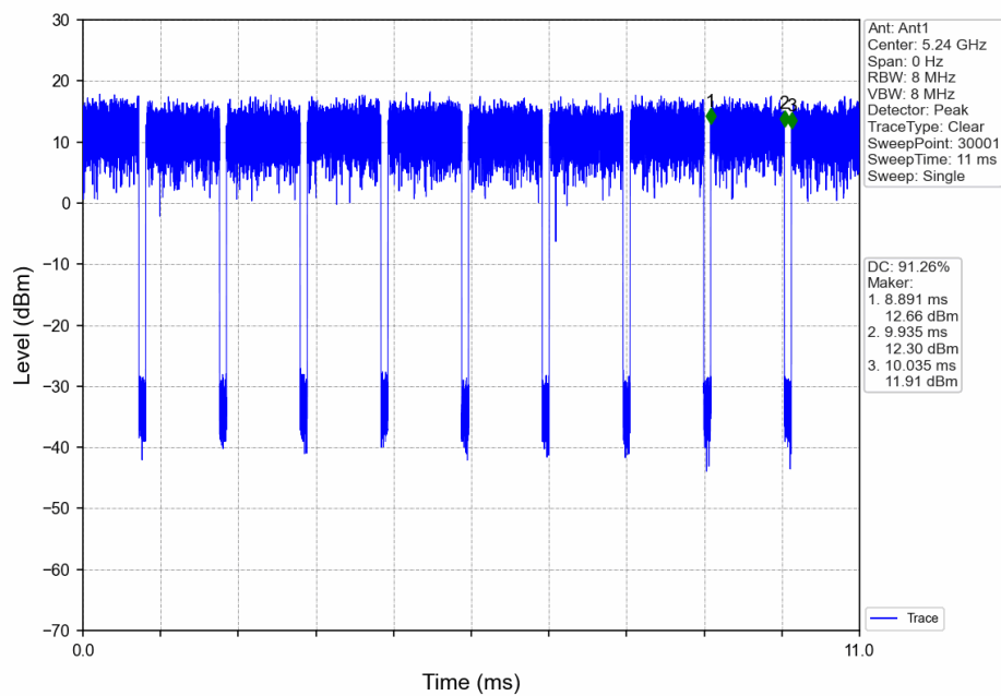
802.11ax(HEW20)_HCH_5240MHz_Ant1_NTNV
