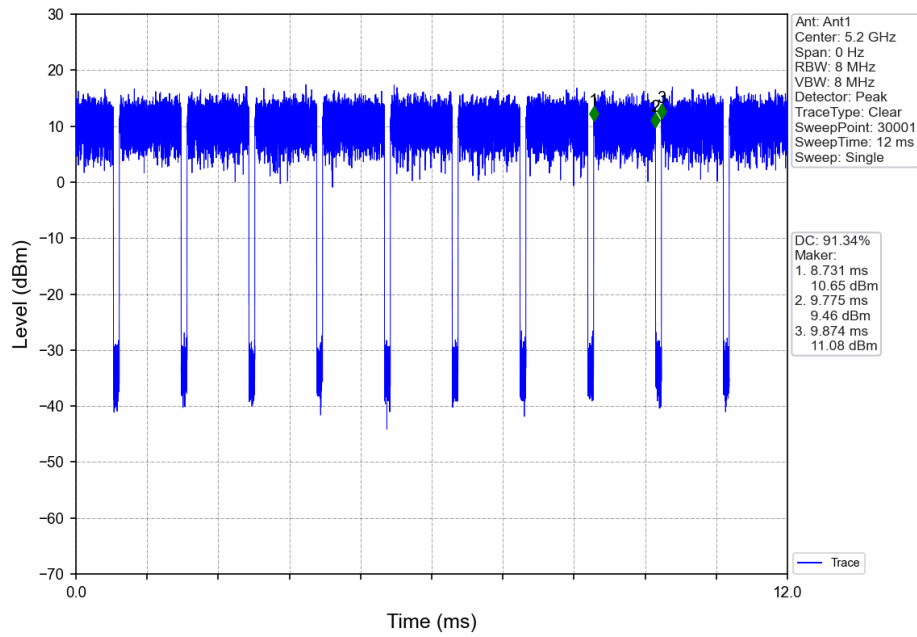
802.11ax(HEW20)_HCH_5240MHz_Ant1_NTNV
