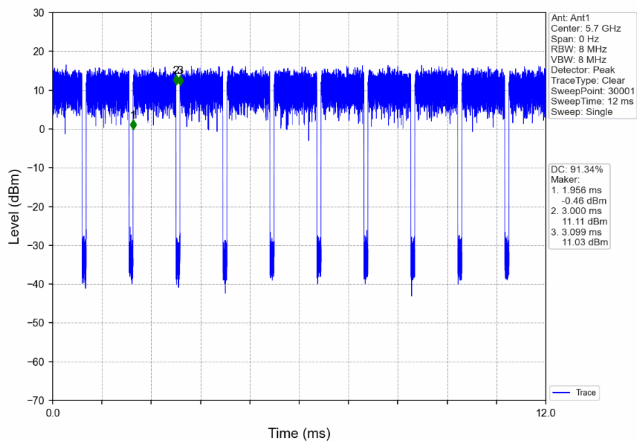
802.11ax(HEW20)_HCH_5700MHz_Ant1_NTNV
