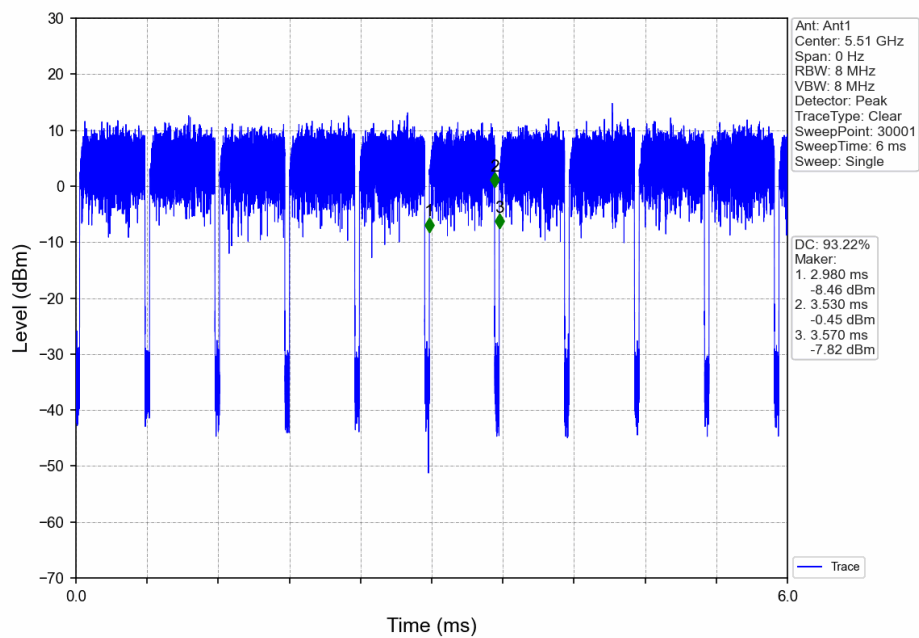
802.11ax(HEW40)_LCH_5510MHz_Ant1_NTNV
