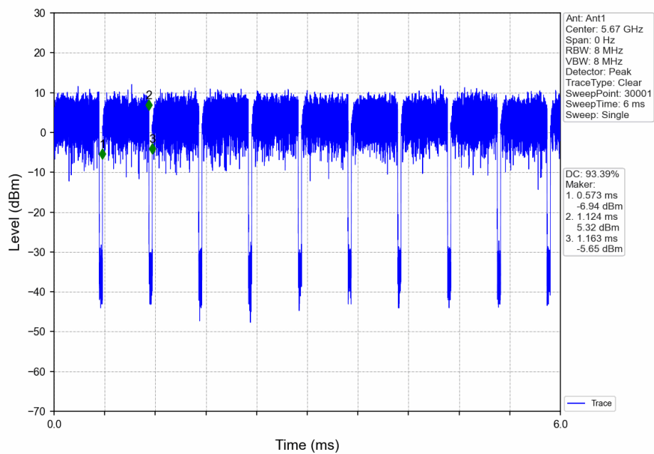
802.11ax(HEW40)_HCH_5670MHz_Ant1_NTNV
