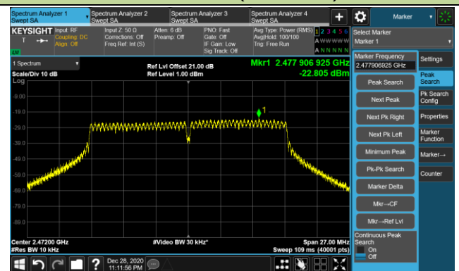
Channel 13 (2472MHz)
