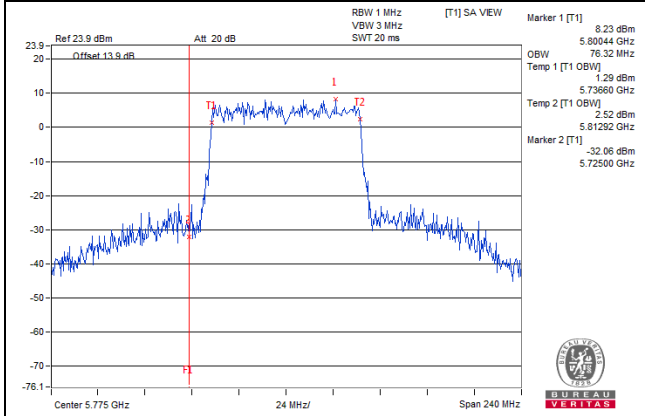
802.11ac(VHT80)_Chain0 / CH155
