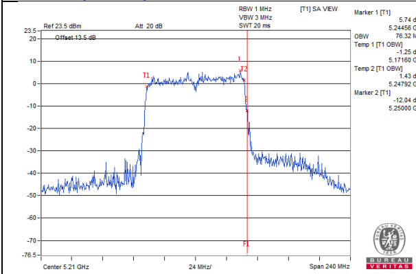
802.11ac(VHT80)_Chain0 / CH42
