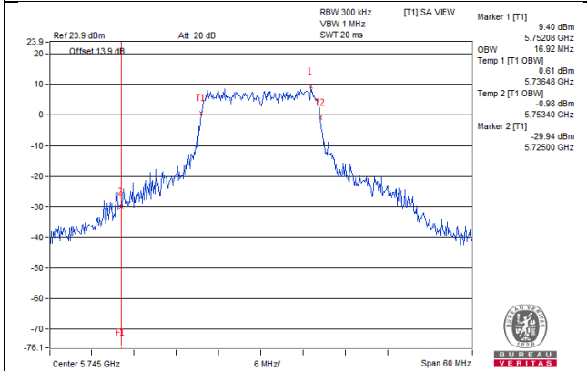
802.11ac(VHT20)_Chain0 / CH149
