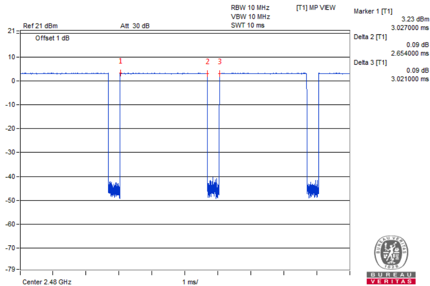
Time-domain plot for Zigbee transmission signal
