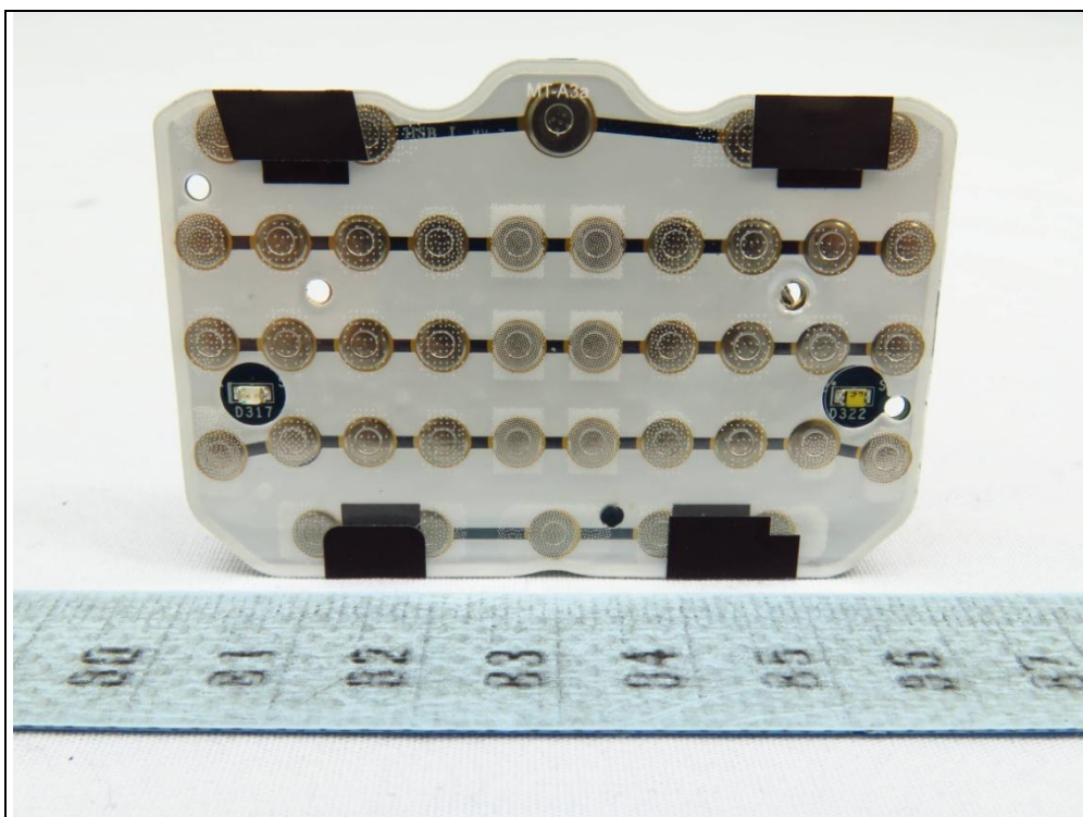
Sample B: Short K/B-Qwety + Scanner (EX20)
