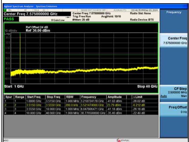
CSE_5G_n77(K)_30KHz_.PI2-BPSK_30M CH635666_1RB@1_
