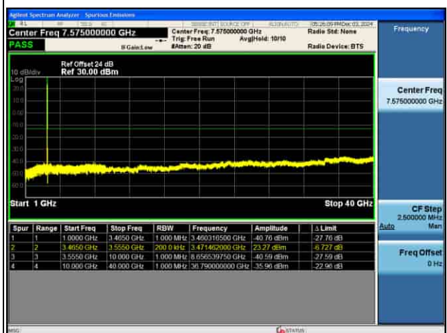
CSE_5G_n77(K)_30KHz_.PI2-BPSK_80M CH634000_1RB@1_
