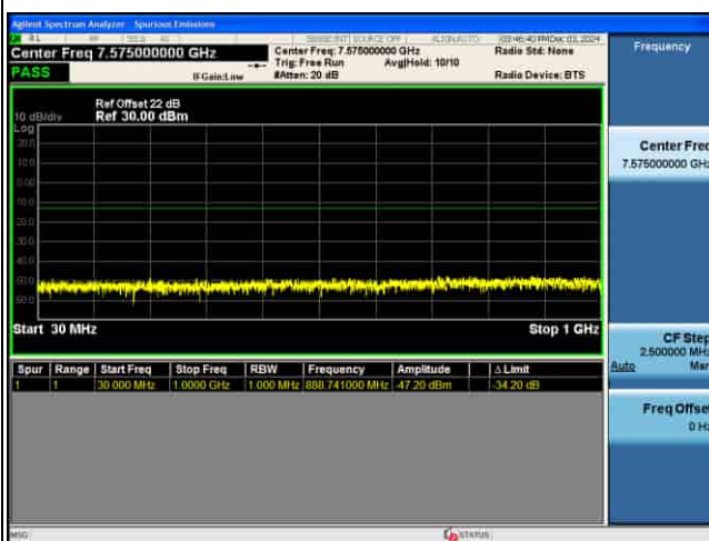
CSE_5G_n77(K)_30KHz_.PI2-BPSK_30M CH635666_1RB@1
