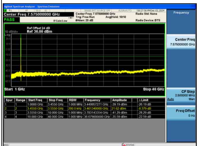
CSE_5G_n77(K)_30KHz_.PI2-BPSK_90M CH633666_1RB@1_
