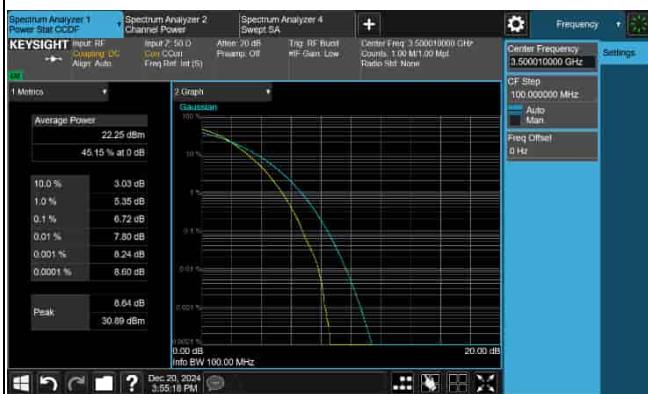
PAPR_5G_n77_30KHz_30M_3500.01MHz-256QAM
