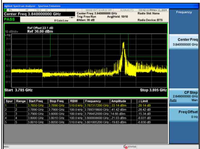
EDGE_4G_B43_QPSK_10M_FULL RB@0_CH45540
