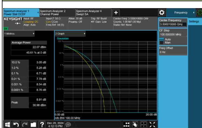
PAPR_5G_n77_30KHz_60M_3500.01MHz-256QAM
