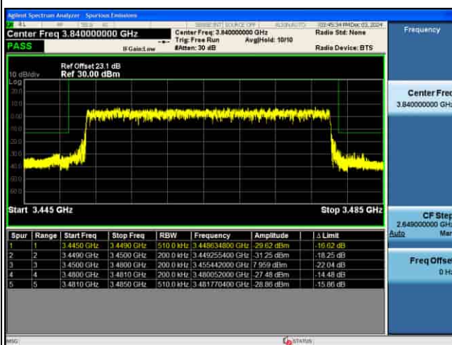
EDGE_5G_n77(K)_30KHz_P12-BPSK_30M_FULL RB@MAX_CH631000
