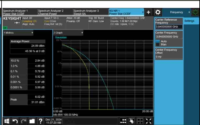
PAPR_5G_n77_30KHz_20M_3840MHz-64QAM
