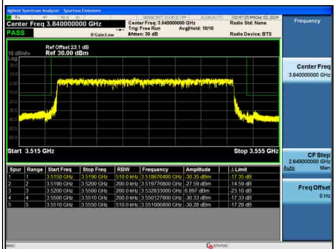
EDGE_5G_n77(K)_30KHz_P12-BPSK_30M_FULL RB@MAX_CH635666
