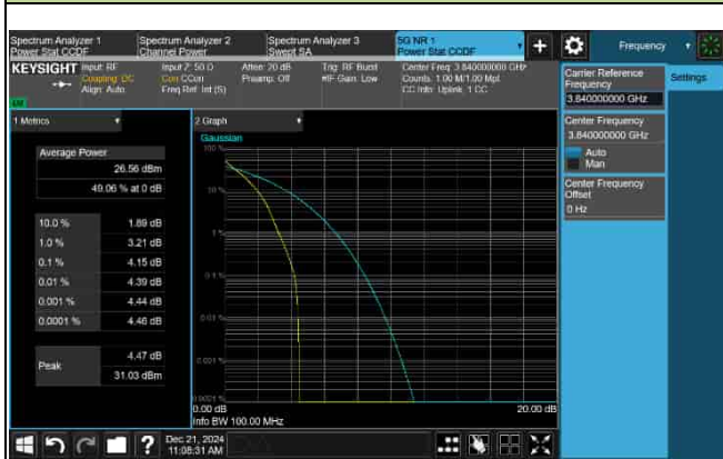
PAPR_5G_n77_30KHz_15M_3840MHz-16QAM
