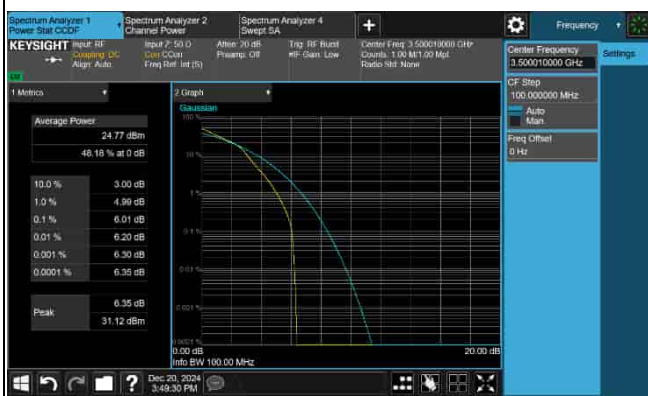
PAPR_5G_n77_30KHz_20M_3500.01MHz-256QAM
