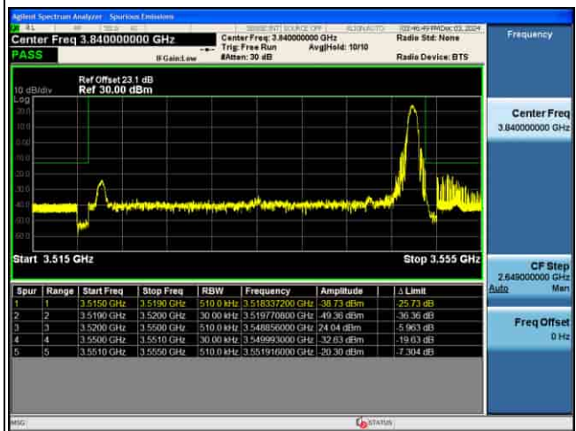
EDGE_5G_n77(K)_30KHz_P12-BPSK_30M_FULL RB@0_CH635666
