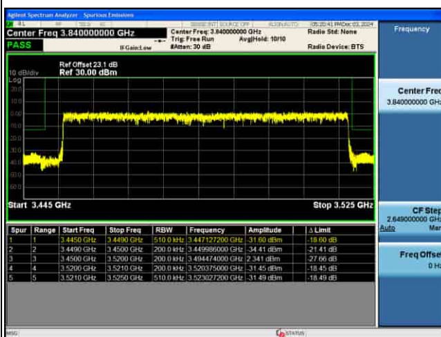
EDGE_5G_n77(K)_30KHz_P12-BPSK_70M_FULL RB@MAX_CH632334
