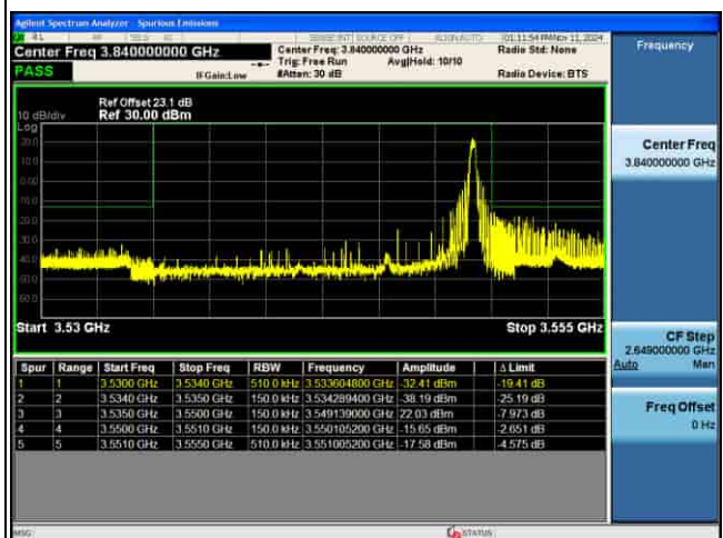
EDGE_4G_B42_QPSK_15M_FULL RB@0_CH43015
