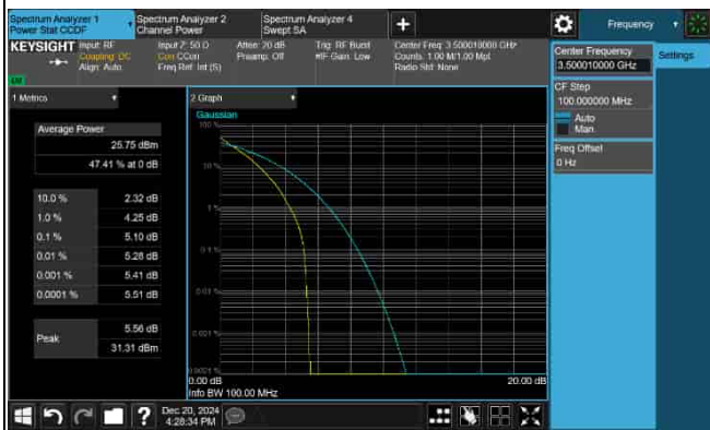
PAPR_5G_n77_30KHz_90M_3500.01MHz-16QAM
