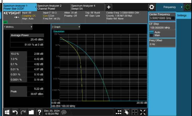
PAPR_5G_n77_30KHz_70M_3500.01MHz-64QAM
