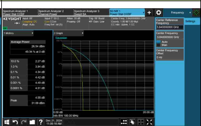
PAPR_5G_n77_30KHz_15M_3840MHz-64QAM
