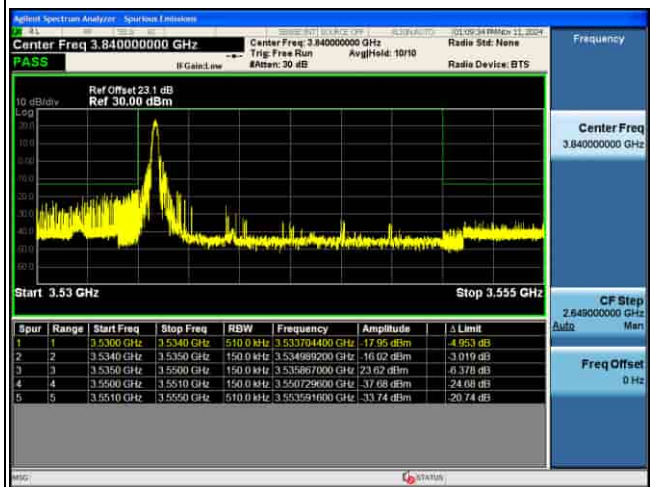
EDGE_4G_B42_QPSK_15M_1RB@MAX_CH43015
