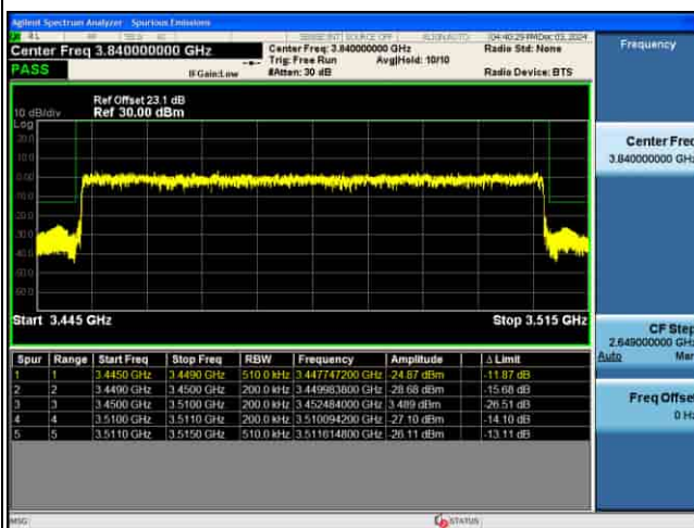
EDGE_5G_n77(K)_30KHz_P12-BPSK_70M_1RB@0_CH632334
