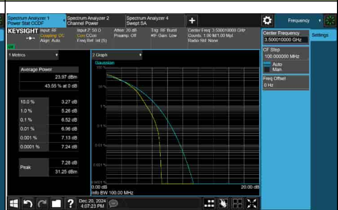
PAPR_5G_n77_30KHz_50M_3500.01MHz-64QAM
