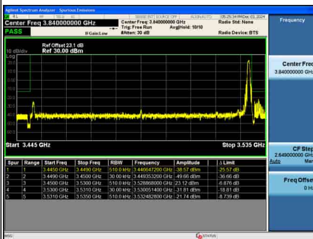
EDGE_5G_n77(K)_30KHz_P12-BPSK_80M_FULL RB@0_CH632668
