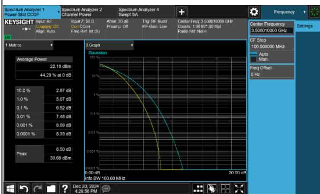
PAPR_5G_n77_30KHz_90M_3500.01MHz-256QAM
