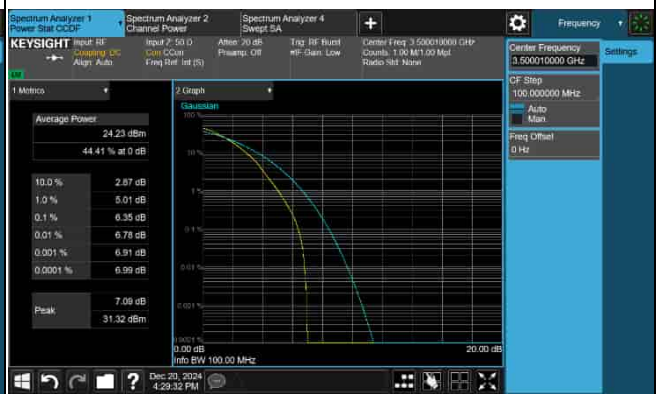
PAPR_5G_n77_30KHz_90M_3500.01MHz-64QAM
