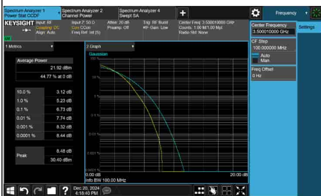
PAPR_5G_n77_30KHz_70M_3500.01MHz-256QAM
