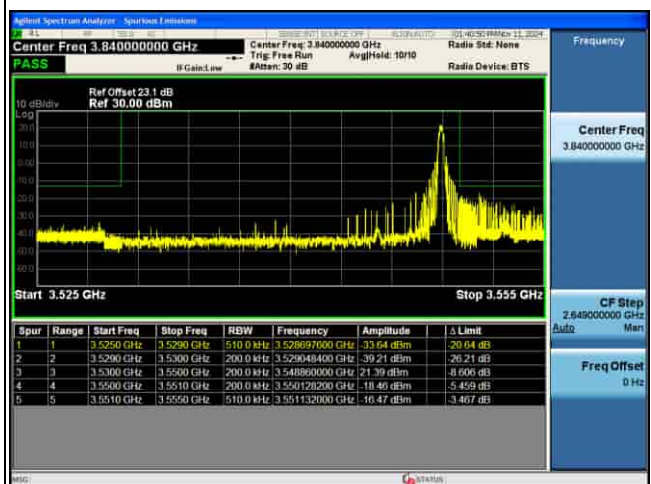
EDGE_4G_B42_QPSK_20M_FULL RB@0_CH42990
