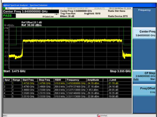
EDGE_5G_n77(K)_30KHz_P12-BPSK_70M_FULL RB@MAX_CH634332
