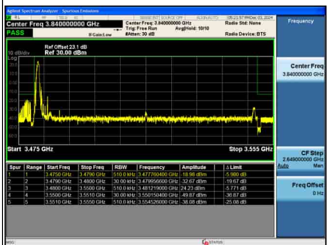
EDGE_5G_n77(K)_30KHz_P12-BPSK_70M_1RB@0_CH634332
