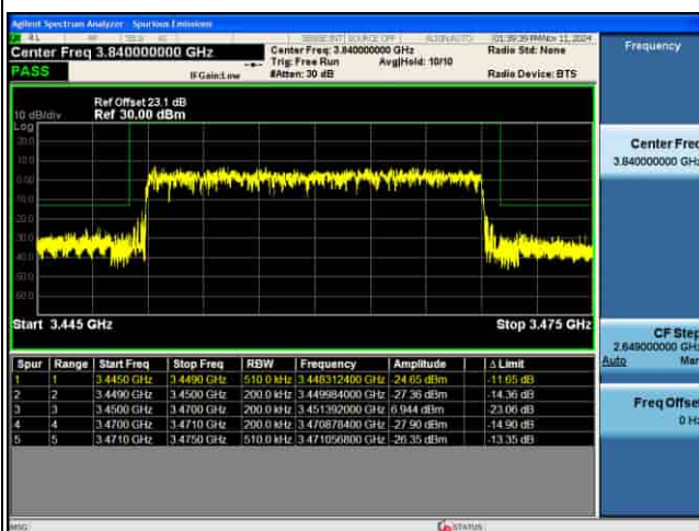
EDGE_4G_B42_QPSK_20M_FULL RB@0_CH42190
