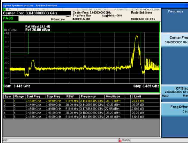
EDGE_5G_n77(K)_30KHz_P12-BPSK_30M_FULL RB@0_CH631000
