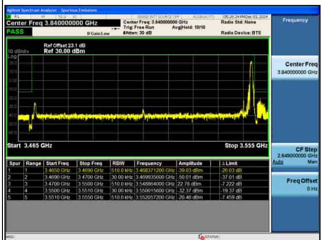
EDGE_5G_n77(K)_30KHz_P12-BPSK_80M_FULL RB@0_CH634000
