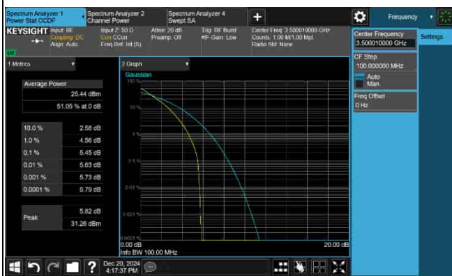
PAPR_5G_n77_30KHz_70M_3500.01MHz-16QAM
