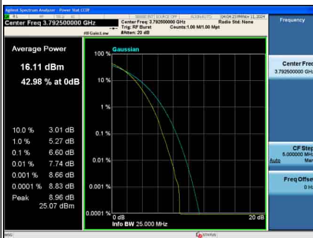
PTAR_4G_B43_256QAM_15M CH45515
