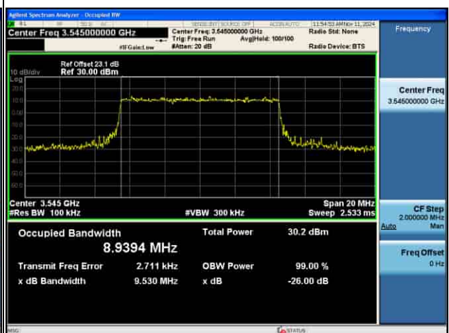
OCC_4G_B42_.QPSK_10M CH43040
