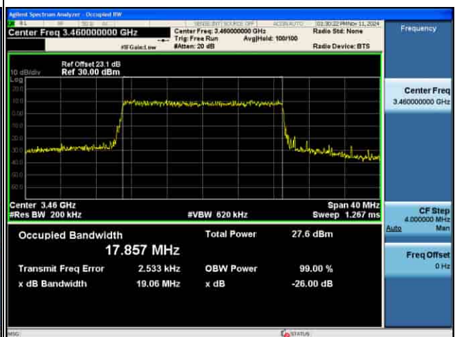
OCC_4G_B42_64QAM_20M CH42990
