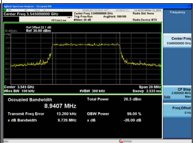
OCC_4G_B42_256QAM_10M CH43040
