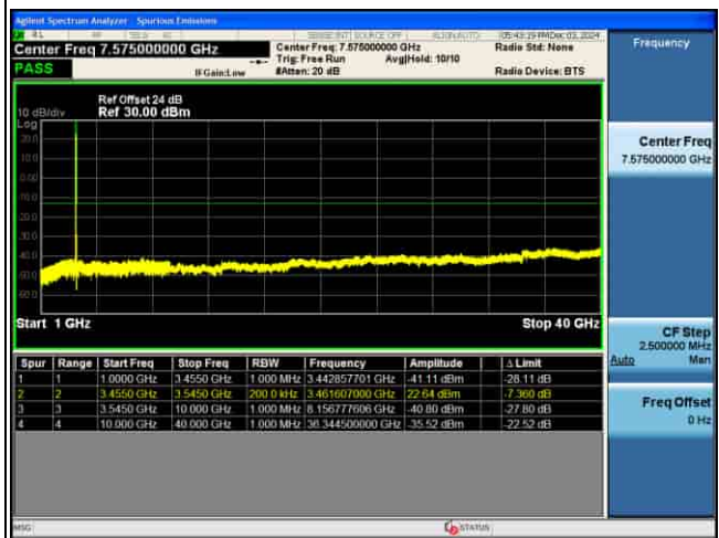
CSE_5G_n77(K)_30KHz_16QAM_80M CH634000_1RB@1_
