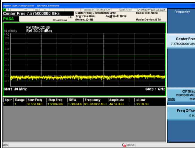
CSE_5G_n77(K)_30KHz_16QAM_60M CH634666_1RB@1
