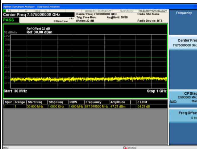
CSE_5G_n77(K)_30KHz_16QAM_90M CH633000_1RB@1
