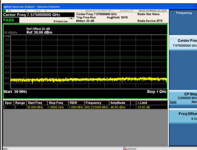
CSE_5G_n77(K)_30KHz_256QAM_60M CH633334_1RB@1_
