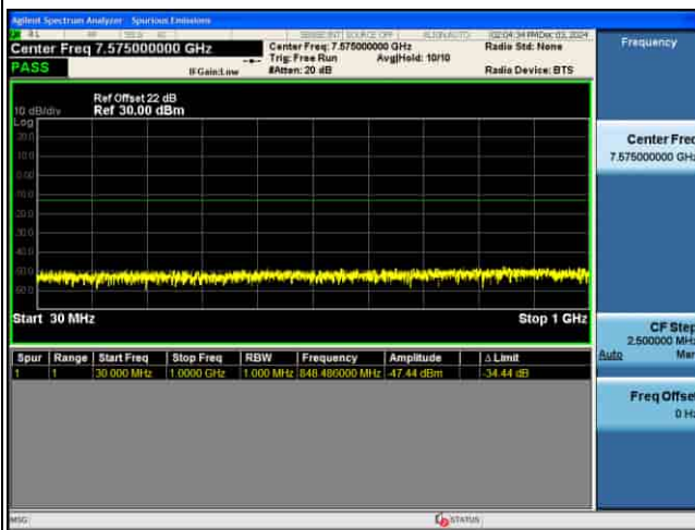
CSE_5G_n77(K)_30KHz_16QAM_15M CH636166_1RB@1
