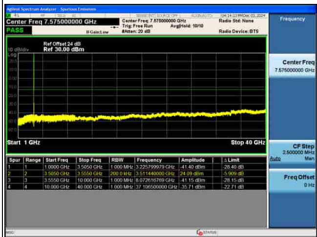
CSE_5G_n77(K)_30KHz_256QAM_50M CH631668_1RB@1_
