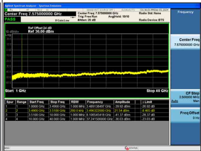
CSE_5G_n77(K)_30KHz_16QAM_10M CH636332_1RB@1_
