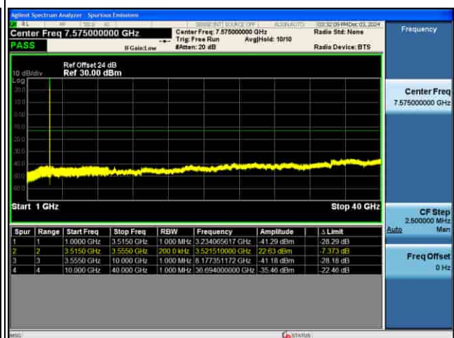
CSE_5G_n77(K)_30KHz_64QAM_30M CH635666_1RB@1_
