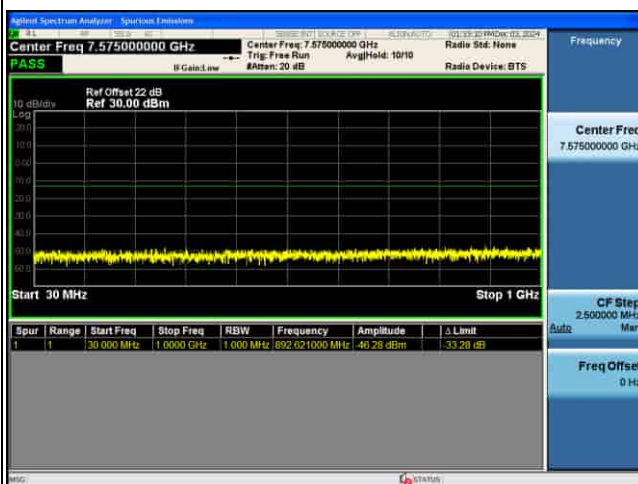
CSE_5G_n77(K)_30KHz_16QAM_15M CH630500_1RB@1
