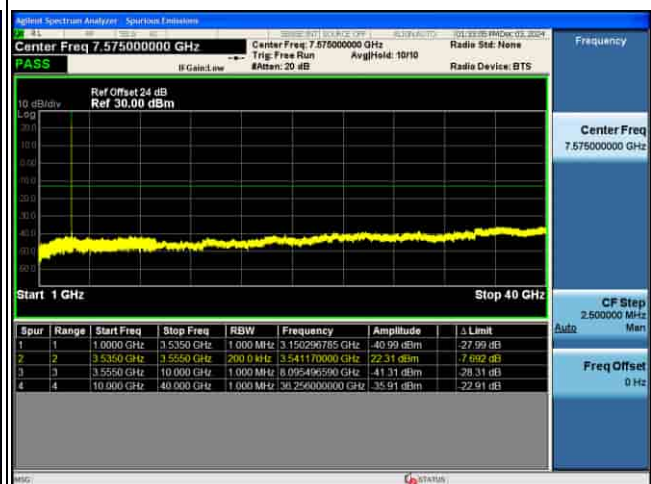
CSE_5G_n77(K)_30KHz_16QAM_15M CH630500_1RB@1_
