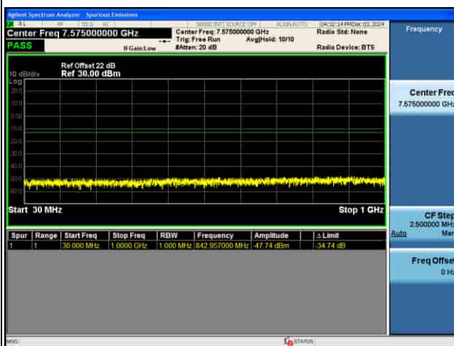
CSE_5G_n77(K)_30KHz_QPSK_50M CH633334_1RB@1
