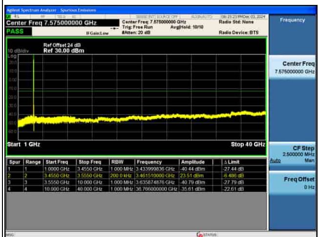
CSE_5G_n77(K)_30KHz_16QAM_100M CH633334_1RB@1_
