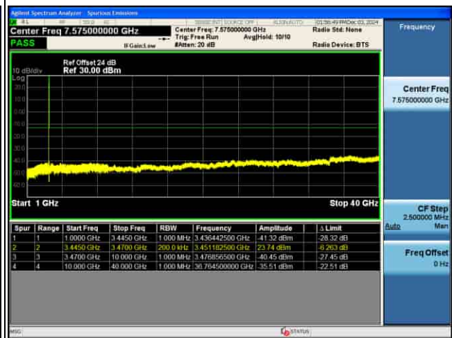
CSE_5G_n77(K)_30KHz_64QAM_15M CH633334_1RB@1_
