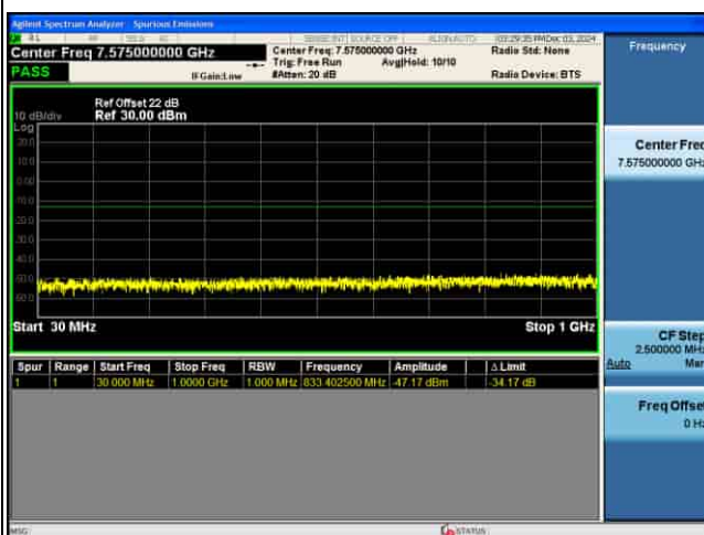
CSE_5G_n77(K)_30KHz_256QAM_30M CH633334_1RB@1_
