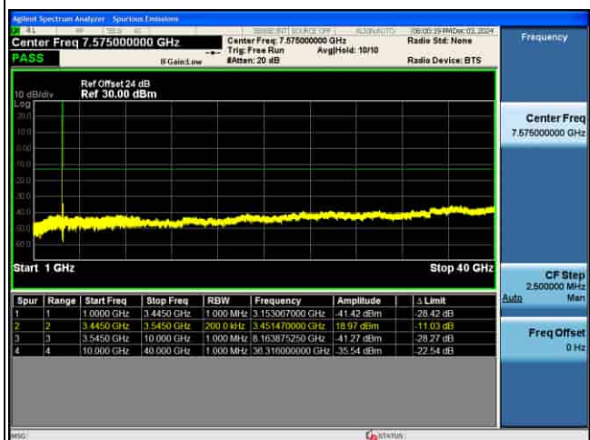
CSE_5G_n77(K)_30KHz_256QAM_90M CH633334_1RB@1_
