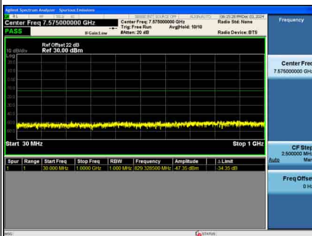
CSE_5G_n77(K)_30KHz_16QAM_100M CH633334_1RB@1
