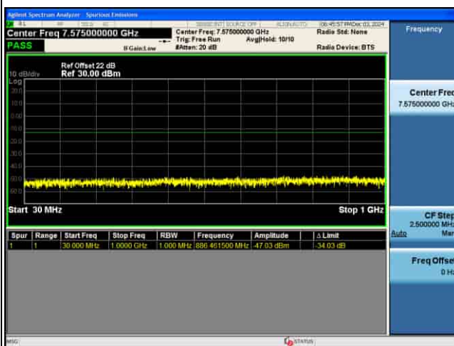
CSE_5G_n77(K)_30KHz_256QAM_100M CH633334_1RB@1_
