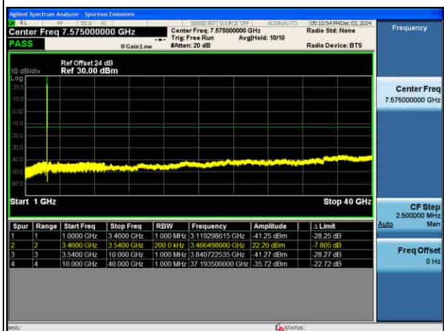
CSE_5G_n77(K)_30KHz_64QAM_70M CH634332_1RB@1_
