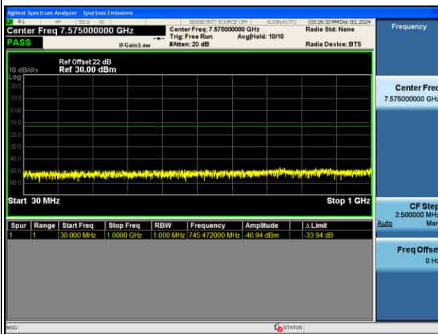
CSE_5G_n77(K)_30KHz_256QAM_40M CH631334_1RB@1_
