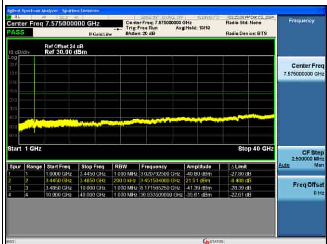
CSE_5G_n77(K)_30KHz_256QAM_30M CH633334_1RB@1_
