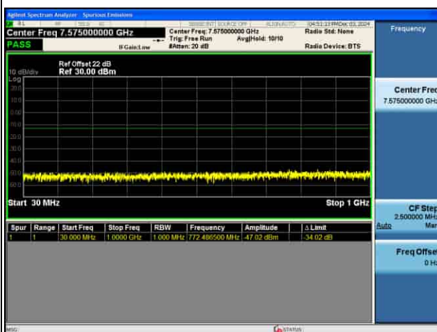
CSE_5G_n77(K)_30KHz_16QAM_60M CH632000_1RB@1
