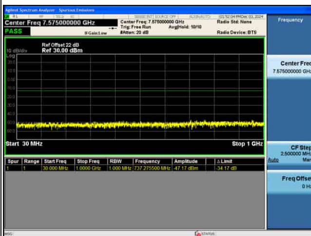
CSE_5G_n77(K)_30KHz_256QAM_15M CH633334_1RB@1_
