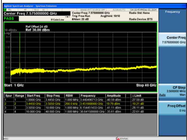
CSE_5G_n77(K)_30KHz_256QAM_50M CH633334_1RB@1_
