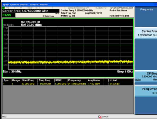
CSE_5G_n77(K)_30KHz_256QAM_50M CH631668_1RB@1_
