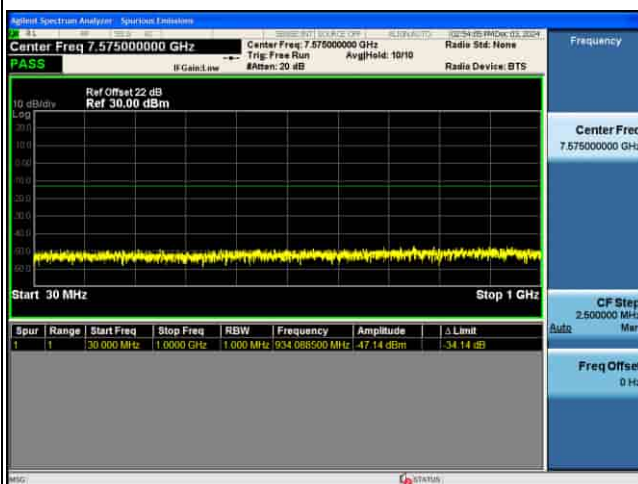
CSE_5G_n77(K)_30KHz_256QAM_20M CH633334_1RB@1_
