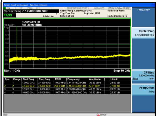
CSE_5G_n77(K)_30KHz_16QAM_80M CH632668_1RB@1_
