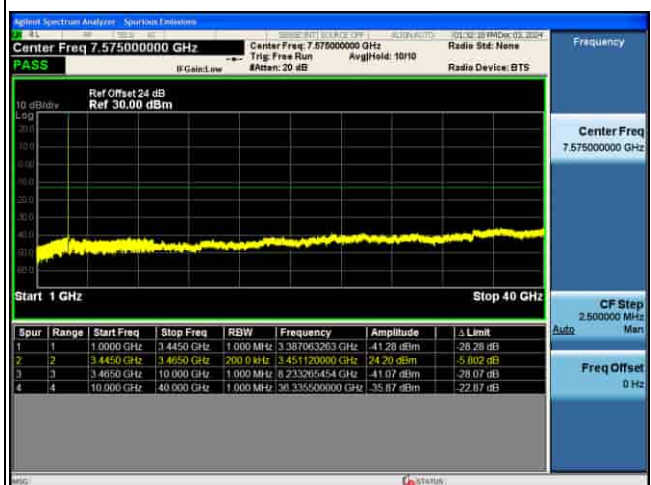
CSE_5G_n77(K)_30KHz_16QAM_10M CH630334_1RB@1_
