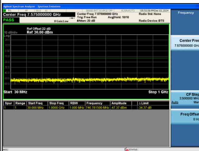
CSE_5G_n77(K)_30KHz_256QAM_80M CH633334_1RB@1_
