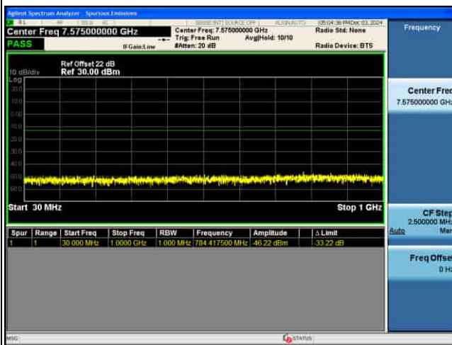
CSE_5G_n77(K)_30KHz_256QAM_80M CH632668_1RB@1_
