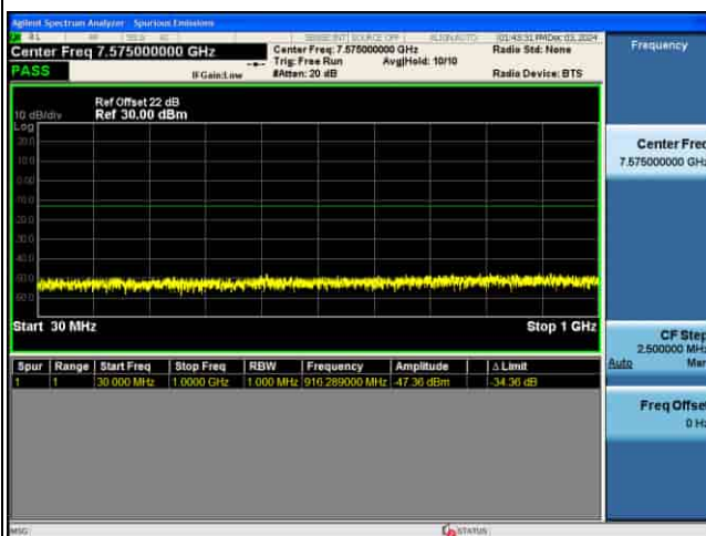
CSE_5G_n77(K)_30KHz_256QAM_10M CH633334_1RB@1_
