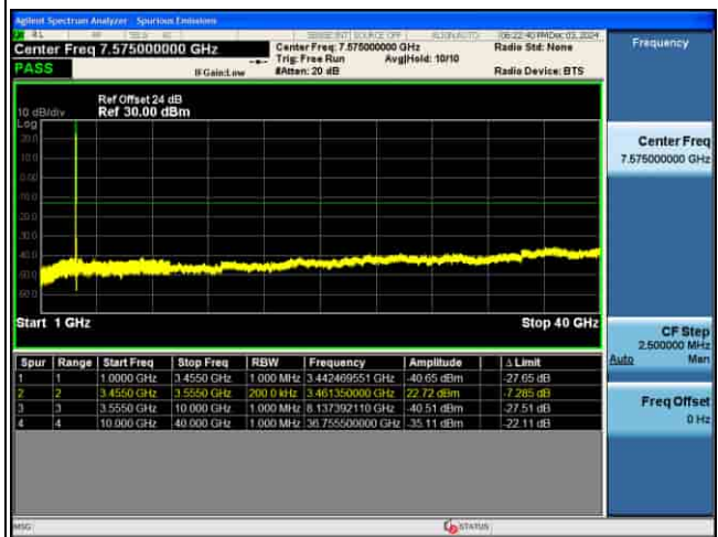
CSE_5G_n77(K)_30KHz_QPSK_100M CH633334_1RB@1_
