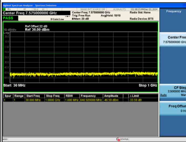
CSE_5G_n77(K)_30KHz_64QAM_10M CH633334_1RB@1
