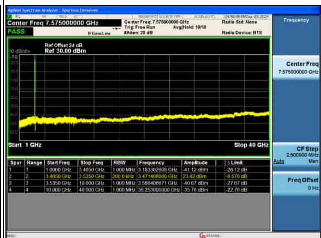
CSE_5G_n77(K)_30KHz_64QAM_60M CH634666_1RB@1_
