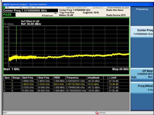
CSE_5G_n77(K)_30KHz_256QAM_70M CH632334_1RB@1_
