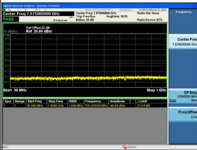
CSE_MIMO(ANT2)_n41_30KHz_16QAM_10M CH519000_1RB@1
