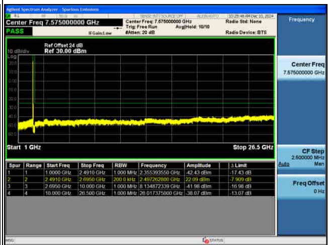
CSE_MIMO(ANT2)_n41_30KHz_16QAM_60M CH519000_1RB@1_
