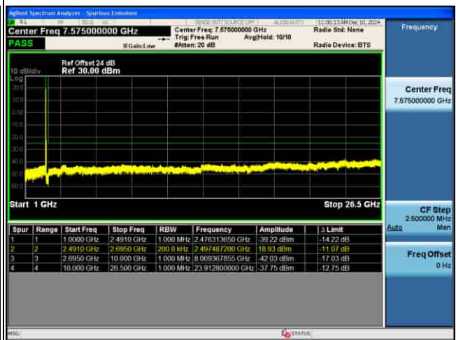
CSE_MIMO(ANT2)_n41_30KHz_16QAM_30M CH519000_1RB@1_
