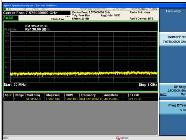
CSE_MIMO(ANT2)_n41_30KHz_QPSK_70M CH519000_1RB@1
