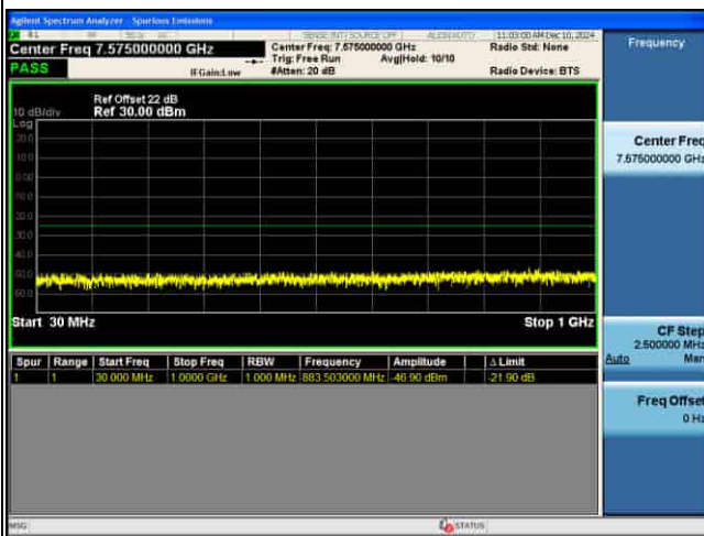
CSE_MIMO(ANT2)_n41_30KHz_QPSK_30M CH519000_1RB@1
