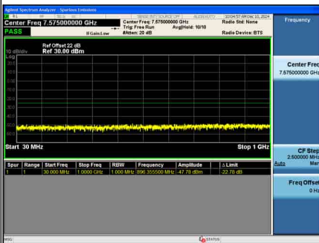
CSE_MIMO(ANT2)_n41_30KHz_16QAM_80M CH529998_1RB@1_
