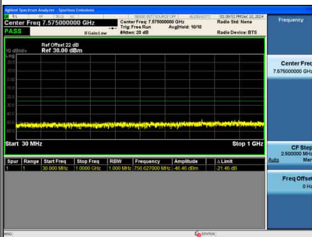
CSE_MIMO(ANT2)_n41_30KHz_QPSK_15M CH536496_1RB@1
