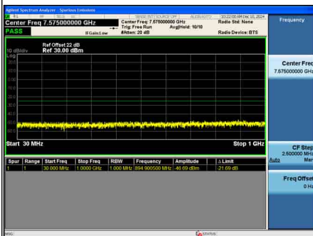
CSE_MIMO(ANT2)_n41_30KHz_QPSK_70M CH531000_1RB@1
