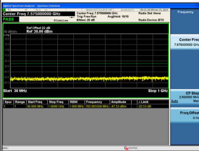
CSE_MIMO(ANT2)_n41_30KHz_16QAM_100M CH519000_1RB@1_
