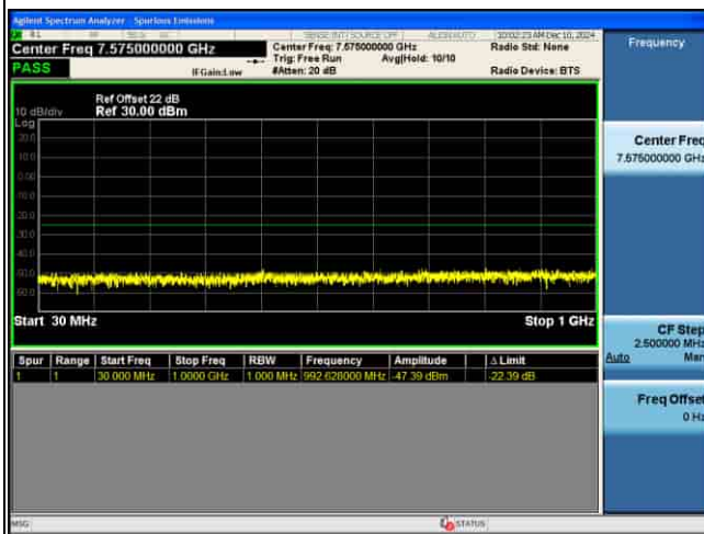
CSE_MIMO(ANT2)_n41_30KHz_QPSK_80M CH519000_1RB@1
