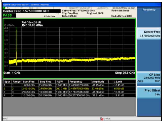
CSE_MIMO(ANT2)_n41_30KHz_16QAM_50M CH519000_1RB@1_
