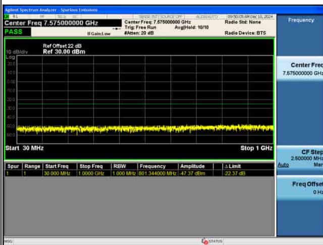
CSE_MIMO(ANT2)_n41_30KHz_16QAM_90M CH528996_1RB@1
