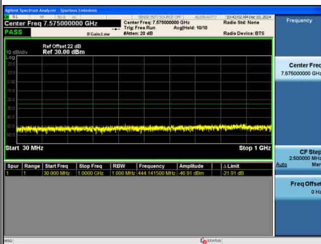
CSE_MIMO(ANT2)_n41_30KHz_QPSK_50M CH532998_1RB@1
