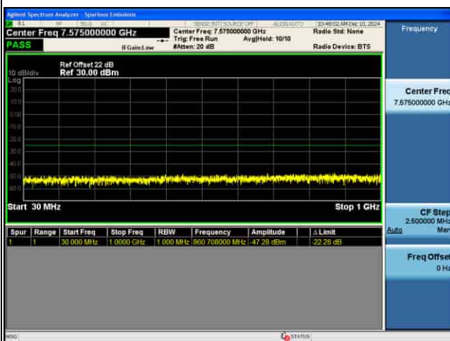
CSE_MIMO(ANT2)_n41_30KHz_16QAM_40M CH534000_1RB@1
