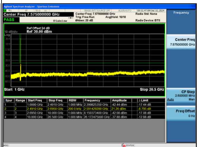
CSE_MIMO(ANT2)_n41_30KHz_16QAM_100M CH528000_1RB@1_
