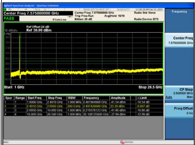
CSE_MIMO(ANT2)_n41_30KHz_16QAM_20M CH519000_1RB@1_
