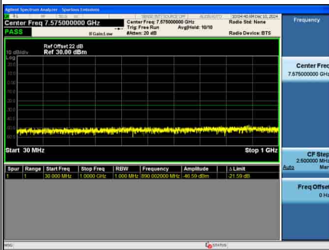
CSE_MIMO(ANT2)_n41_30KHz_16QAM_80M CH519000_1RB@1_
