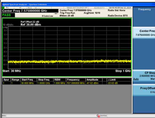
CSE_MIMO(ANT2)_n41_30KHz_16QAM_90M CH519000_1RB@1
