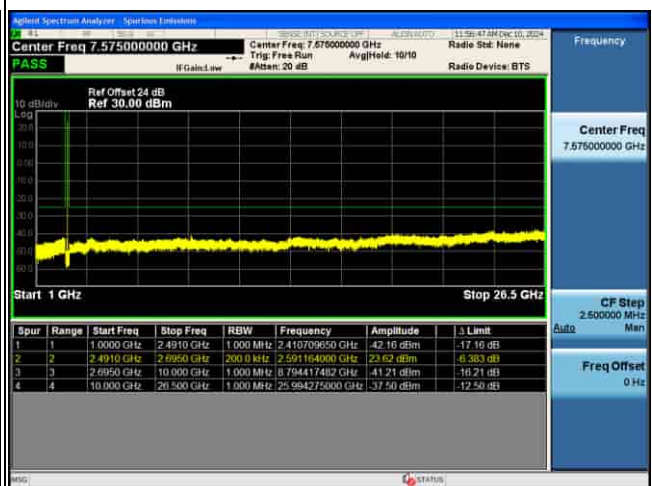
CSE_MIMO(ANT2)_n41_30KHz_16QAM_10M CH537000_1RB@1_
