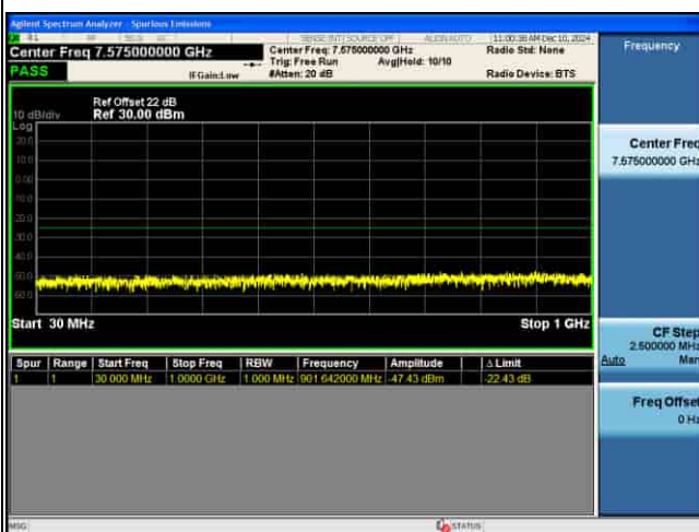
CSE_MIMO(ANT2)_n41_30KHz_16QAM_30M CH534996_1RB@1
