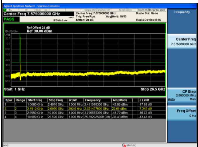
CSE_MIMO(ANT2)_n41_30KHz_QPSK_70M CH531000_1RB@1_
