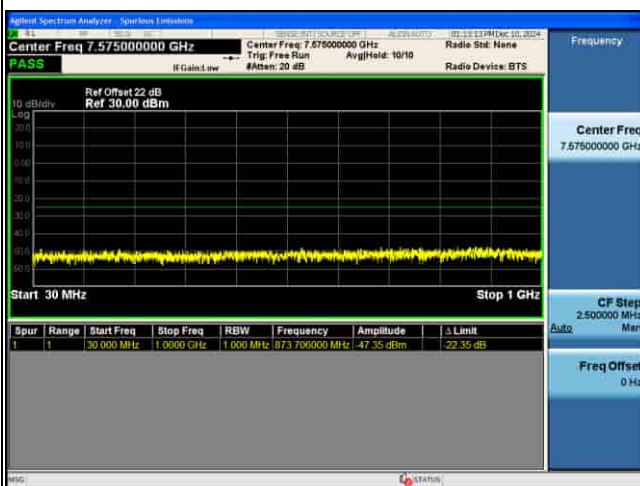
CSE_MIMO(ANT2)_n41_30KHz_16QAM_15M CH536496_1RB@1
