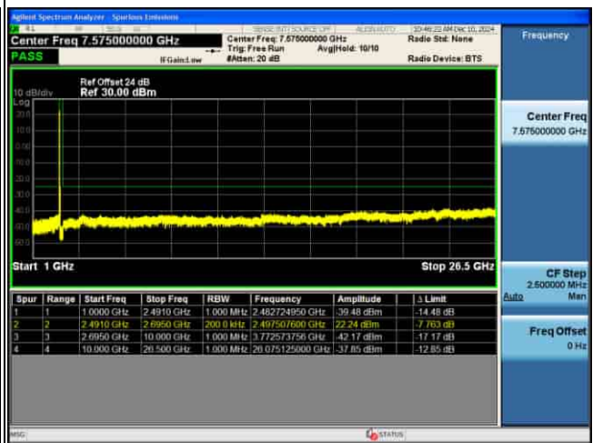
CSE_MIMO(ANT2)_n41_30KHz_16QAM_40M CH519000_1RB@1_
