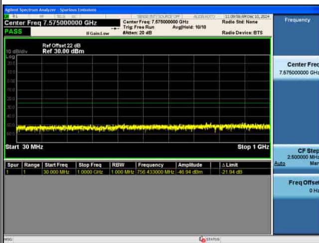
CSE_MIMO(ANT2)_n41_30KHz_16QAM_20M CH535998_1RB@1
