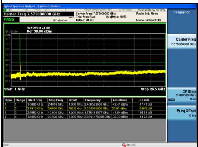
CSE_MIMO(ANT2)_n41_30KHz_QPSK_80M CH529998_1RB@1_
