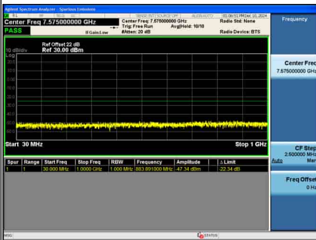
CSE_MIMO(ANT2)_n41_30KHz_QPSK_15M CH519000_1RB@1
