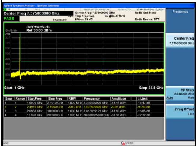
CSE_MIMO(ANT2)_n41_30KHz_QPSK_50M CH519000_1RB@1_
