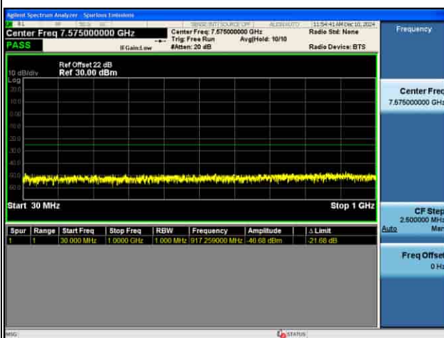
CSE_MIMO(ANT2)_n41_30KHz_16QAM_10M CH537000_1RB@1
