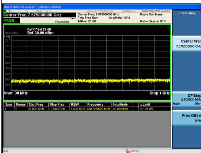
CSE_MIMO(ANT2)_n41_30KHz_QPSK_80M CH529998_1RB@1
