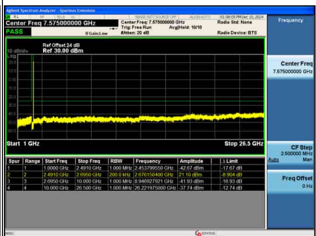
CSE_MIMO(ANT2)_n41_30KHz_QPSK_15M CH536496_1RB@1_
