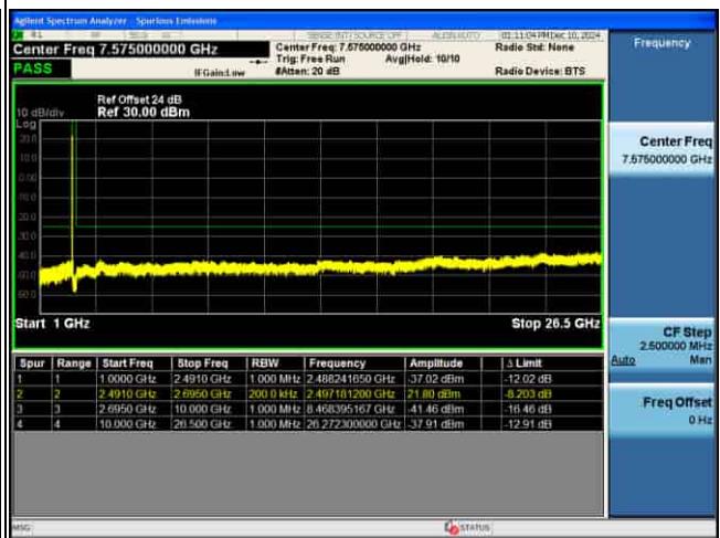
CSE_MIMO(ANT2)_n41_30KHz_16QAM_15M CH519000_1RB@1_
