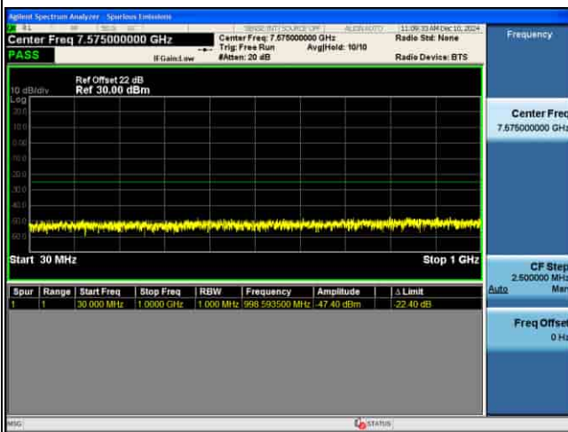
CSE_MIMO(ANT2)_n41_30KHz_16QAM_20M CH519000_1RB@1
