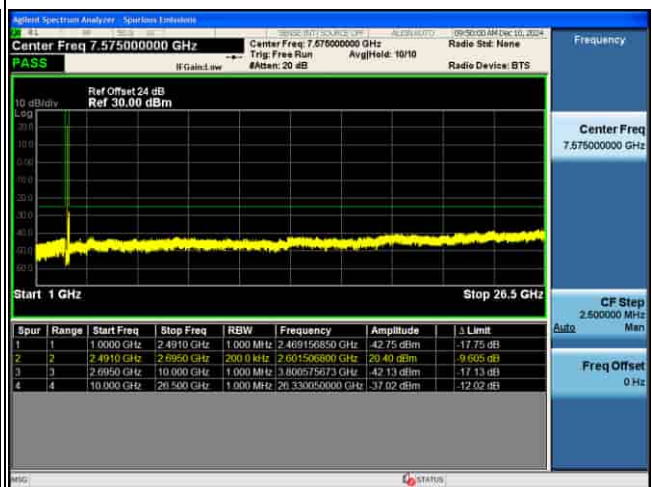
CSE_MIMO(ANT2)_n41_30KHz_16QAM_90M CH528996_1RB@1_
