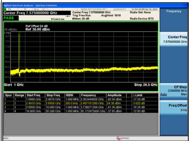
CSE_MIMO(ANT2)_n41_30KHz_16QAM_10M CH519000_1RB@1_
