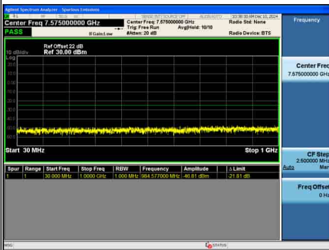
CSE_MIMO(ANT2)_n41_30KHz_16QAM_50M CH519000_1RB@1_
