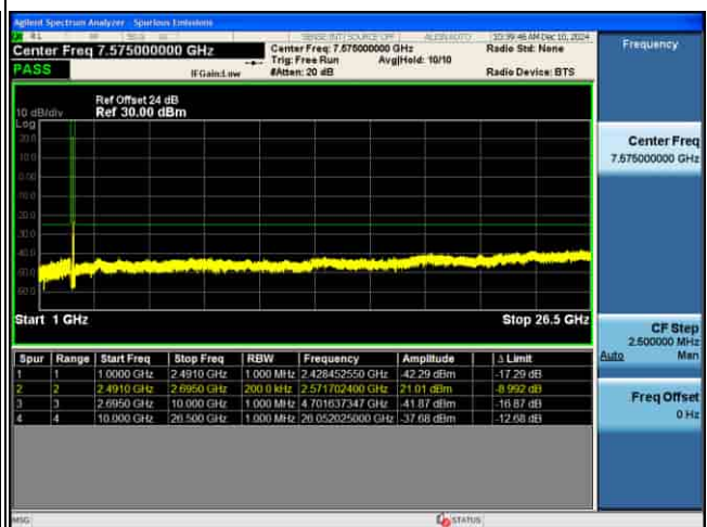
CSE_MIMO(ANT2)_n41_30KHz_16QAM_50M CH532998_1RB@1_
