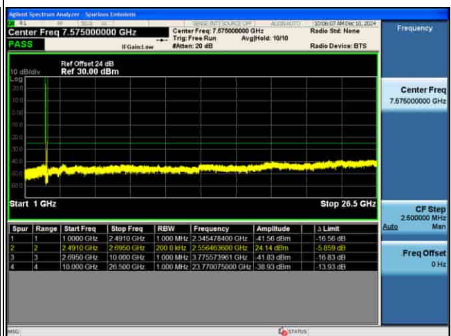
CSE_MIMO(ANT2)_n41_30KHz_16QAM_80M CH529998_1RB@1_
