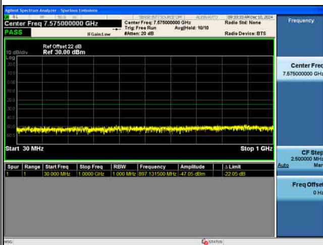
CSE_MIMO(ANT2)_n41_30KHz_16QAM_100M CH528000_1RB@1_
