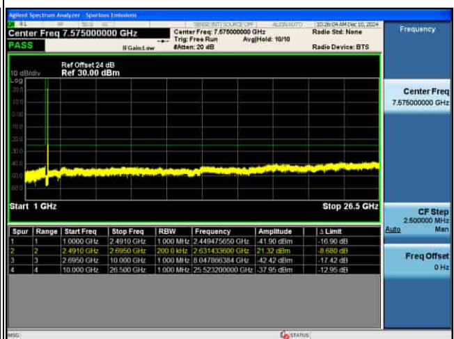
CSE_MIMO(ANT2)_n41_30KHz_16QAM_60M CH531996_1RB@1_
