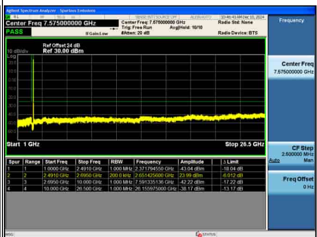
CSE_MIMO(ANT2)_n41_30KHz_16QAM_40M CH534000_1RB@1_
