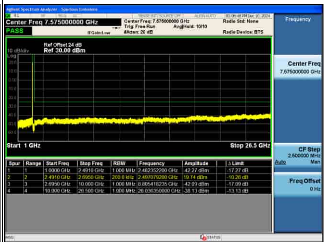
CSE_MIMO(ANT2)_n41_30KHz_QPSK_15M CH519000_1RB@1_
