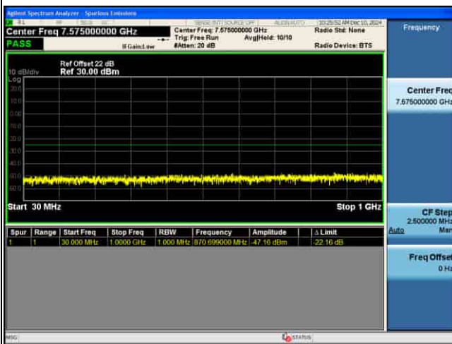
CSE_MIMO(ANT2)_n41_30KHz_16QAM_60M CH519000_1RB@1
