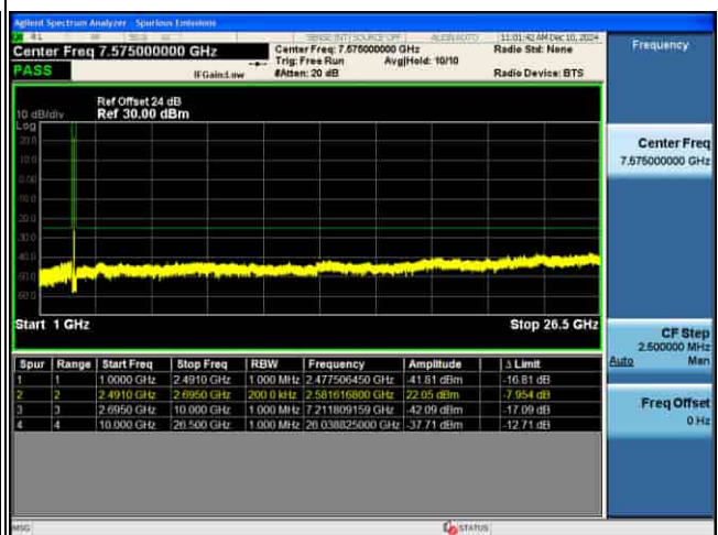
CSE_MIMO(ANT2)_n41_30KHz_16QAM_30M CH534996_1RB@1_
