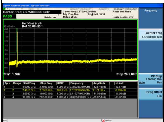
CSE_MIMO(ANT2)_n41_30KHz_16QAM_15M CH536496_1RB@1_
