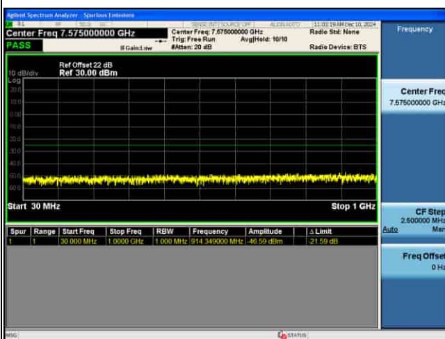
CSE_MIMO(ANT2)_n41_30KHz_QPSK_30M CH534996_1RB@1
