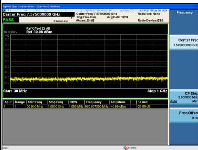
CSE_MIMO(ANT2)_n41_30KHz_16QAM_50M CH532998_1RB@1_
