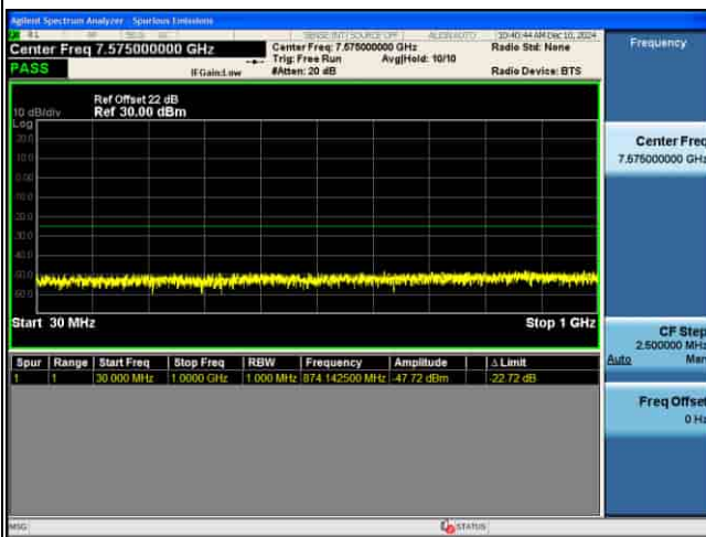
CSE_MIMO(ANT2)_n41_30KHz_QPSK_50M CH519000_1RB@1
