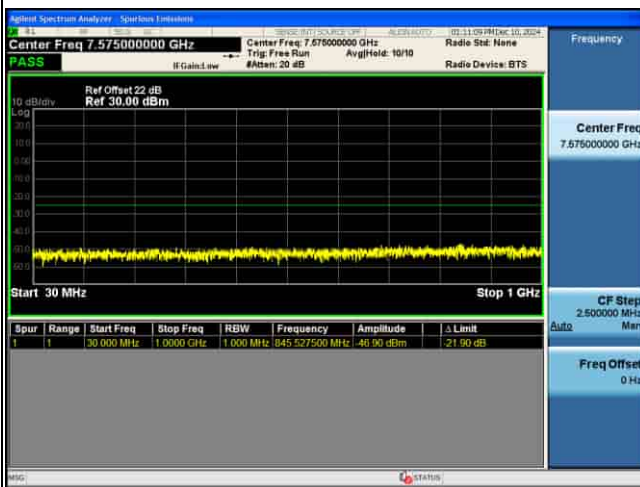
CSE_MIMO(ANT2)_n41_30KHz_16QAM_15M CH519000_1RB@1
