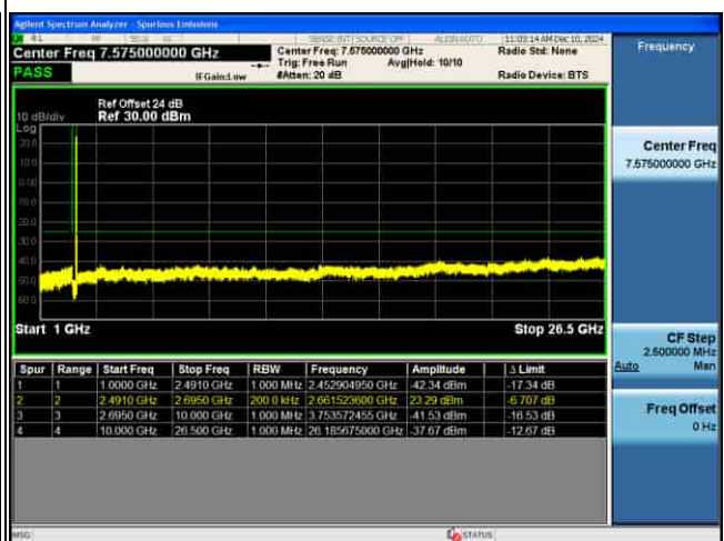
CSE_MIMO(ANT2)_n41_30KHz_QPSK_30M CH534996_1RB@1_
