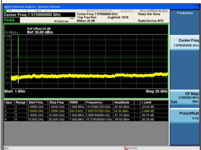
CSE_5G_n25_15KHz_64QAM_20M CH381000_1RB@1_
