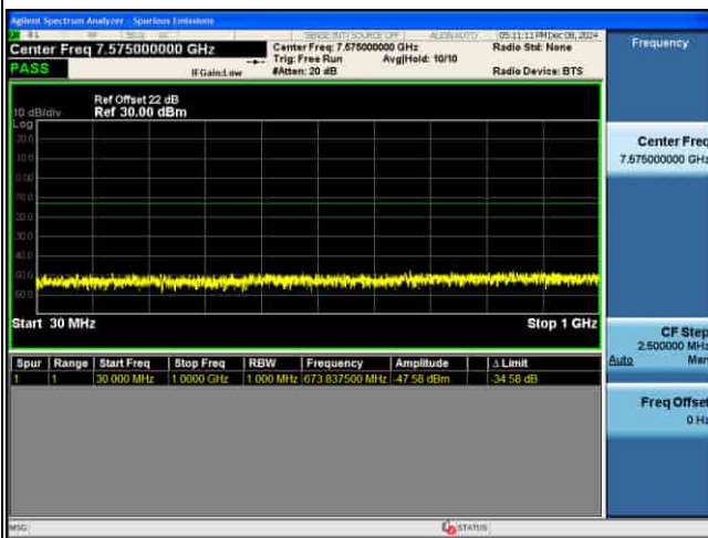
CSE_5G_n25_15KHz_64QAM_20M CH376500_1RB@1
