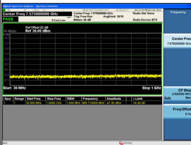
CSE_5G_n25_15KHz_64QAM_20M CH381000_1RB@1
