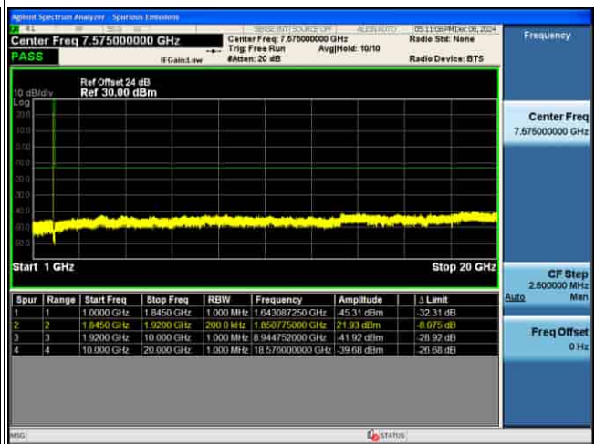
CSE_5G_n25_15KHz_64QAM_20M CH376500_1RB@1_
