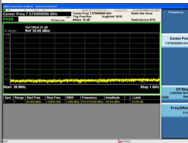
CSE_MIMO(ANT5)_n48_30KHz_256QAM_15M CH646166_1RB@1_
