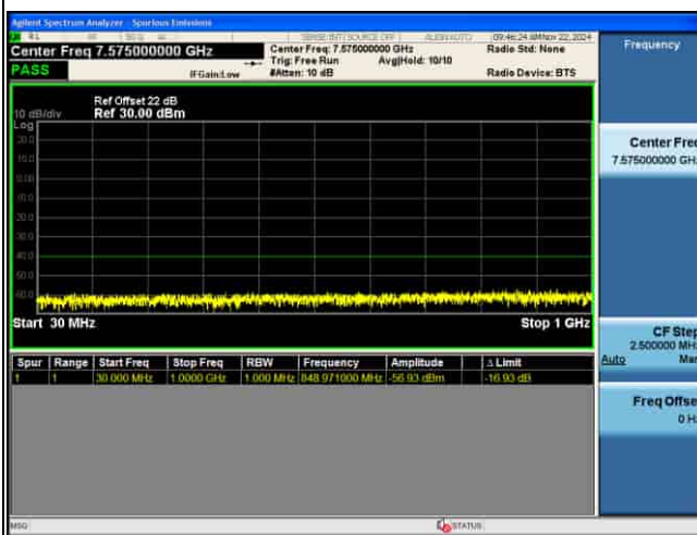
CSE_MIMO(ANT5)_n48_30KHz_16QAM_40M CH641666_1RB@1
