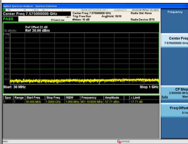
CSE_5G_n48_30KHz_64QAM_40M CH641666 1RB@1
