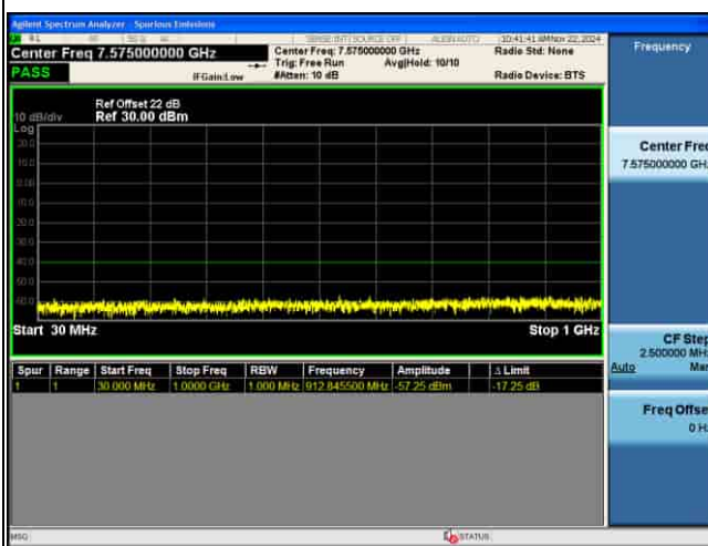
CSE_MIMO(ANT5)_n48_30KHz_QPSK_30M CH645666_1RB@1
