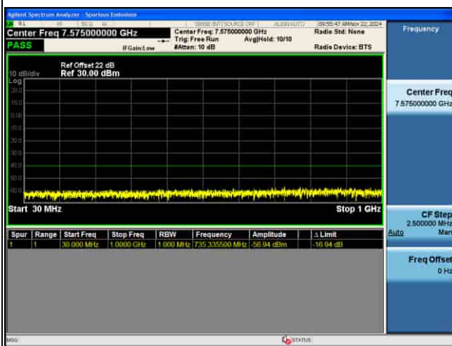
CSE_MIMO(ANT5)_n48_30KHz_64QAM_40M CH641666_1RB@1
