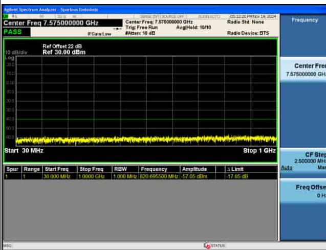
CSE_5G_n48_30KHz_64QAM_15M CH646166 1RB@1
