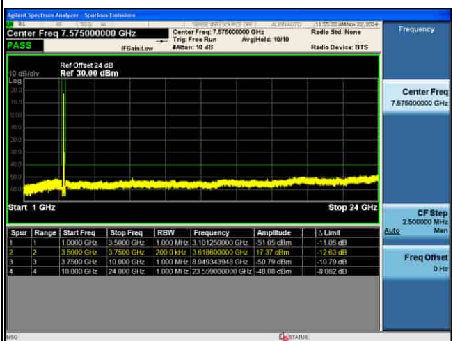
CSE_MIMO(ANT5)_n48_30KHz_16QAM_15M CH646166_1RB@1_
