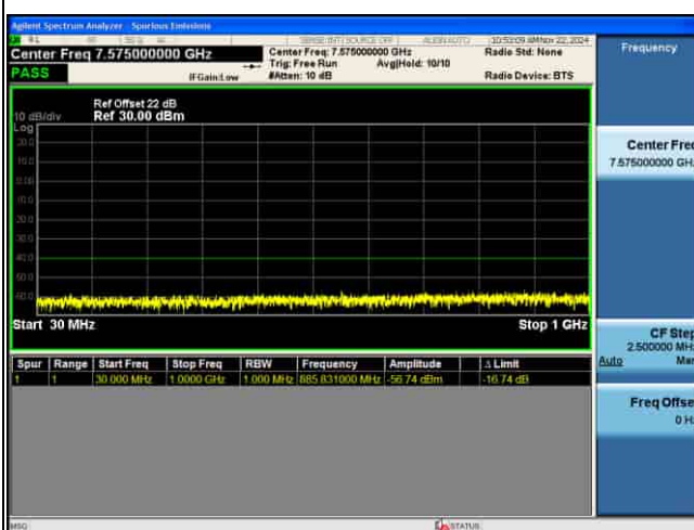
CSE_MIMO(ANT5)_n48_30KHz_16QAM_20M CH646000_1RB@1
