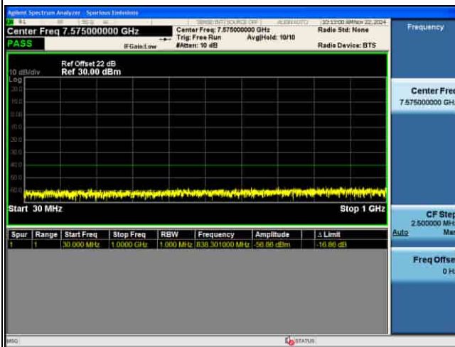
CSE_MIMO(ANT5)_n48_30KHz_256QAM_30M CH641666_1RB@1_
