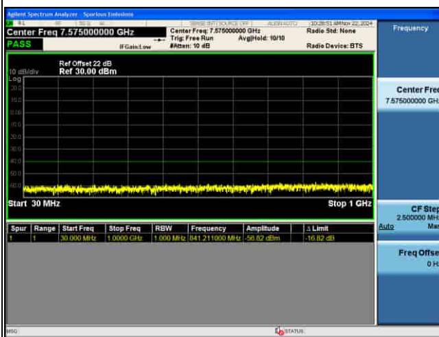
CSE_MIMO(ANT5)_n48_30KHz_16QAM_30M CH641666_1RB@1
