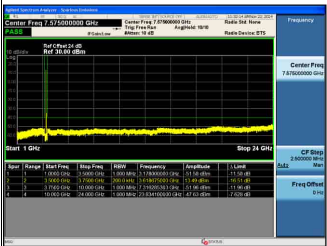
CSE_MIMO(ANT5)_n48_30KHz_256QAM_15M CH646166_1RB@1_
