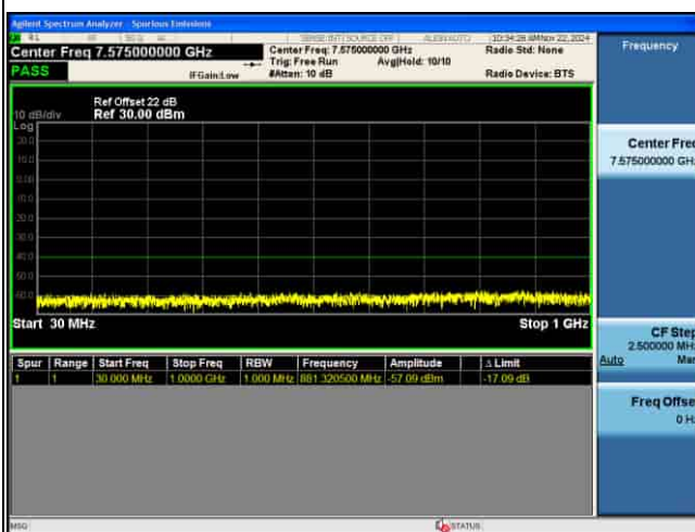
CSE_MIMO(ANT5)_n48_30KHz_16QAM_30M CH645666_1RB@1
