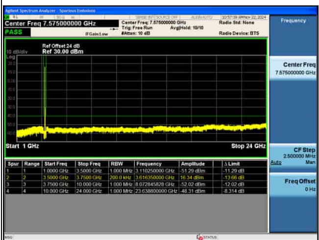
CSE_MIMO(ANT5)_n48_30KHz_16QAM_20M CH646000_1RB@1_
