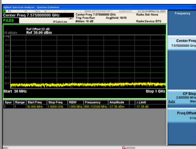
CSE_MIMO(ANT5)_n48_30KHz_256QAM_20M CH646000_1RB@1
