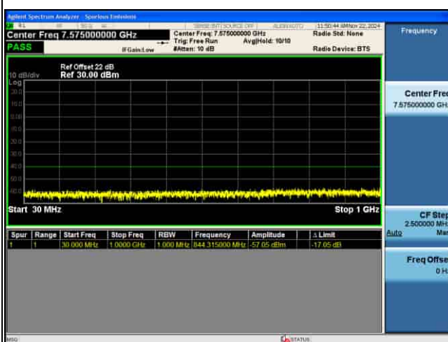
CSE_MIMO(ANT5)_n48_30KHz_16QAM_15M CH646166_1RB@1
