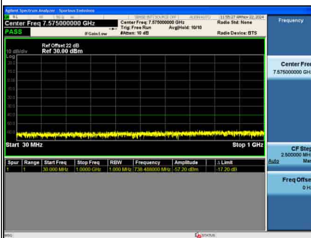
CSE_MIMO(ANT5)_n48_30KHz_16QAM_15M CH646166_1RB@1
