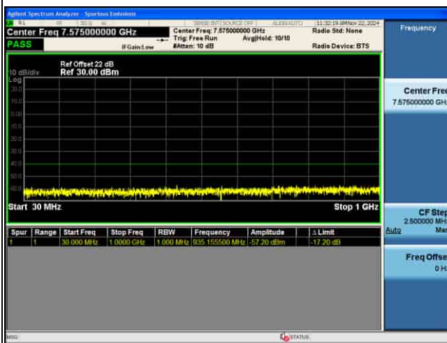
CSE_MIMO(ANT5)_n48_30KHz_256QAM_15M CH646166_1RB@1_
