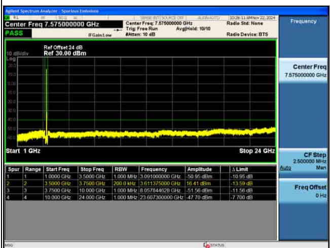
CSE_MIMO(ANT5)_n48_30KHz_64QAM_30M CH645666_1RB@1_
