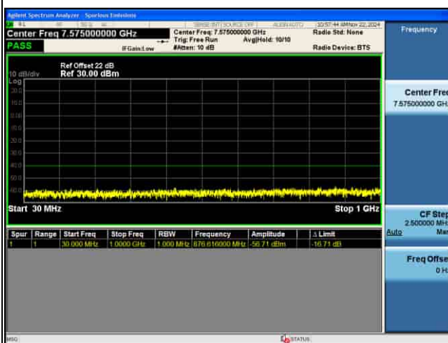
CSE_MIMO(ANT5)_n48_30KHz_16QAM_20M CH646000_1RB@1
