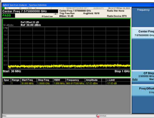
CSE_5G_n48_30KHz_64QAM_10M CH641666 1RB@1
