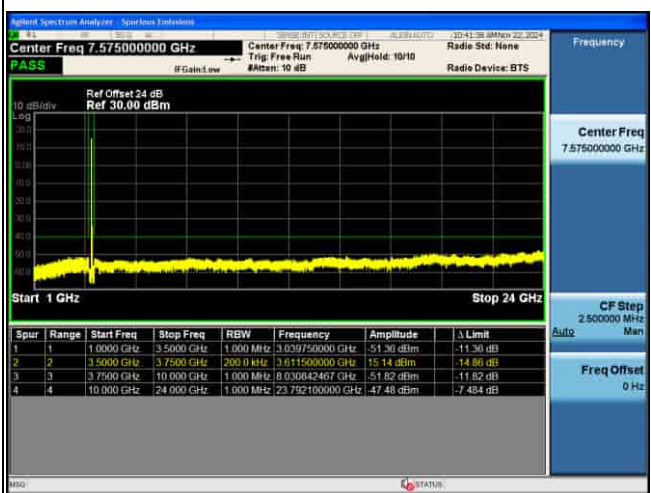
CSE_MIMO(ANT5)_n48_30KHz_QPSK_30M CH645666_1RB@1_
