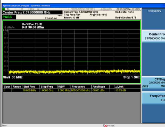
CSE_5G_n48_30KHz_256QAM_30M CH645666 1RB@1
