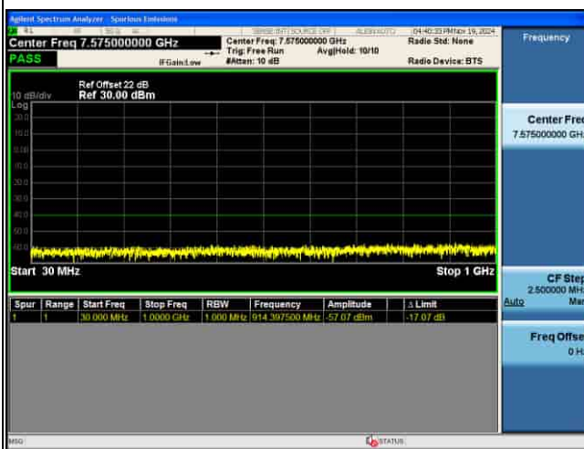
CSE_5G_n48_30KHz_64QAM_20M CH641666 1RB@1
