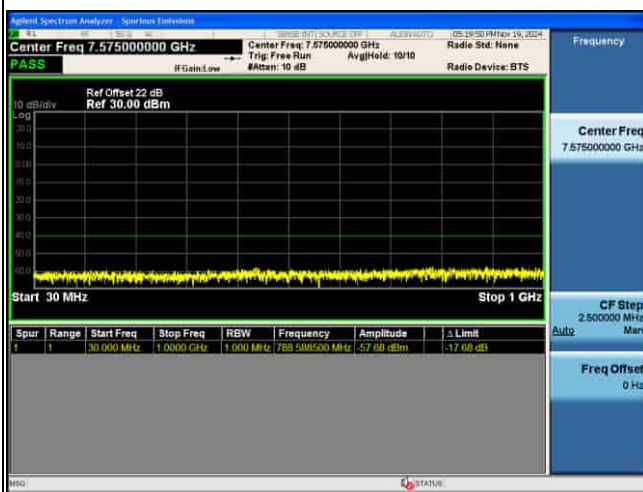
CSE_5G_n48_30KHz_16QAM_15M CH641666 1RB@1
