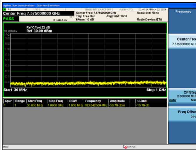
CSE_MIMO(ANT5)_n48_30KHz_256QAM_10M CH641666_1RB@1
