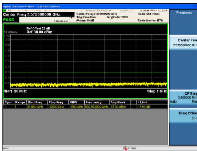
CSE_MIMO(ANT5)_n48_30KHz_64QAM_15M CH641666_1RB@1
