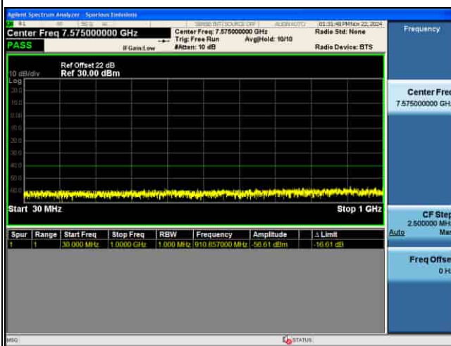
CSE_MIMO(ANT5)_n48_30KHz_64QAM_10M CH641666_1RB@1
