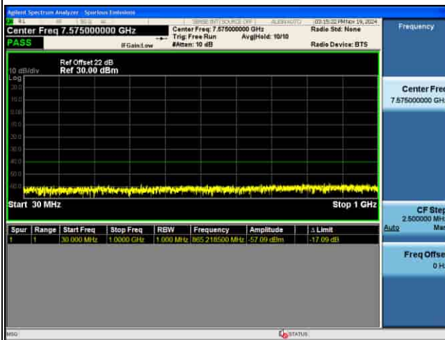
CSE_5G_n48_30KHz_256QAM_40M CH641666 1RB@1
