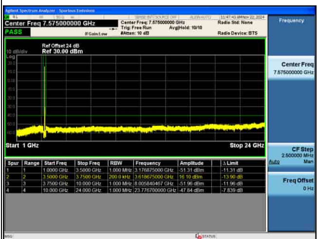
CSE_MIMO(ANT5)_n48_30KHz_64QAM_15M CH646166_1RB@1_
