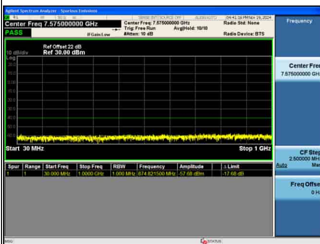
CSE_5G_n48_30KHz_64QAM_20M CH646000 1RB@1
