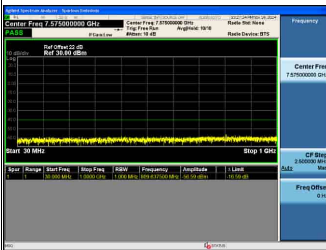
CSE_5G_n48_30KHz_256QAM_30M CH641666 1RB@1
