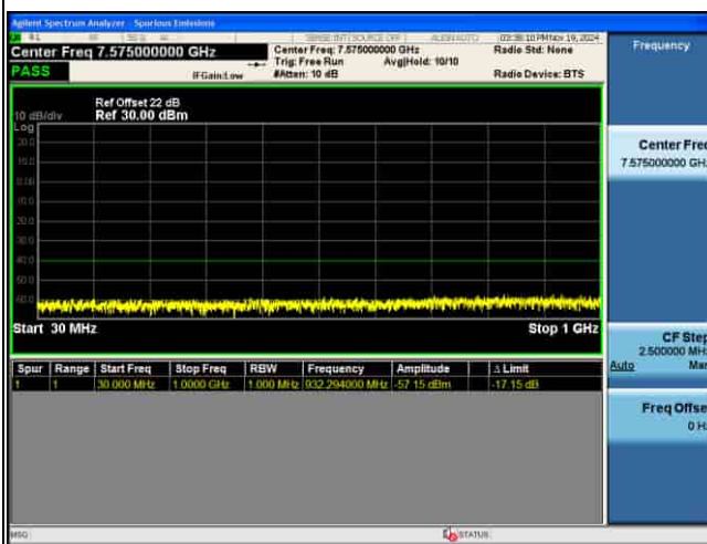
CSE_5G_n48_30KHz_64QAM_30M CH641666 1RB@1
