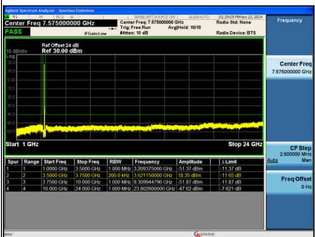
CSE_MIMO(ANT5)_n48_30KHz_16QAM_10M CH646332_1RB@1_
