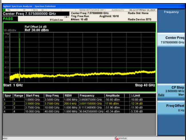
CSE_5G_n48_30KHz_64QAM_10M CH646332 1RB@1_
