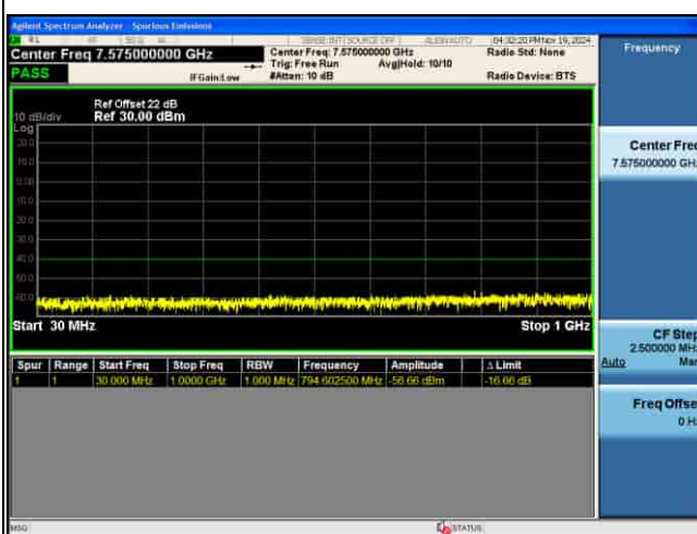
CSE_5G_n48_30KHz_16QAM_20M CH646000 1RB@1
