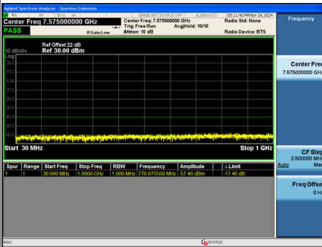
CSE_5G_n48_30KHz_64QAM_15M CH641666 1RB@1
