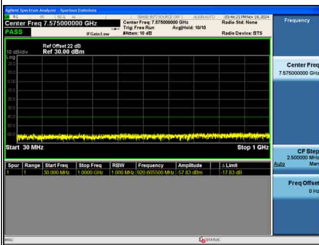
CSE_5G_n48_30KHz_16QAM_30M CH641666 1RB@1
