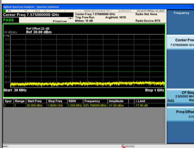
CSE_5G_n48_30KHz_256QAM_40M CH645332 1RB@1
