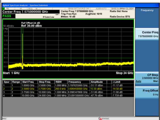
CSE_MIMO(ANT5)_n48_30KHz_64QAM_40M CH645332_1RB@1_
