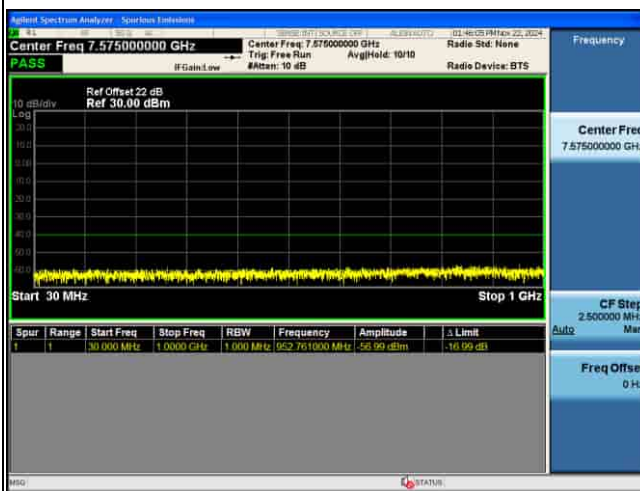
CSE_MIMO(ANT5)_n48_30KHz_256QAM_10M CH646332_1RB@1
