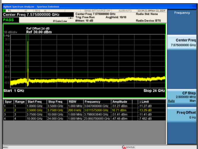
CSE_MIMO(ANT5)_n48_30KHz_16QAM_30M CH645666_1RB@1_
