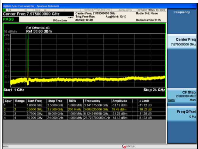
CSE_5G_n48_30KHz_16QAM_40M CH645332 1RB@1_
