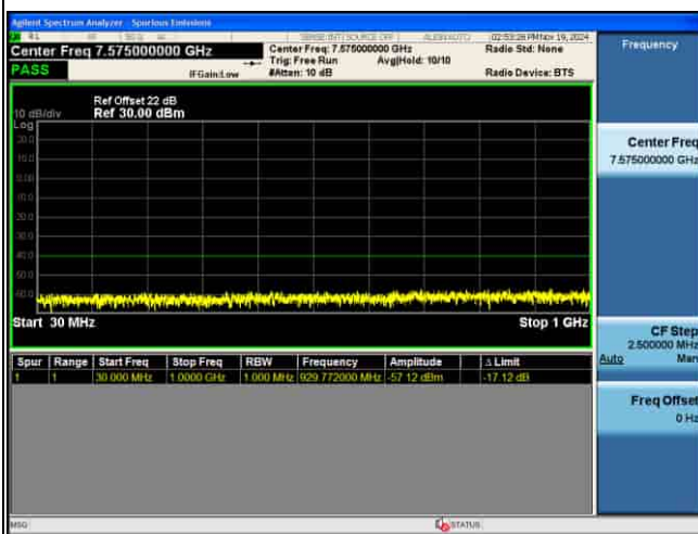
CSE_5G_n48_30KHz_16QAM_40M CH641666 1RB@1
