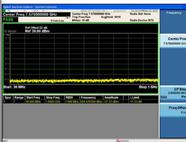
CSE_MIMO(ANT5)_n48_30KHz_64QAM_10M CH646332_1RB@1
