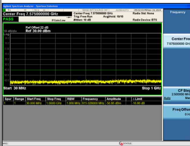
CSE_5G_n48_30KHz_256QAM_15M CH641666 1RB@1
