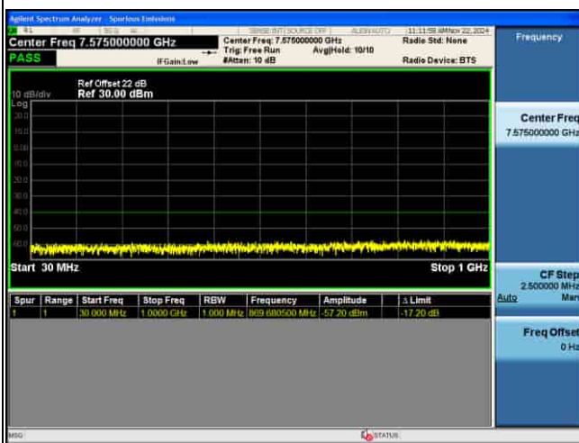
CSE_MIMO(ANT5)_n48_30KHz_256QAM_20M CH641666_1RB@1
