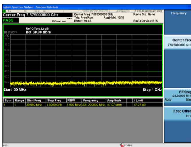
CSE_MIMO(ANT5)_n48_30KHz_64QAM_15M CH646166_1RB@1
