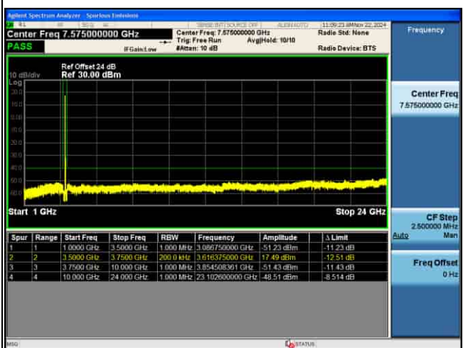
CSE_MIMO(ANT5)_n48_30KHz_64QAM_20M CH646000_1RB@1_
