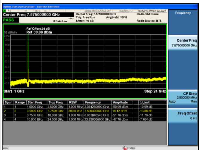
CSE_MIMO(ANT5)_n48_30KHz_16QAM_40M CH645332_1RB@1_
