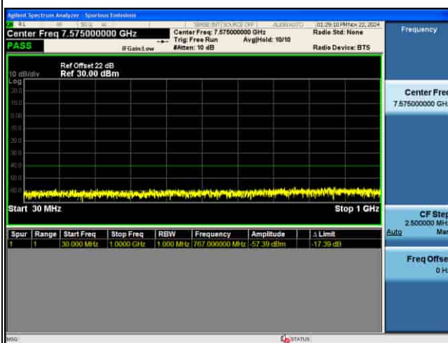
CSE_MIMO(ANT5)_n48_30KHz_16QAM_10M CH646332_1RB@1
