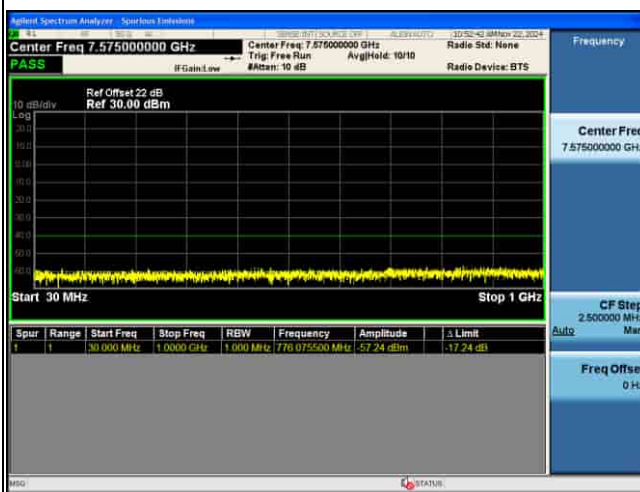
CSE_MIMO(ANT5)_n48_30KHz_16QAM_20M CH641666_1RB@1
