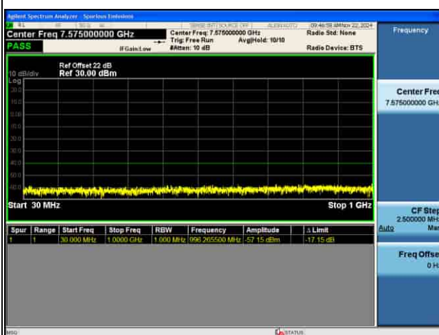
CSE_MIMO(ANT5)_n48_30KHz_16QAM_40M CH645332_1RB@1
