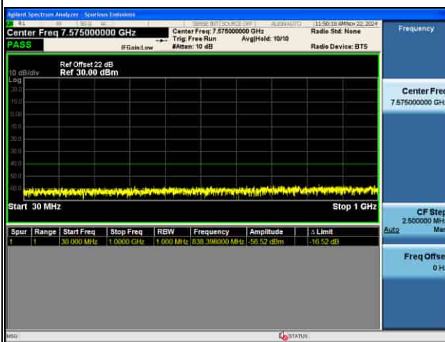
CSE_MIMO(ANT5)_n48_30KHz_16QAM_15M CH641666_1RB@1
