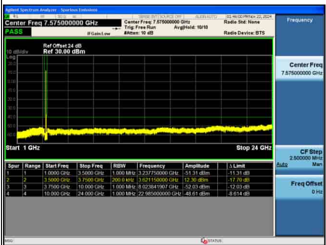
CSE_MIMO(ANT5)_n48_30KHz_256QAM_10M CH646332_1RB@1_
