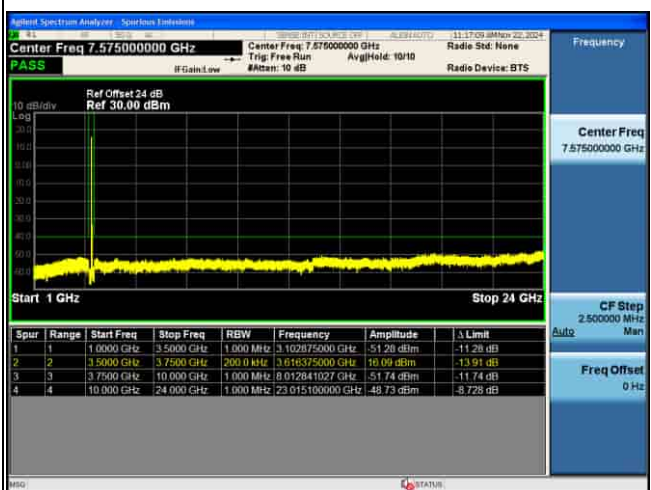
CSE_MIMO(ANT5)_n48_30KHz_256QAM_20M CH646000_1RB@1_
