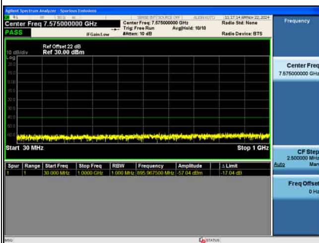
CSE_MIMO(ANT5)_n48_30KHz_256QAM_20M CH646000_1RB@1
