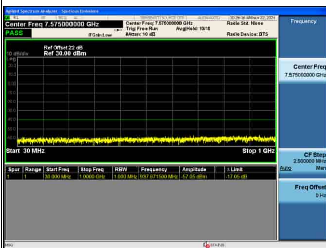
CSE_MIMO(ANT5)_n48_30KHz_64QAM_30M CH645666_1RB@1
