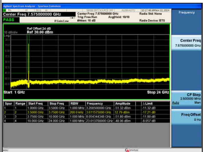
CSE_MIMO(ANT5)_n48_30KHz_256QAM_30M CH645666_1RB@1_
