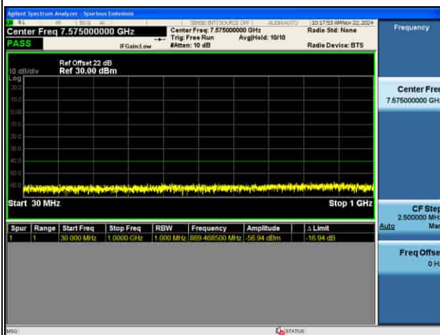
CSE_MIMO(ANT5)_n48_30KHz_256QAM_30M CH645666_1RB@1_
