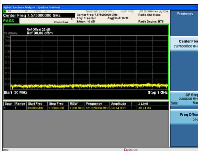
CSE_5G_n48_30KHz_64QAM_30M CH645666 1RB@1
