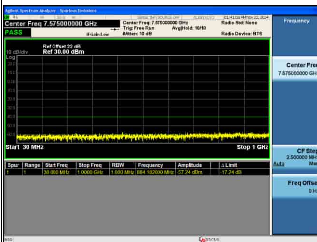
CSE_MIMO(ANT5)_n48_30KHz_256QAM_10M CH646332_1RB@1
