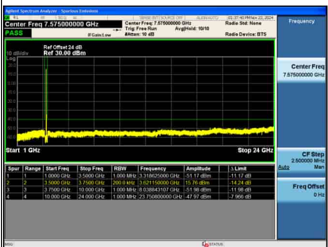
CSE_MIMO(ANT5)_n48_30KHz_64QAM_10M CH646332_1RB@1_
