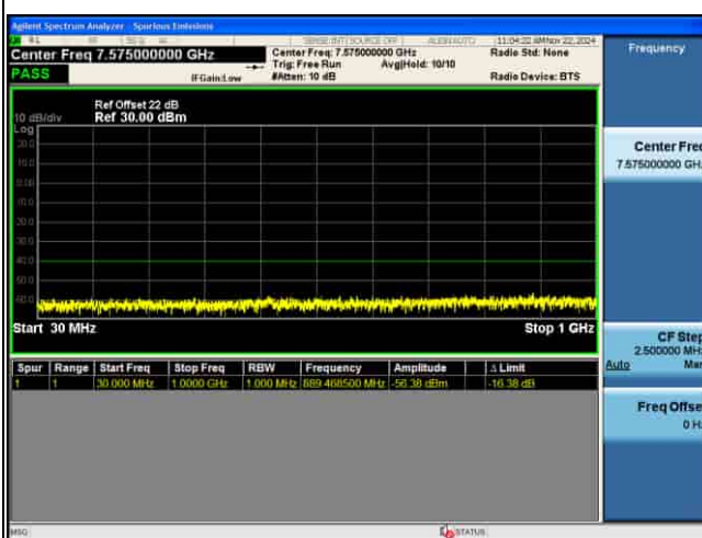
CSE_MIMO(ANT5)_n48_30KHz_64QAM_20M CH646000_1RB@1
