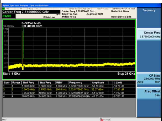
CSE_5G_n48_30KHz_16QAM_10M CH646332 1RB@1_
