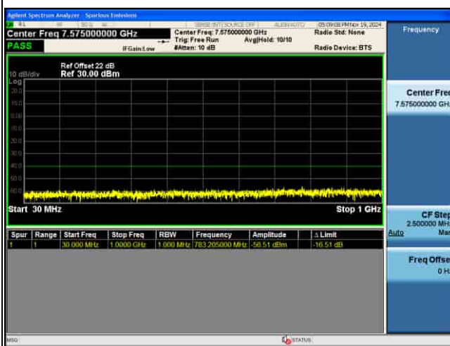
CSE_5G_n48_30KHz_256QAM_15M CH646166 1RB@1
