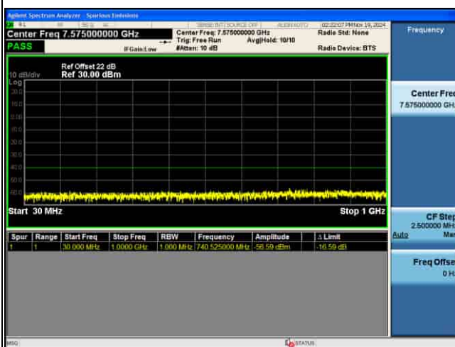
CSE_5G_n48_30KHz_.PI2-BPSK_40M CH645332 1RB@1_
