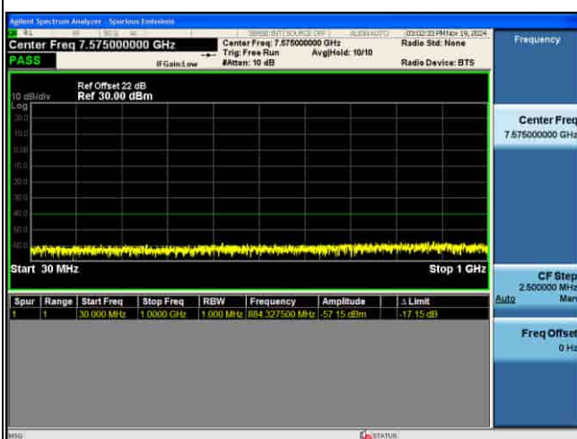
CSE_5G_n48_30KHz_64QAM_40M CH645332 1RB@1
