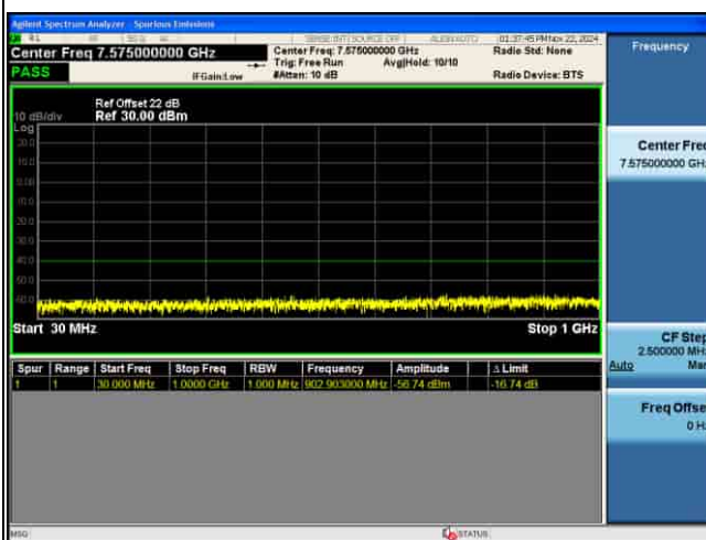
CSE_MIMO(ANT5)_n48_30KHz_64QAM_10M CH646332_1RB@1
