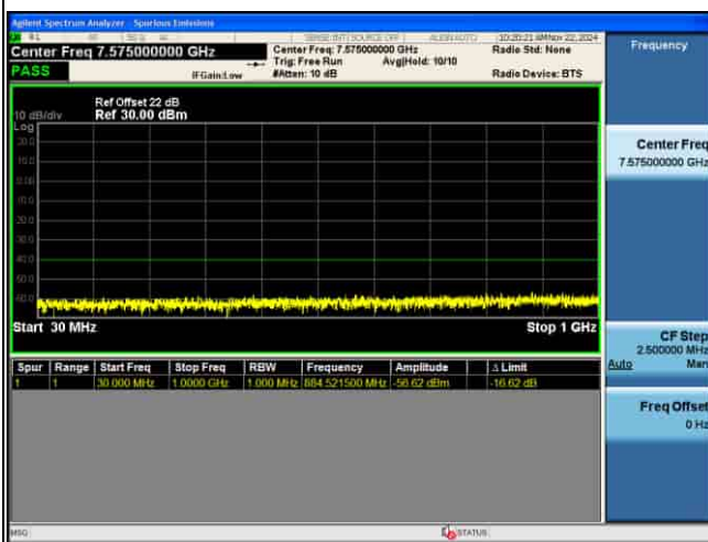
CSE_MIMO(ANT5)_n48_30KHz_64QAM_30M CH641666_1RB@1
