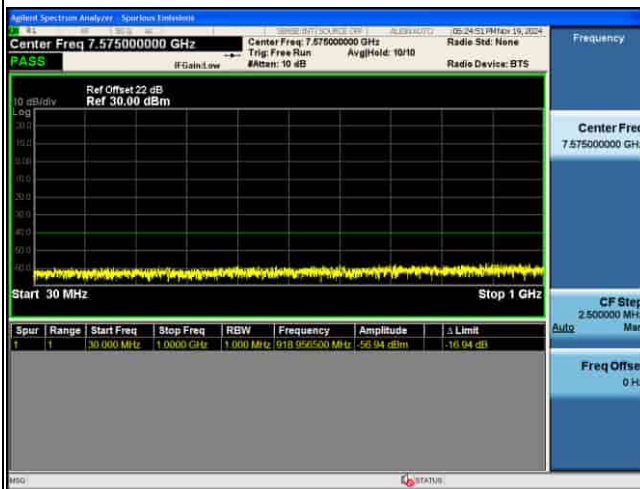
CSE_5G_n48_30KHz_256QAM_10M CH641666 1RB@1
