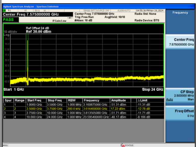
CSE_5G_n48_30KHz_256QAM_20M CH646000 1RB@1_
