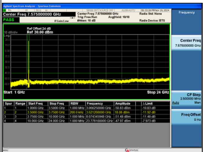
CSE_5G_n48_30KHz_256QAM_10M CH646332 1RB@1_
