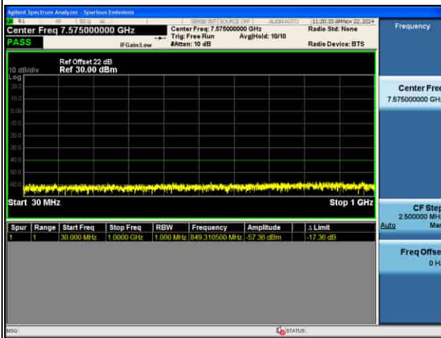
CSE_MIMO(ANT5)_n48_30KHz_256QAM_15M CH641666_1RB@1_
