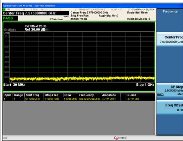
CSE_5G_n48_30KHz_16QAM_30M CH645666 1RB@1
