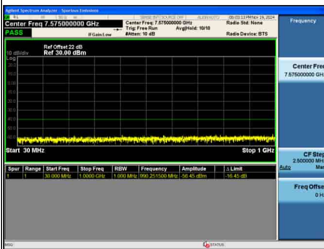
CSE_5G_n48_30KHz_16QAM_10M CH641666 1RB@1
