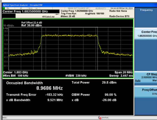
OCC_5G_n25_15KHz_16QAM_10M CH376500
