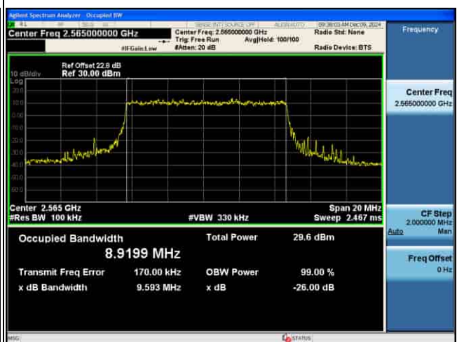
OCC_5G_n7_15KHz_16QAM_10M CH513000
