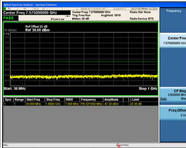
CSE_4G_B41_256QAM_20M CH40640 1RB@0
