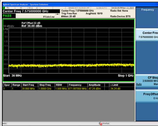
CSE_4G_B66_16QAM_1.4M CH132322 1RB@Mid
