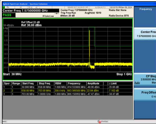
CSE_4G_B71_16QAM_10M CH133297 1RB@0
