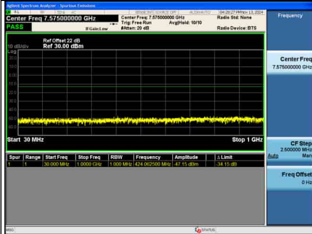
CSE_4G_B66_64QAM_5M CH132647 1RB@0
