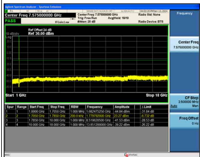
CSE_4G_B66_16QAM_1.4M CH132665 1RB@Max_
