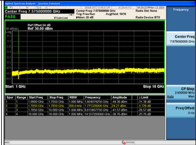
CSE_4G_B66_64QAM_5M CH132647 1RB@0_
