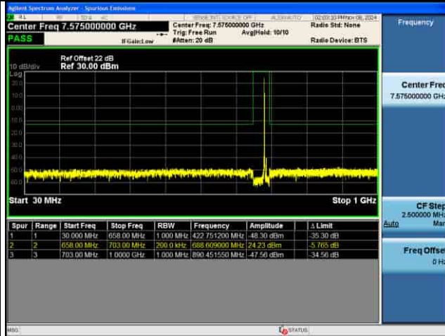
CSE_4G_B71_16QAM_10M CH133422 1RB@0
