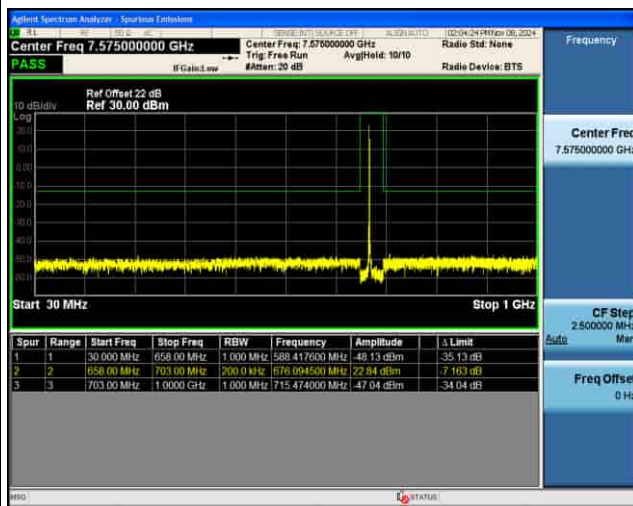
CSE_4G_B71_16QAM_10M CH133422 1RB@0
