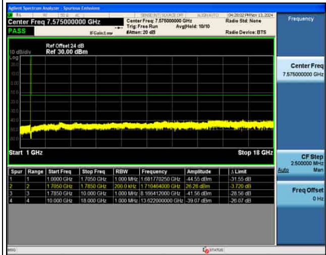
CSE_4G_B66_64QAM_5M CH132322 1RB@0_
