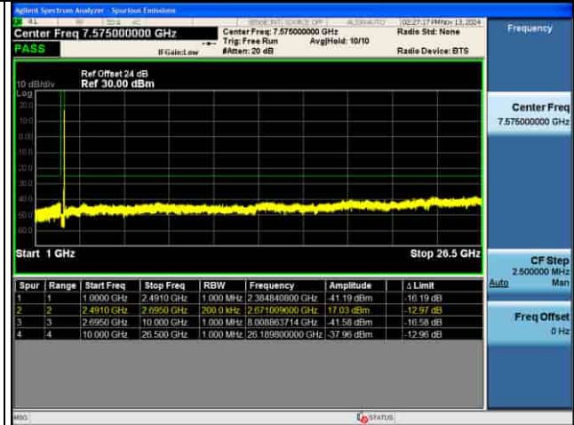
CSE_4G_B41_256QAM_20M CH41490 1RB@0_
