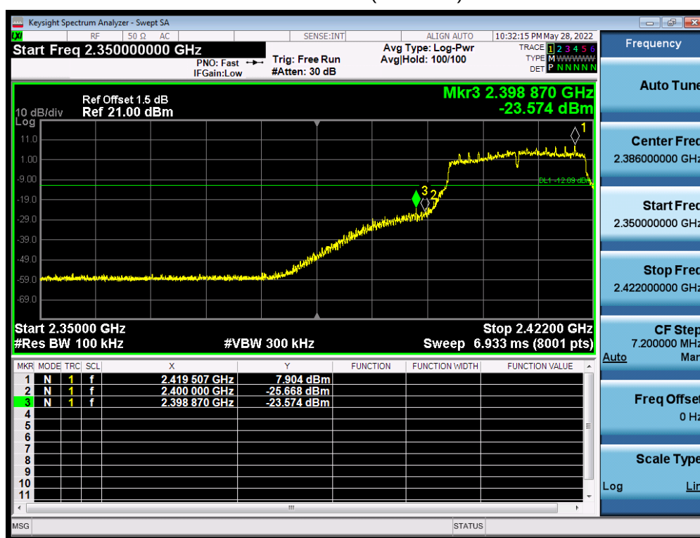
Mode 4 CH01(2412MHz)
