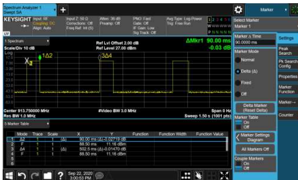
Mode 1 CH27 913.75MHz
