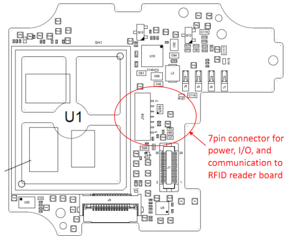
modification(Seychelles) Main PCB Assembly
