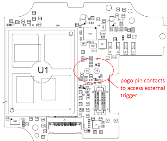
8680i (Seychelles) Main PCB Assembly
