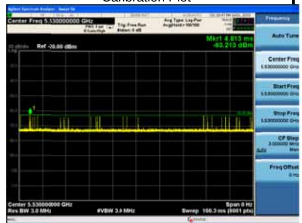
11ac80 CH106 5530MHz Radar Type 5 Calibration Plot
