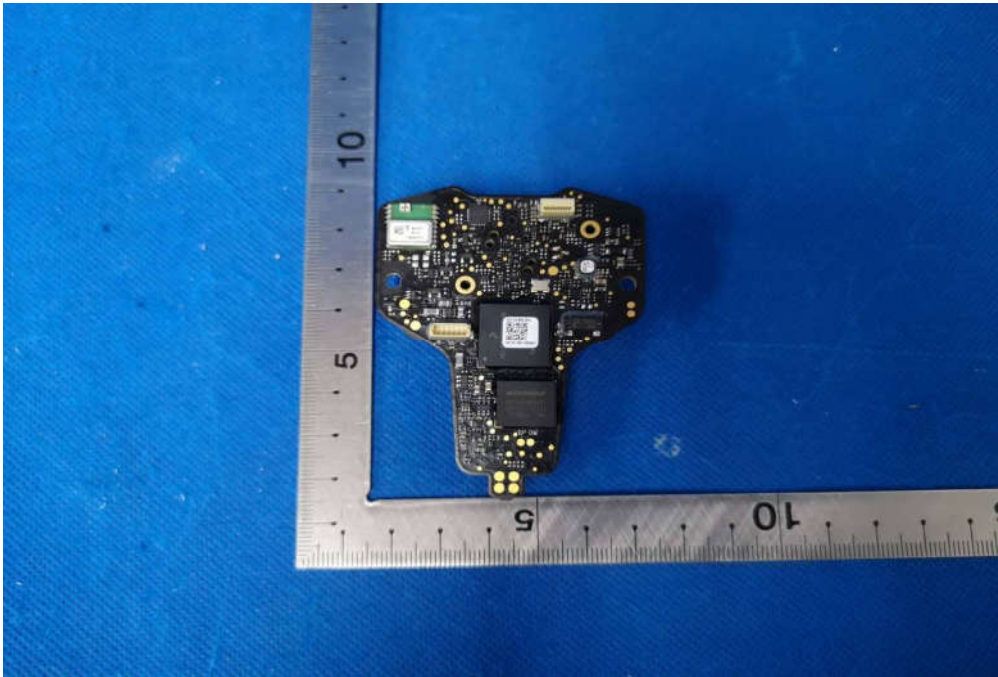
(3) EUT Photo (short distance scanner)
