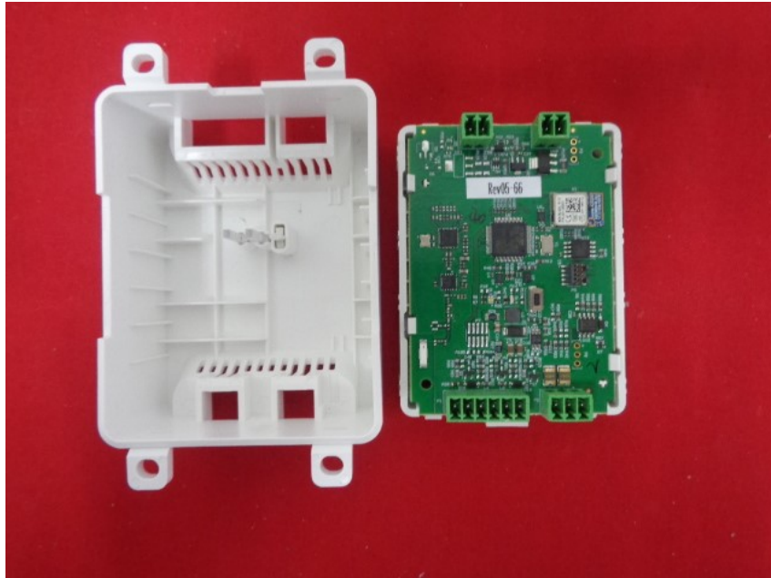
Pic 1. Internal of view
