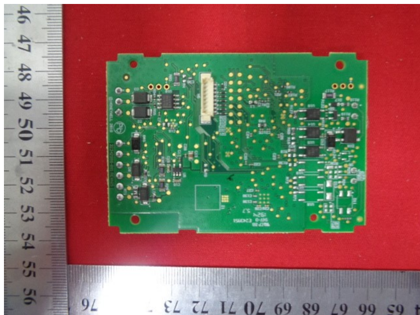
Pic 4. Back of view
