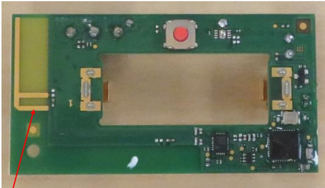
PCB BOTTOM VIEW
