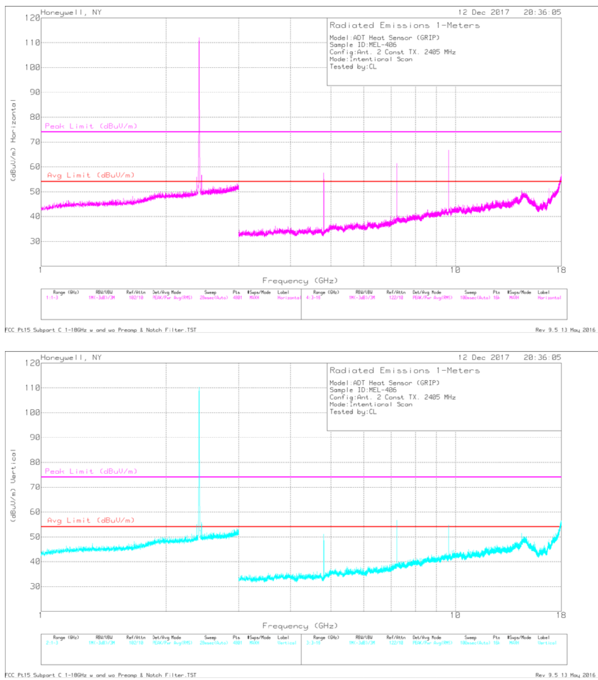
Antenna 2 Low Channel - Plot
