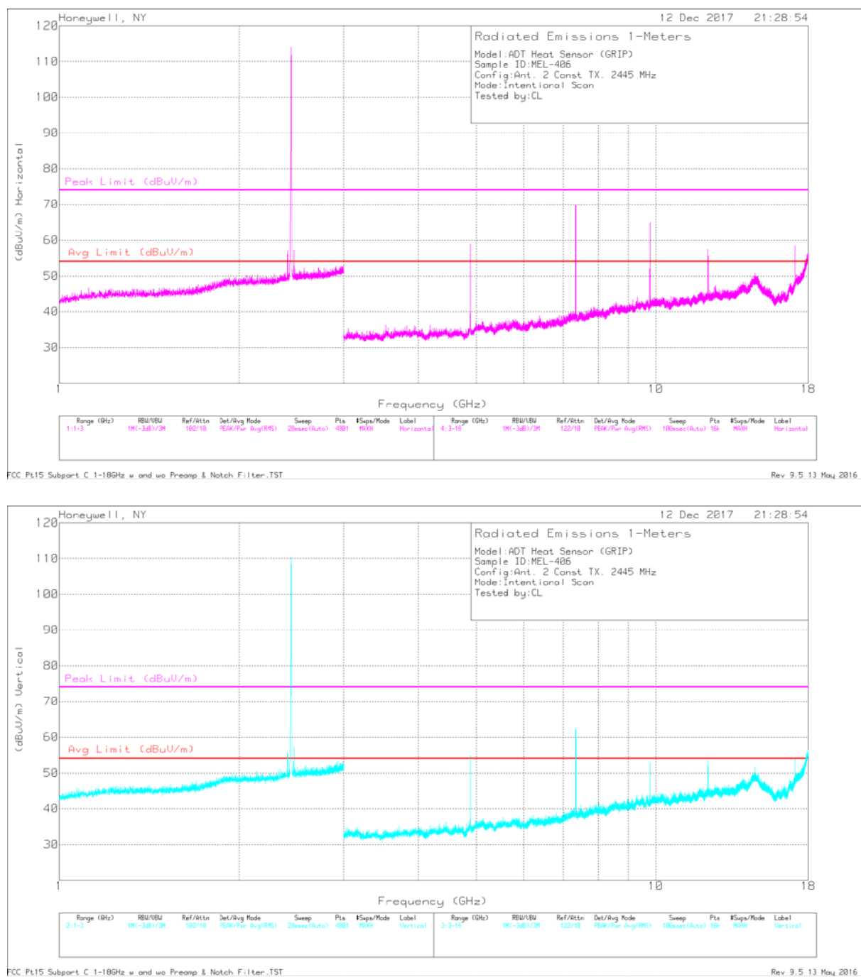
Antenna 2 Mid Channel - Plot
