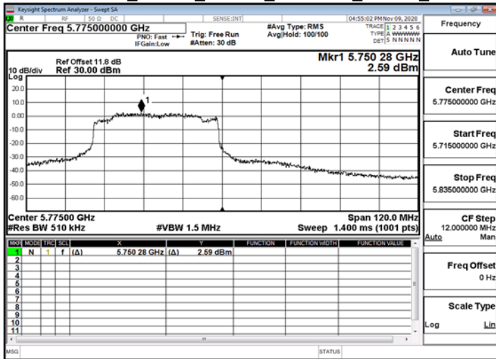
802.11ax_80MHz_ChainA_5775MHz_RU484_66
