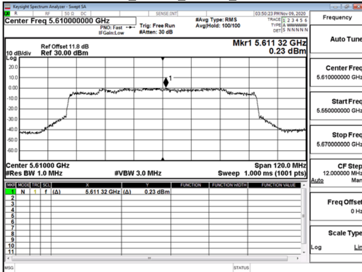
802.11ax_80MHz_ChainA_5610MHz_RU484_66
