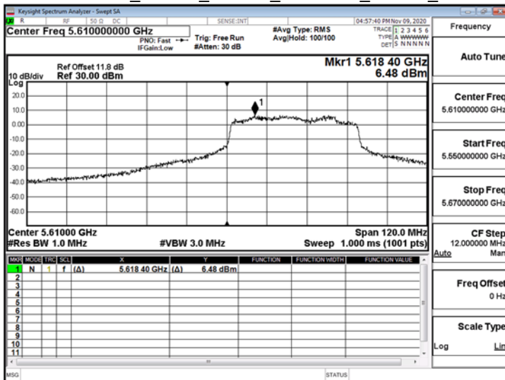
802.11ax_80MHz_ChainA_5610MHz_RU484_66
