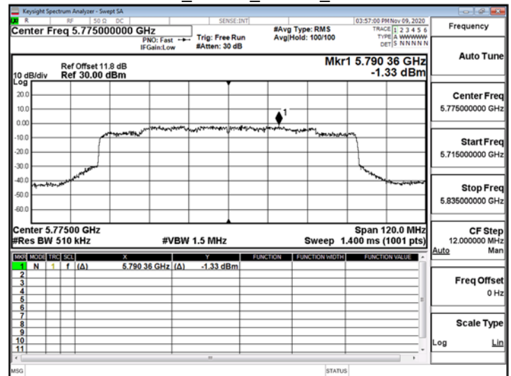
802.11ax_80MHz_ChainA_5775MHz
