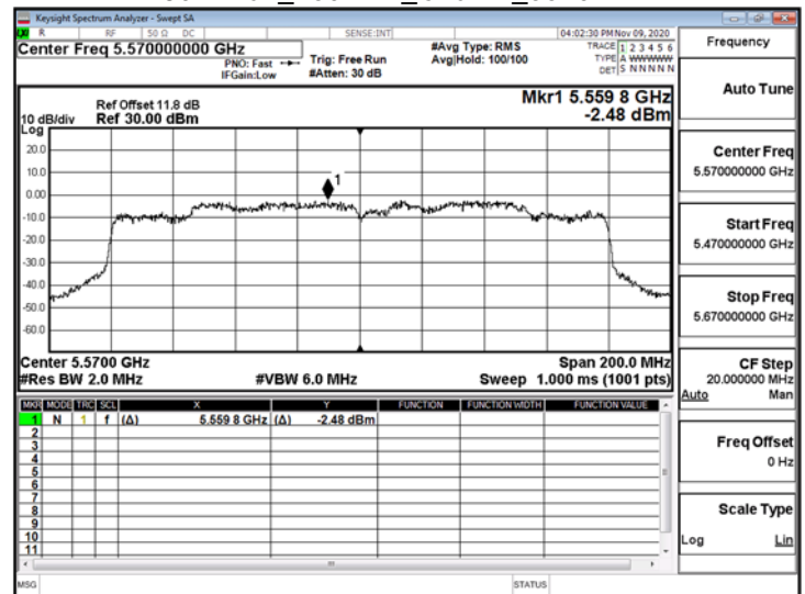
802.11ax_160MHz_ChainA_5570MHz
