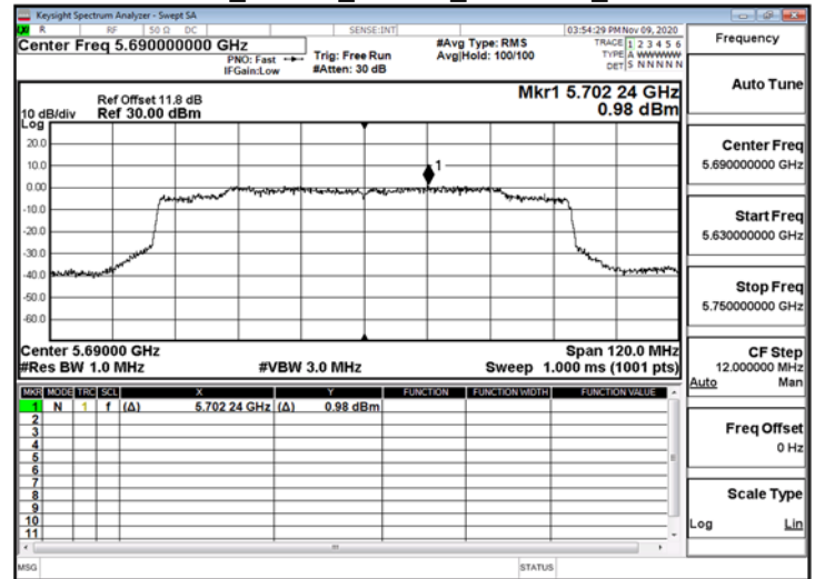
802.11ax_80MHz_ChainA_5690MHz_UNII 3
