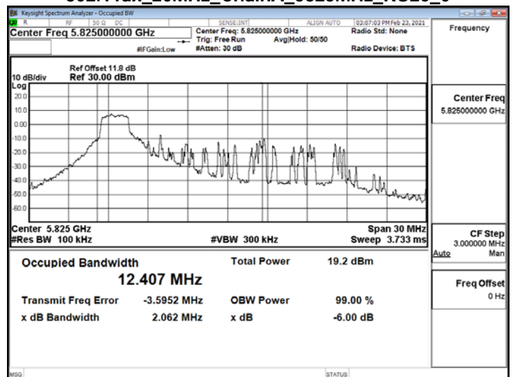
802.11ax_20MHz_ChainA_5825MHz_RU26_0
