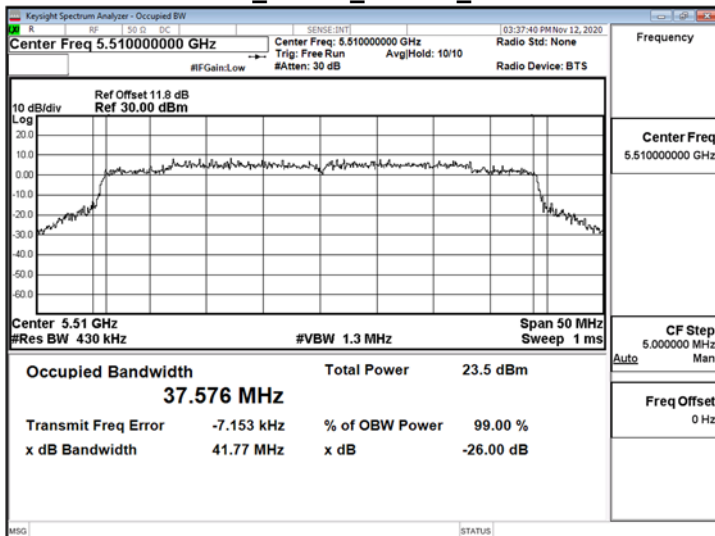
802.11ax_40MHz_ChainA_5510MHz
