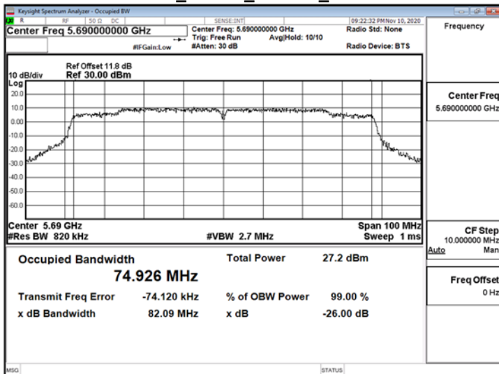
802.11ac_80MHz_ChainA_5690MHz
