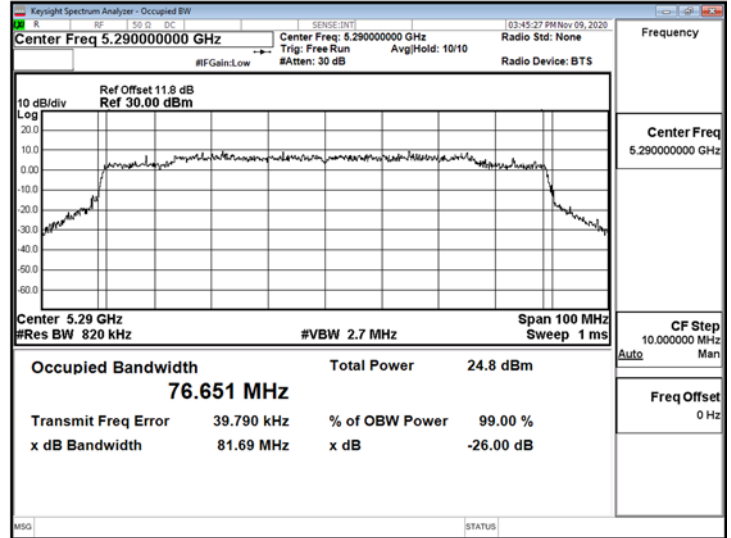
802.11ax_80MHz_ChainA_5290MHz
