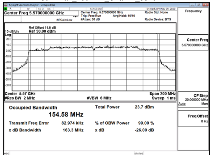
802.11ax_160MHz_ChainA_5570MHz
