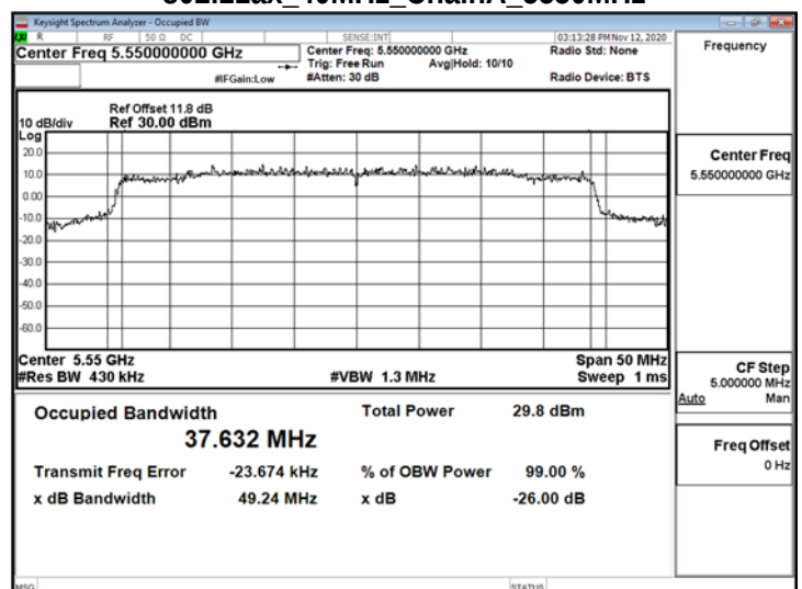
802.11ax_40MHz_ChainA_5550MHz
