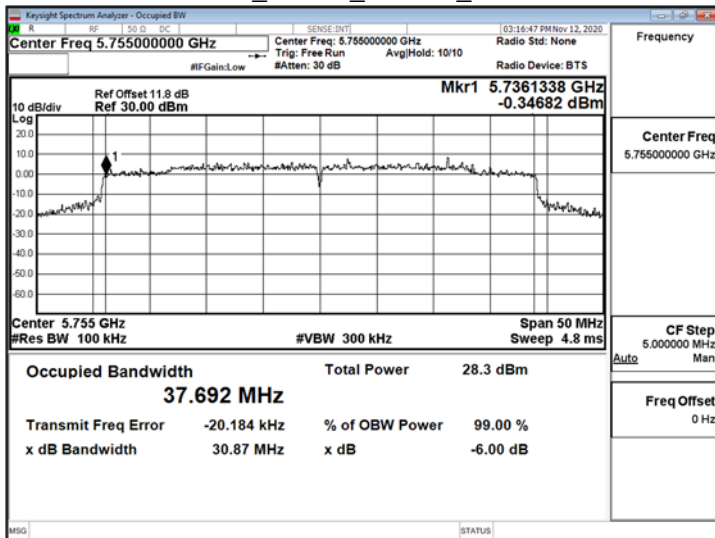
802.11ax_40MHz_ChainA_5755MHz
