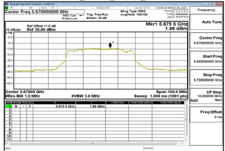
802.11ax_40MHz_ChainA_5670MHz_RU242_62
