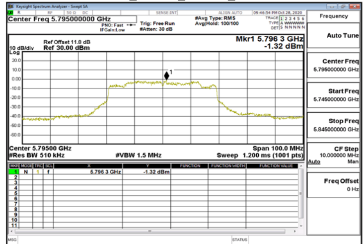
802.11ax_40MHz_ChainA_5795MHz_RU242_62
