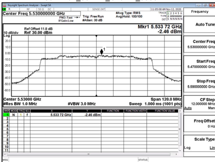
802.11ax_80MHz_ChainA_5530MHz
