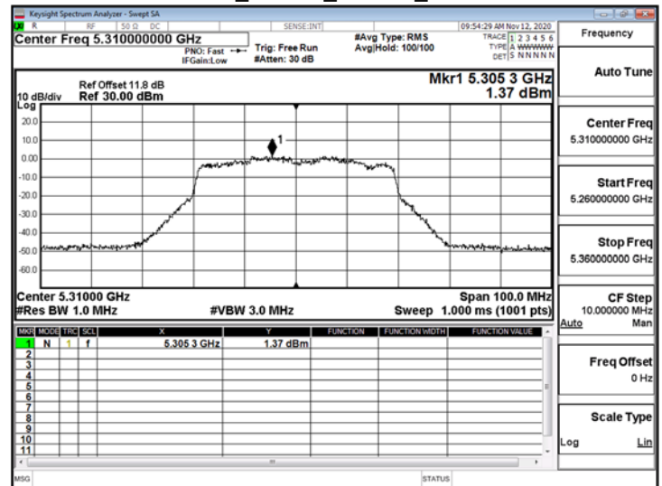
802.11ax_40MHz_ChainA_5310MHz_RU242_62
