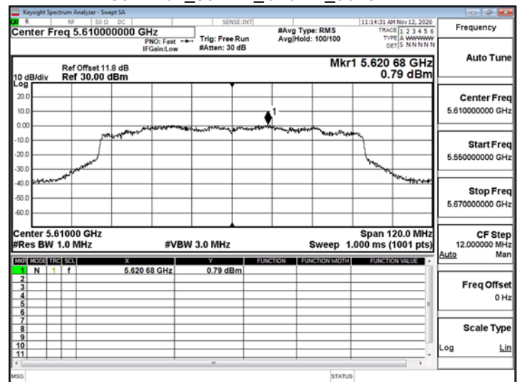
802.11ax_80MHz_ChainA_5610MHz_RU484_66
