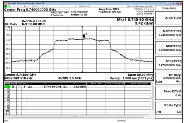
802.11ax_20MHz_ChainB_5745MHz_RU106_53
