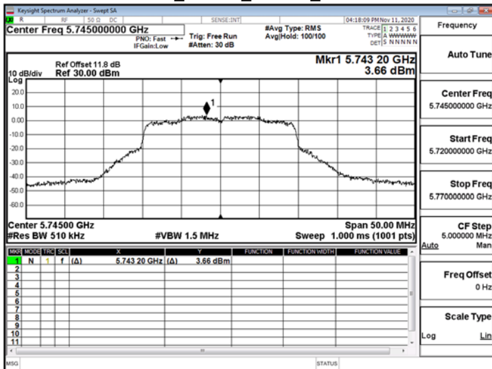
802.11ax_20MHz_ChainA_5745MHz_RU106_53
