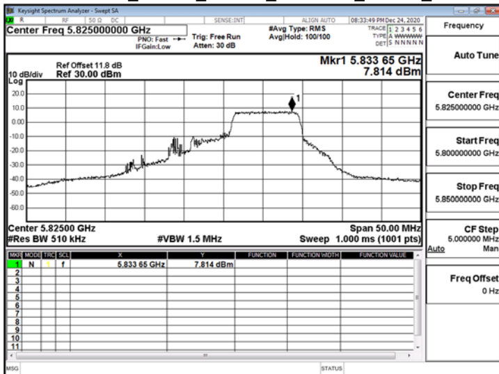
802.11ax_20MHz_ChainA_5825MHz_RU26_8
