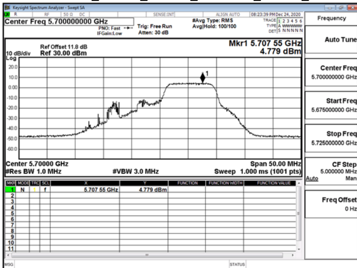
802.11ax_20MHz_ChainA_5700MHz_RU106_54
