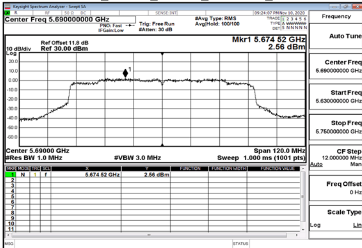
802.11ac_80MHz_ChainA_5690MHz_UNII 3
