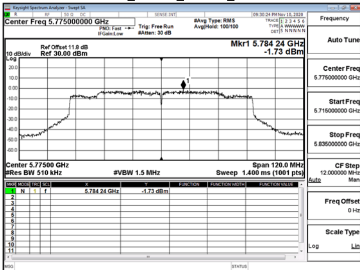
802.11ac_80MHz_ChainA_5775MHz
