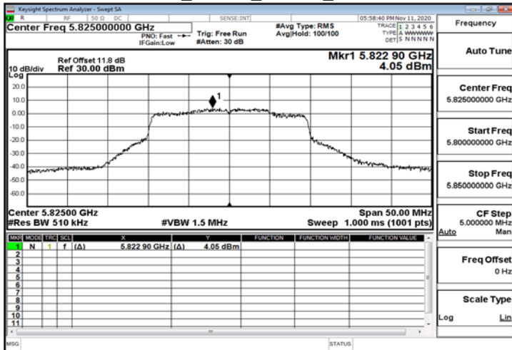
802.11ax_20MHz_ChainA_5825MHz_RU106_54
