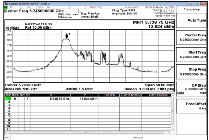
802.11ax_20MHz_ChainA_5745MHz_RU52_37
