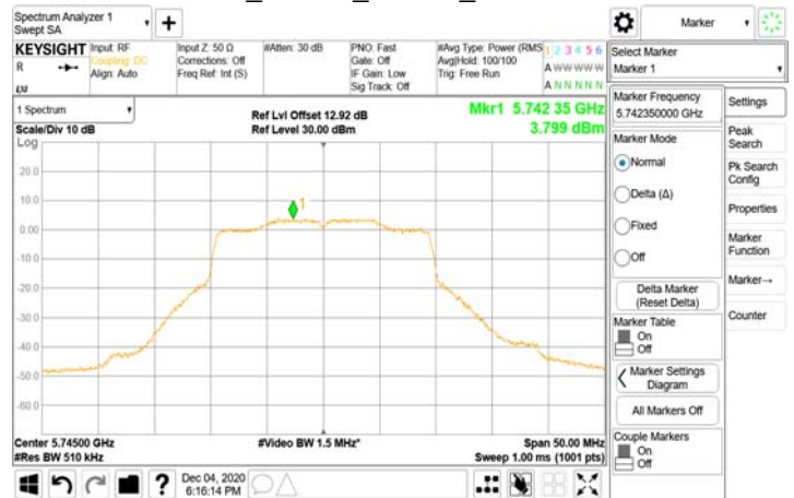
802.11ax_20MHz_Chian0_5745MHz-106-53
