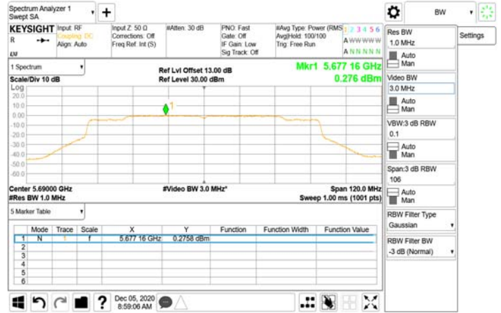
802.11ax_80MHz_Chian1_5690MHz_UNII 3
