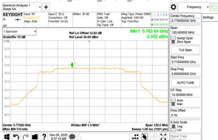
802.11ax_80MHz_Chian1_5775MHz-484-66
