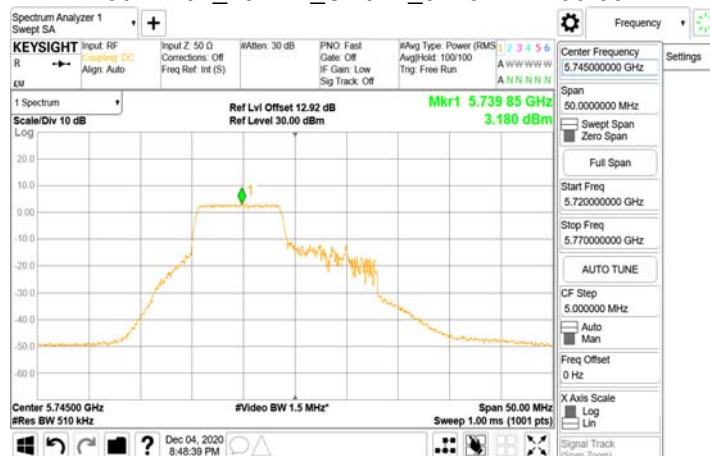
802.11ax_20MHz_Chian1_5745MHz-26-0
